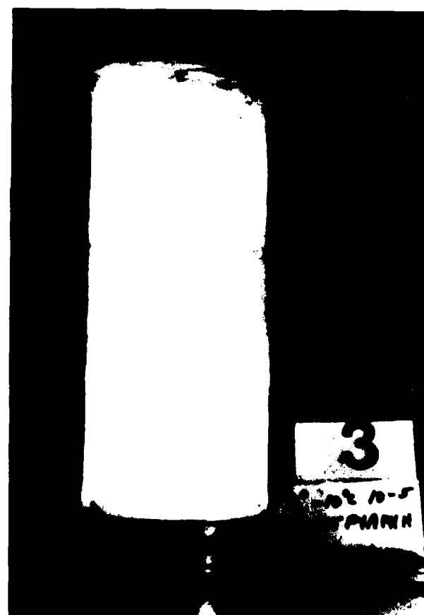
b. Deformation normal to plane of ice sheet or parallel to direction of crystal elongation.
