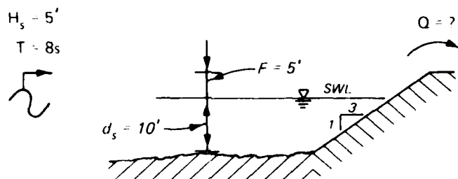
Figure 4. Definition sketch, Example 1
