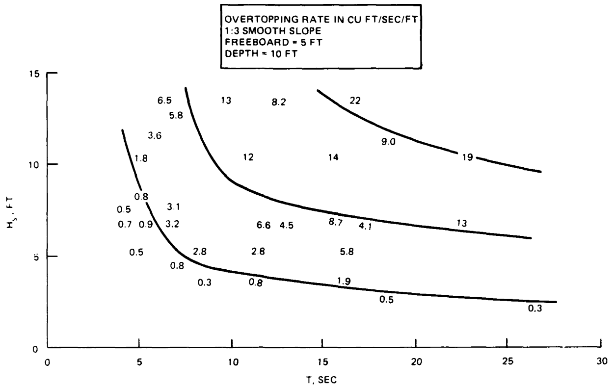
Figure 5. Dimensional overtopping rate plot, Example 2
