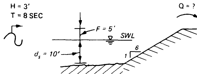
Figure 11. Definition sketch, Example 4
