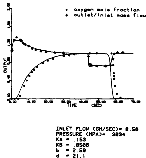
Fig. 10 3 Atmosphere breakthrough data and simulation - nonlinear coupled isotherms
