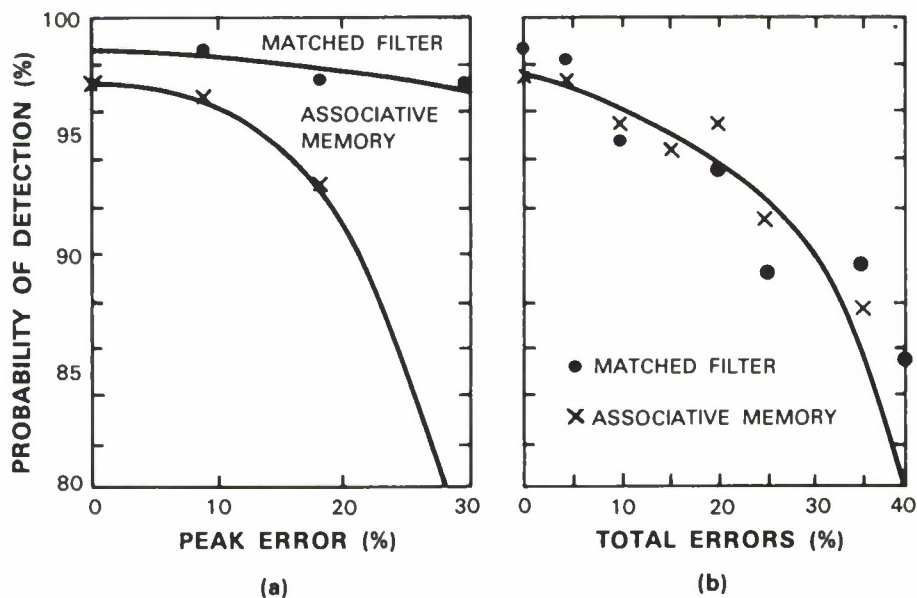
Figure 5-12. Line-detector performance for 5-by-5 images at +6-dB input SNR with (a) random additive errors in the processor coefficients, and (b) random dropouts of processor elements. The curves show averages over many processor error patterns.
