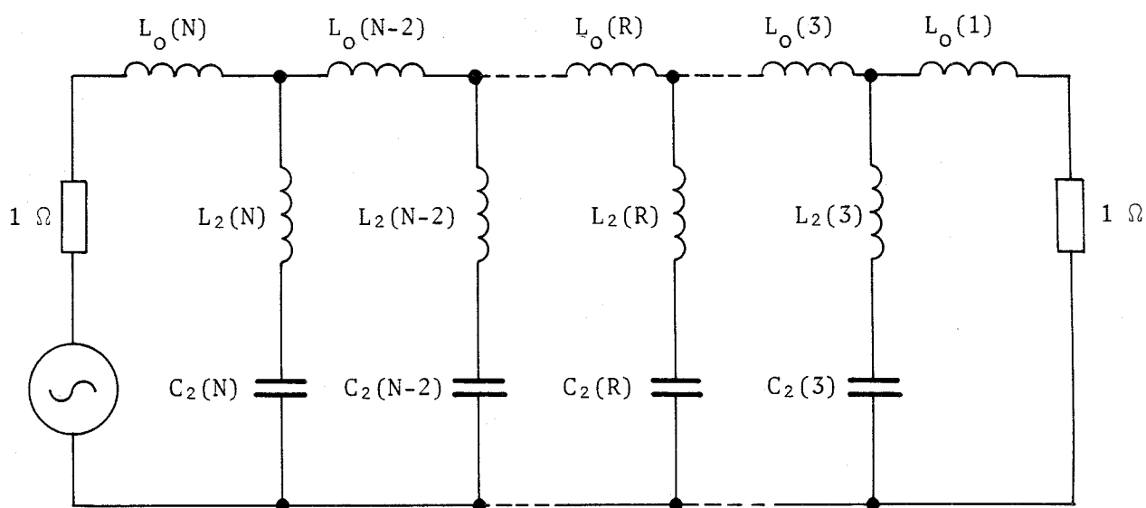
Figure 2. The generalised Chebyshev lowpass prototype filter
