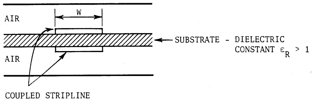
Figure 7. Inhomogeneous broadside - coupled stripline configuration
