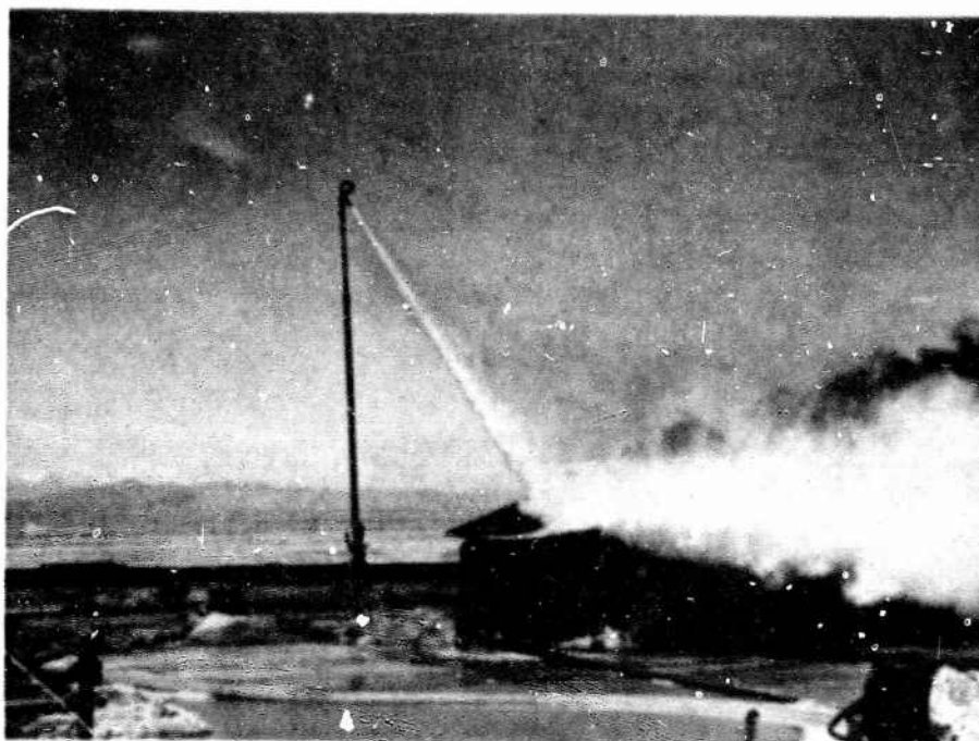
Fig. 18 - 1,000 gpm monitor mounted on a 30 ft erectable tower
