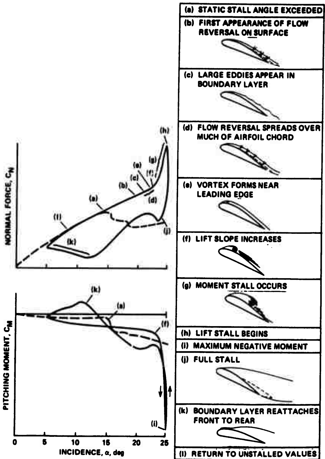
Figure 1.1 Dynamic Stall Chronology (from Carr, Ref. 1).
