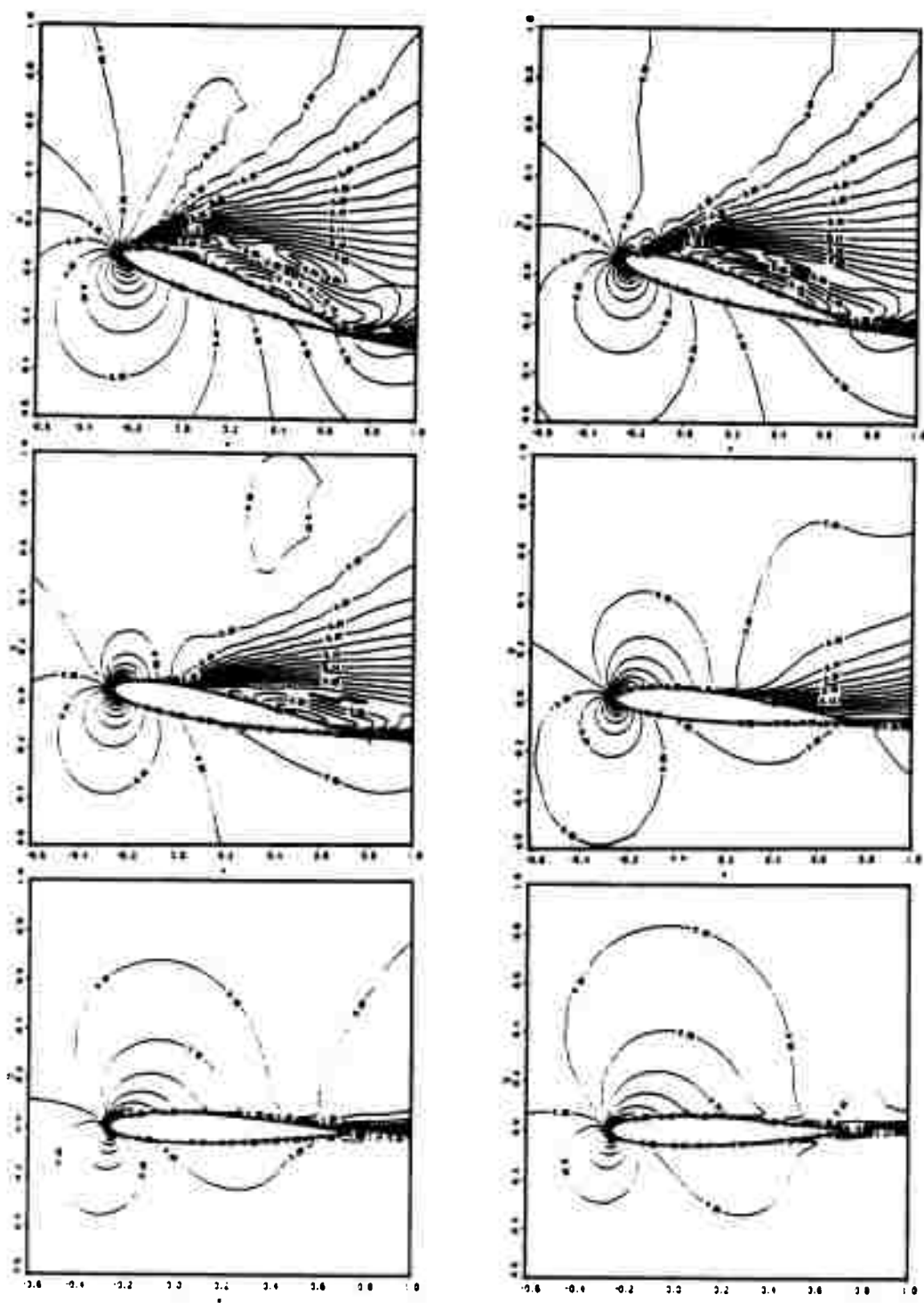
Figure 4.12 Mach Number Contour Plots, Downstroke--Baldwin-Lomax Model M_{\infty} = .283 , Re = 3.45 \times 10^6 , \alpha = 15^{\circ} - 10^{\circ} \cos(.3t) 23.67, 20.02, 15.03, 10.03, 6.36, 5 degrees.
