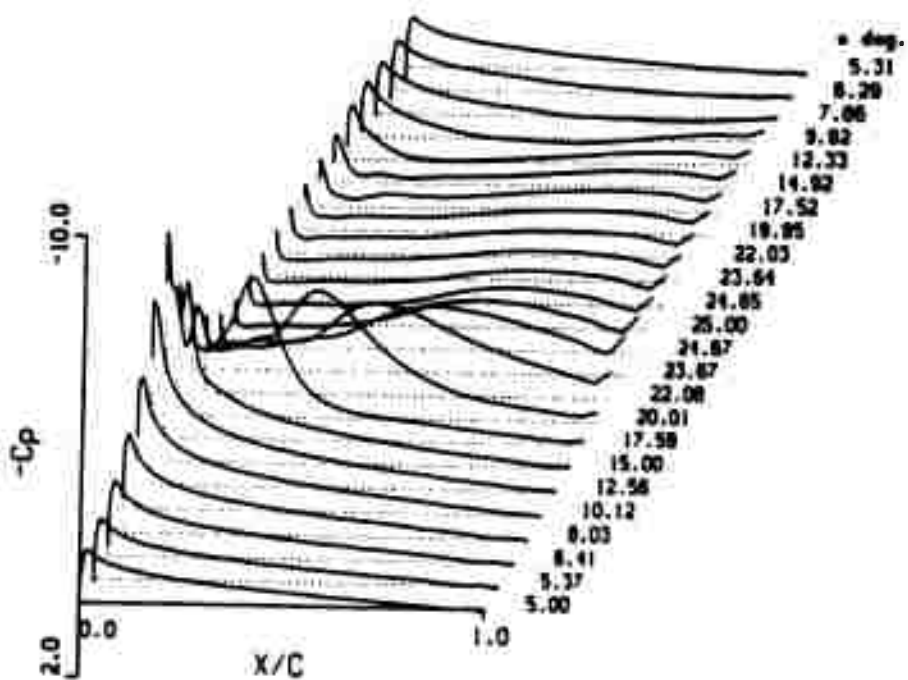
Figure 4.29 Surface Pressure Coefficient Carpet Plots--Baldwin-Lomax Model Top: M_\infty = .5 , Re = .345 \times 10^6 , \alpha = 15^\circ - 10^\circ \cos(.3t) Bottom: M_\infty = .284 (Previous Results).
