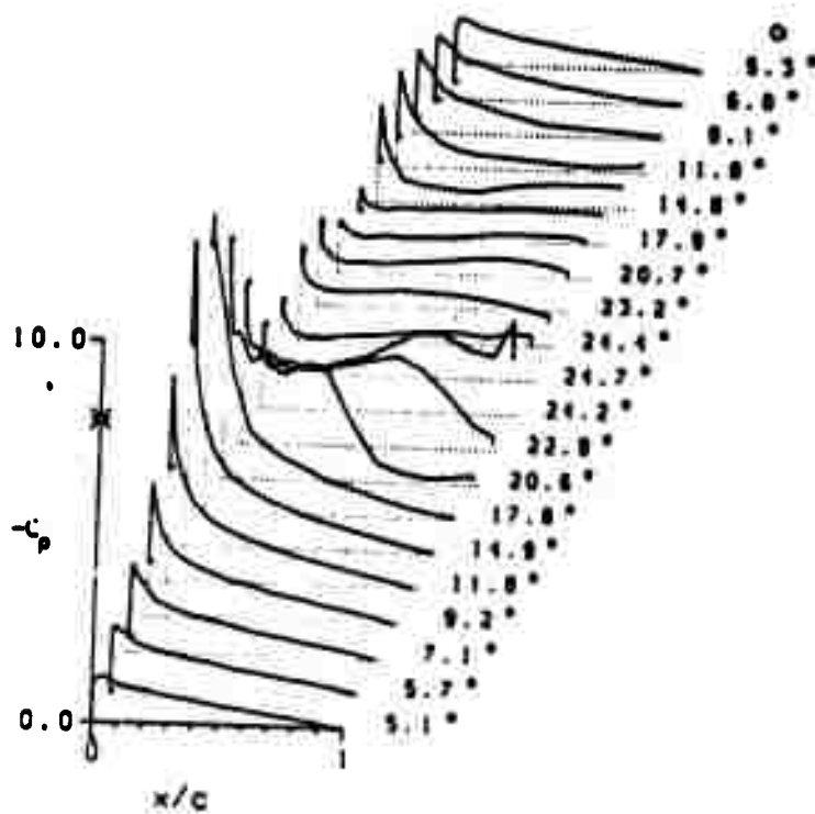
Figure 4.6 Surface Pressure Coefficient Carpet Plots--Baldwin-Lomax Model M_{\infty} = .283 , Re = 3.45 \times 10^6 , \alpha = 15^{\circ} - 10^{\circ} \cos(.3t) , Top--theoretical, Bottom--experimental (Ref. 8).
