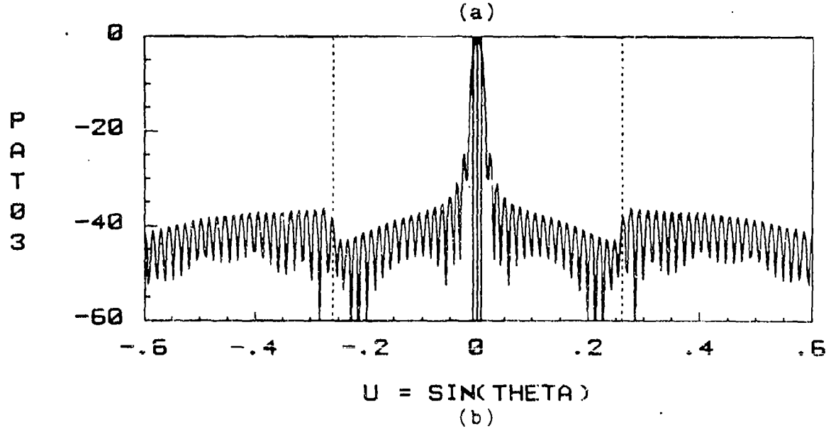
Fig 28. One Failure Near End: a) Optimum Distribution; b) Far Field Pattern
