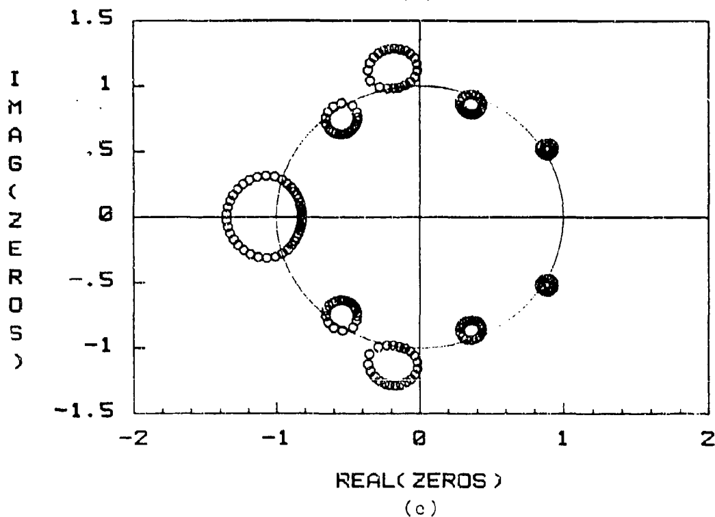
Fig 23 cont. Zero Travel Due to Phase Perturbations of Selected Elements of an 11 Element Array: b) Single (-1); c) Single (1)
