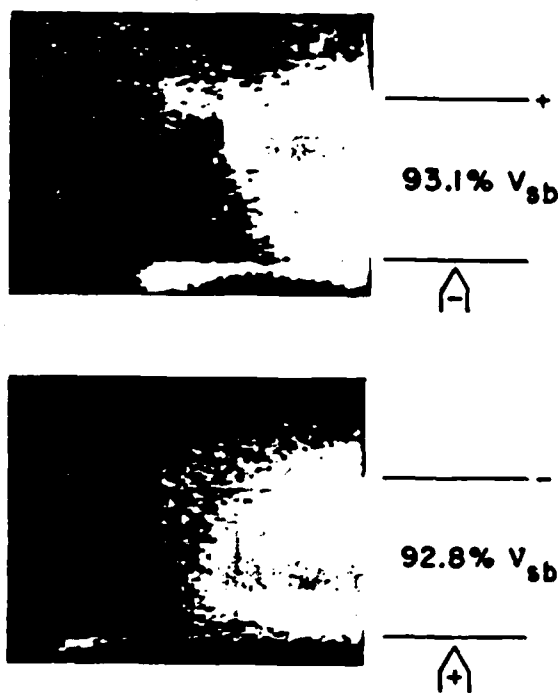
Figure 2. Streak photographs of the initial stages of breakdown in the two hetero-polar configurations. Positions of the electrodes are indicated in the drawings at the right.
