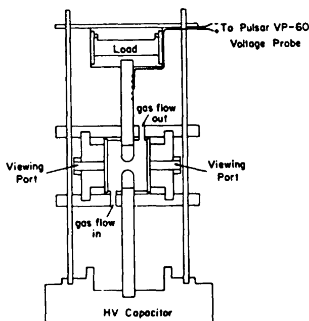
Fig. 1 Experimental Arrangement
