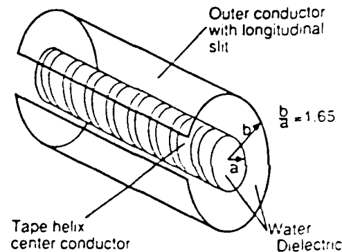
Fig. 1. Helical line pulser.
