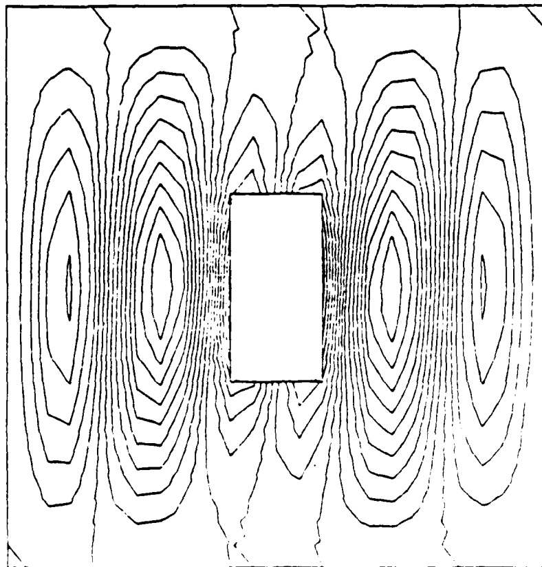
Figure 40 0° Panel--Mode 4
