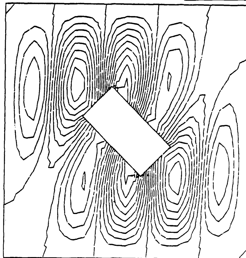
Figure 58 +45° Panel Mode 5
