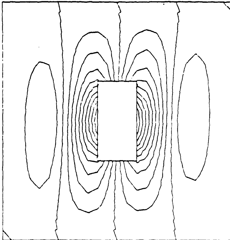
Figure 37 0° Panel--Mode 1
