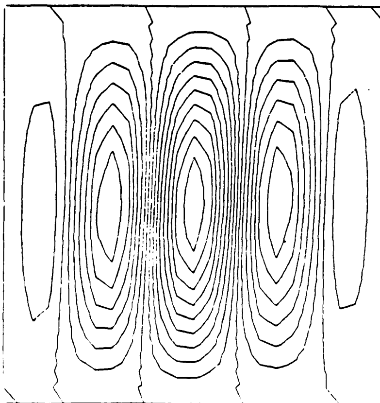
Figure 30 Solid Panel--Mode 2
