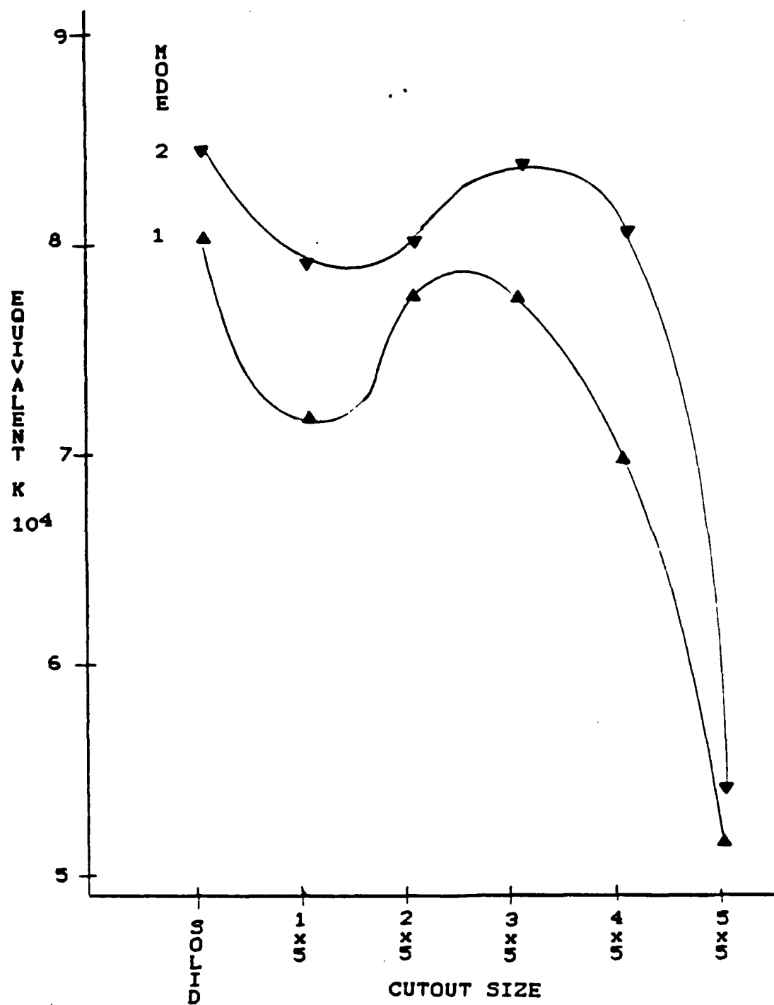
Figure 68 Equivalent Stiffness vs Cutout Size
