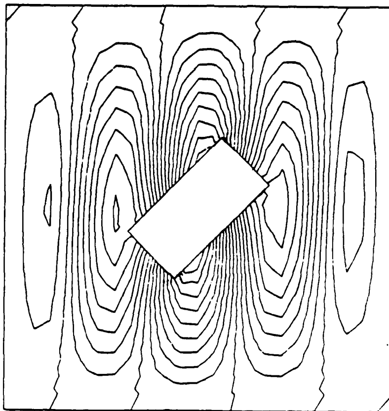
Figure 81 -45° Panel Mode 2
