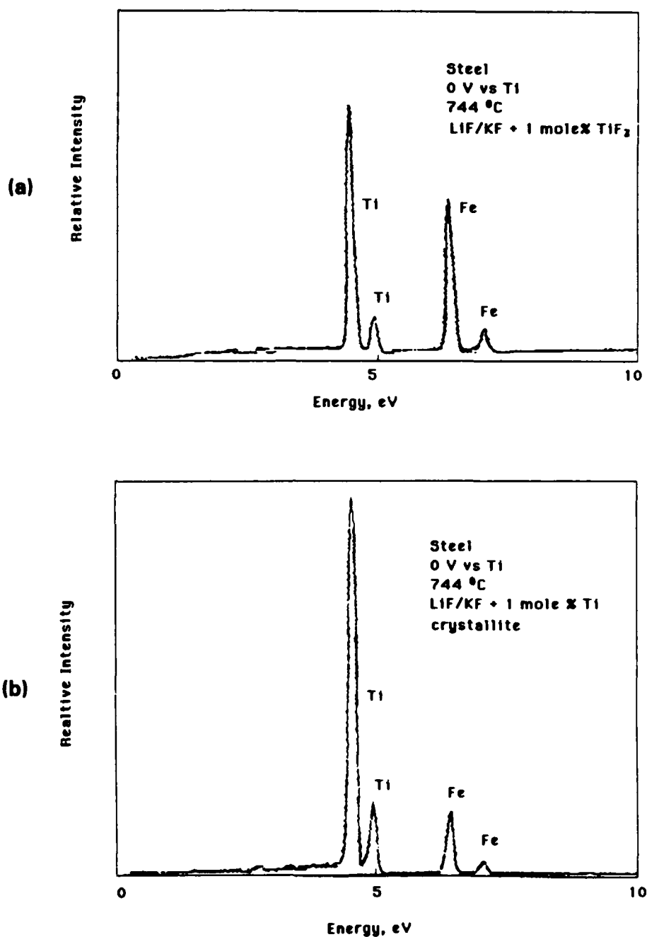
Fig. 17 EDAX for steel surface subjected to electrolysis at 0 V vs \text{Ti/Ti}^{3+} electrode ( 10 \text{ mA/cm}^2 ) in Ti containing LiF/KF molten salt at 744^\circ\text{C} (a); crystallite formed under the same conditions (b).
