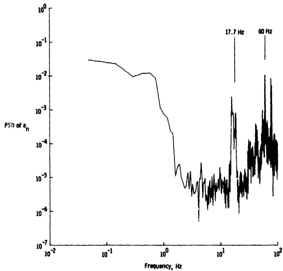
Figure 7.3-3. Power spectral density of 200-sample/sec normal acceleration.
