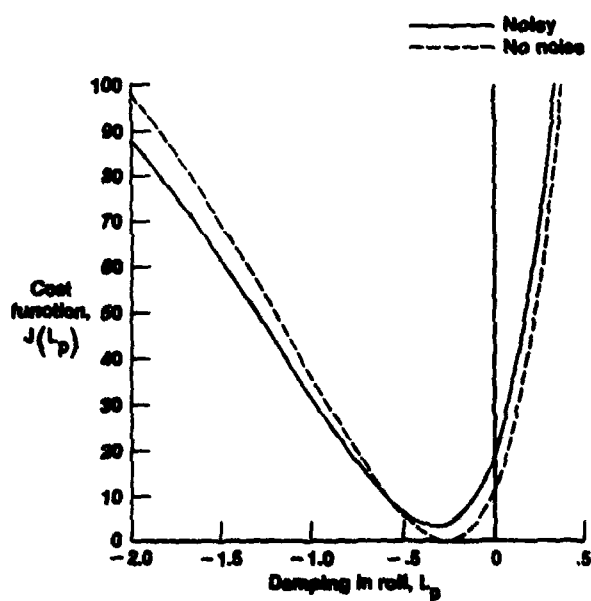
Figure 4.4-4. Comparison of the cost functions for the no-noise and noisy cases.
