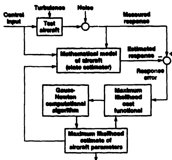
Figure 4.1-1. Maximum likelihood estimation concept.
