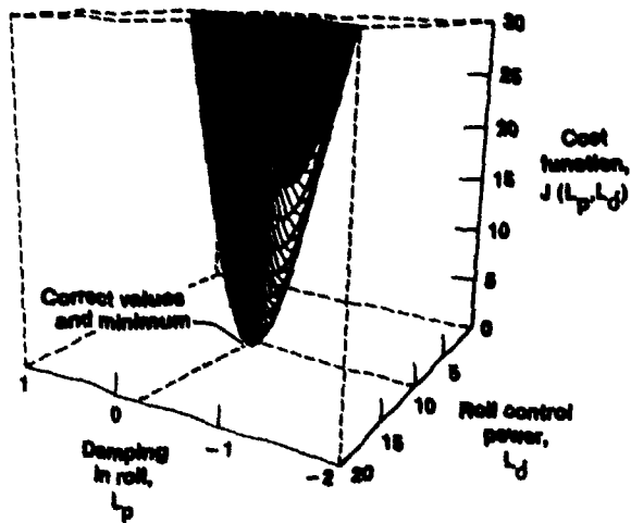
Figure 4.4-12. Detailed view of cost function surface for no-noise case.
