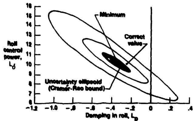
Figure 4.4-16. Isocontrol lines and uncertainty ellipse of the cost function for the noisy case.
