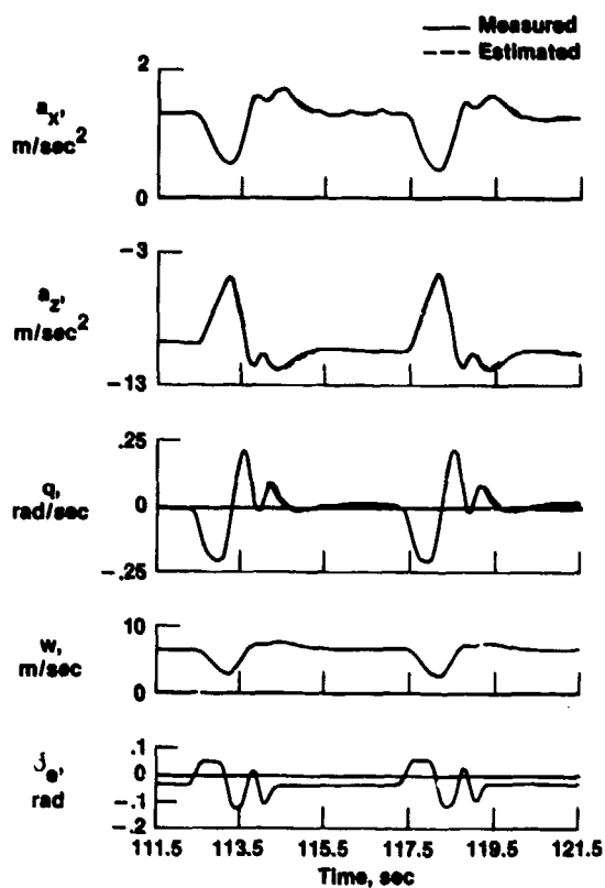
Figure 6.3-3. A 3211 input (Plaetschke and Schulte, 1979).
