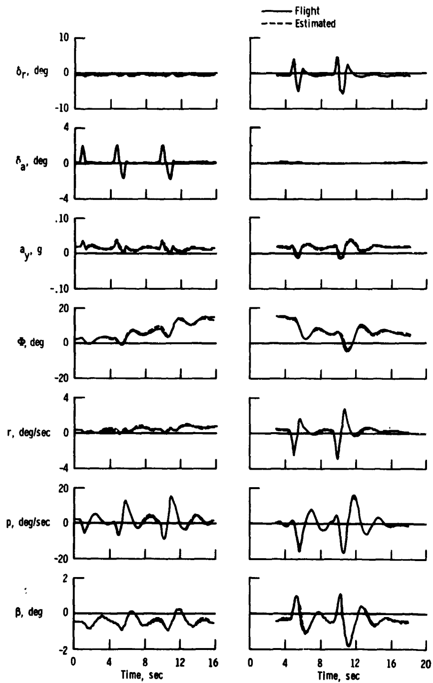
Figure 6.4-15. Lateral-directional double maneuver of an F-111A aircraft.
