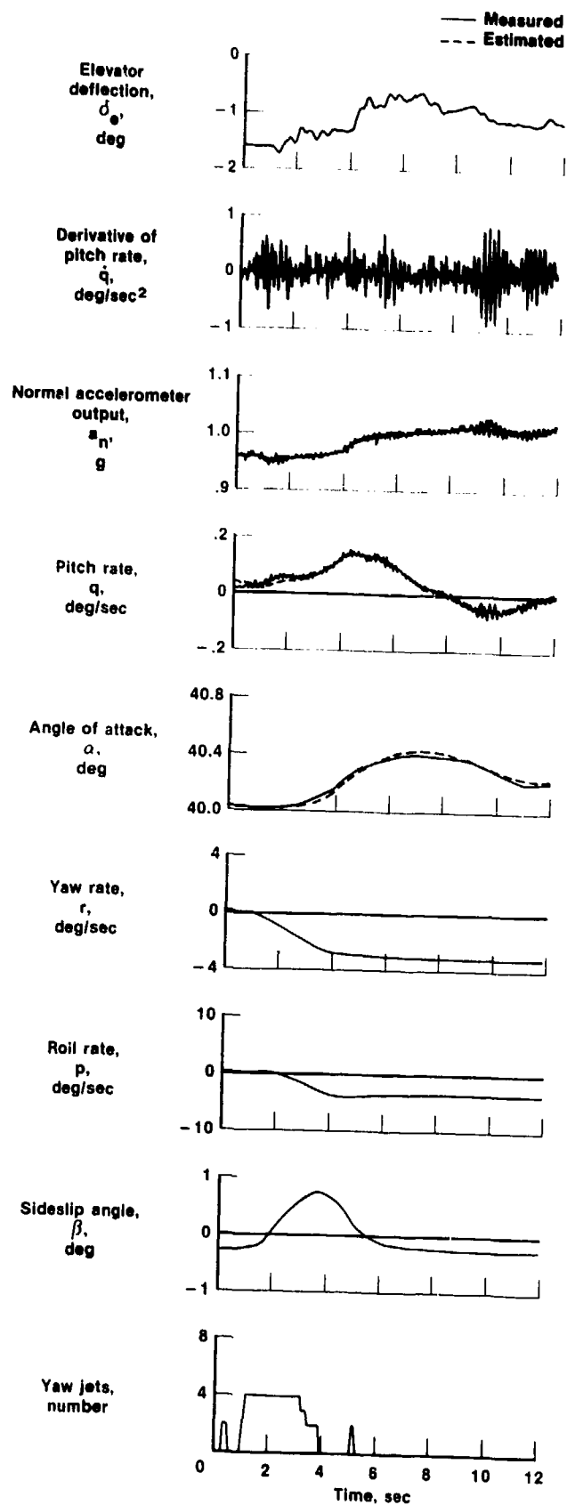
Figure 5.2-4. Fit of small longitudinal maneuver with gyroscopic effects.
