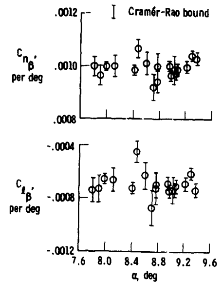
Figure 9.1-5. Estimates from simulated data with white noise.
