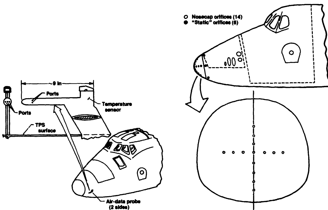
Figure 8.5-2. Shuttle side probes.
