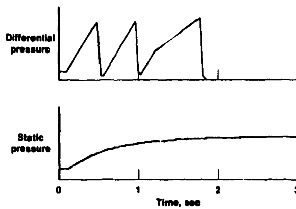
Figure 8.7-2. Step response test of pressure sensor.
