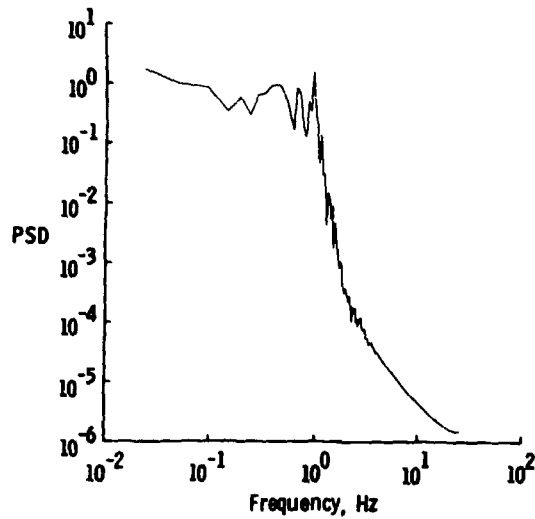
Figure 9.1-8. Spectrum of simulated colored noise.
