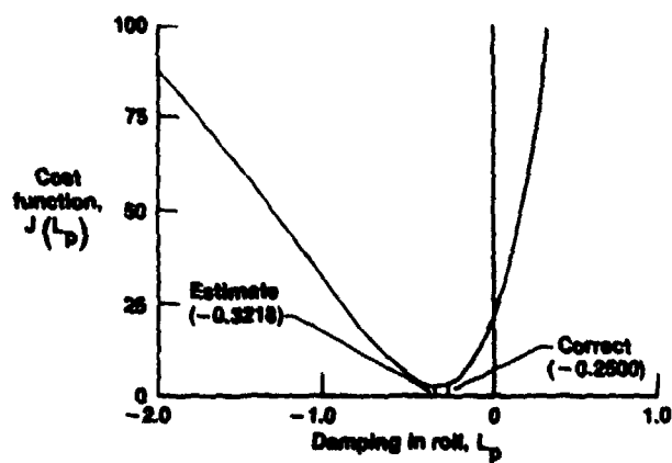
Figure 4.4-3. Cost function as a function of L_p for noisy case.
