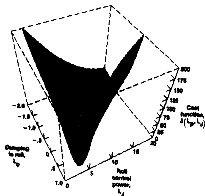
Figure 4.4-10. Restricted view of cost function surface.
