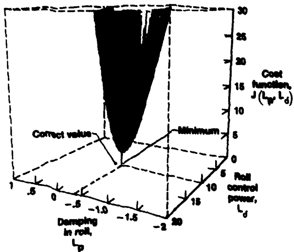
Figure 4.4-14. Detailed view of cost function surface for noisy case.
