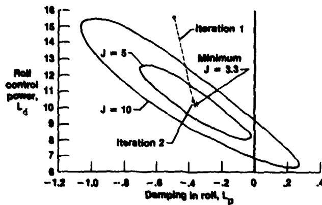
Figure 4.4-15. Isolines of constant cost for region near minimum for noisy case.
