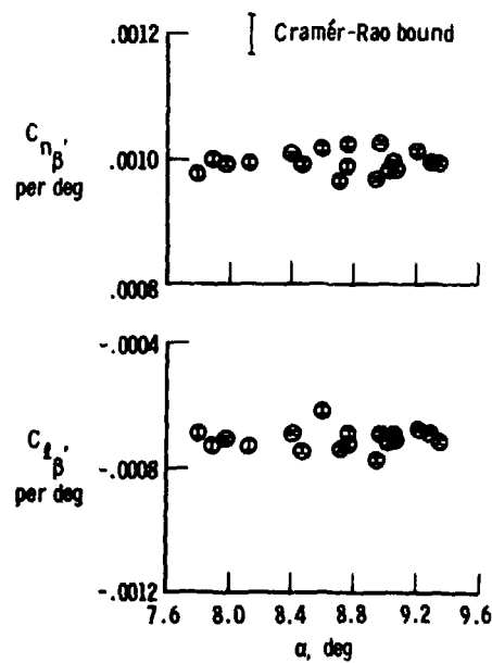
Figure 9.1-10. Estimates from simulated data with colored noise.
