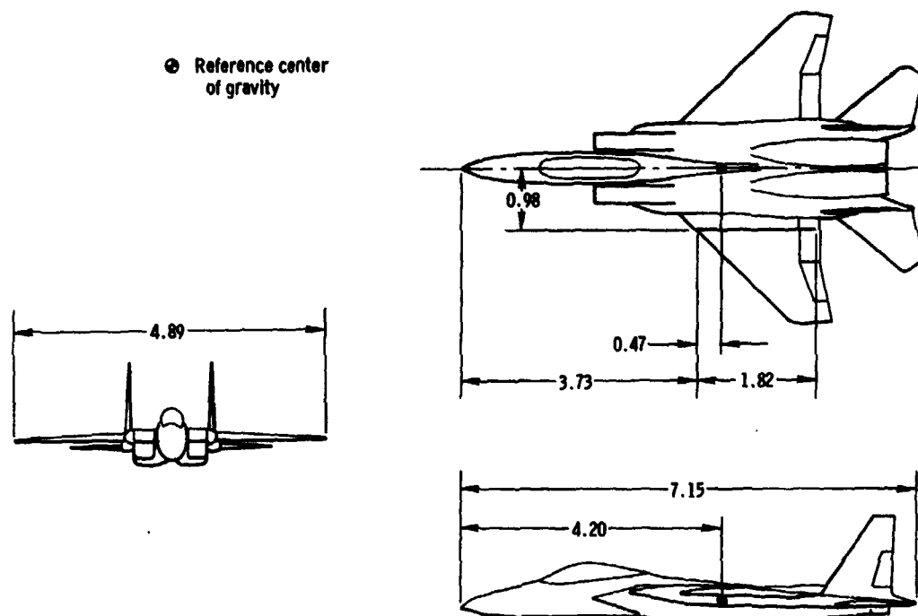
Figure 9.2-3. The 3/8-scale F-15 model (dimensions in meters).
