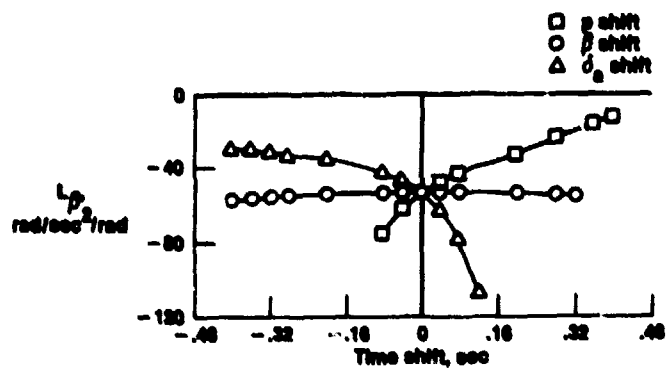
Figure 7.3-2. Effects of time shifts.
