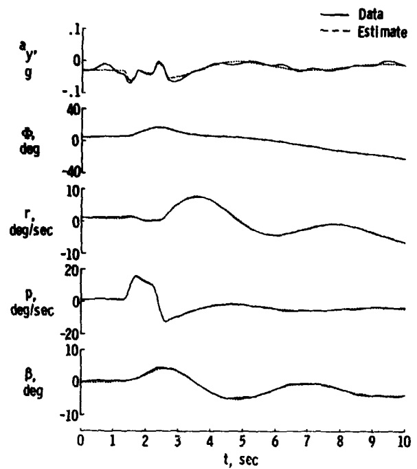
Figure 9.1-9. Time history of simulated data with colored noise.
