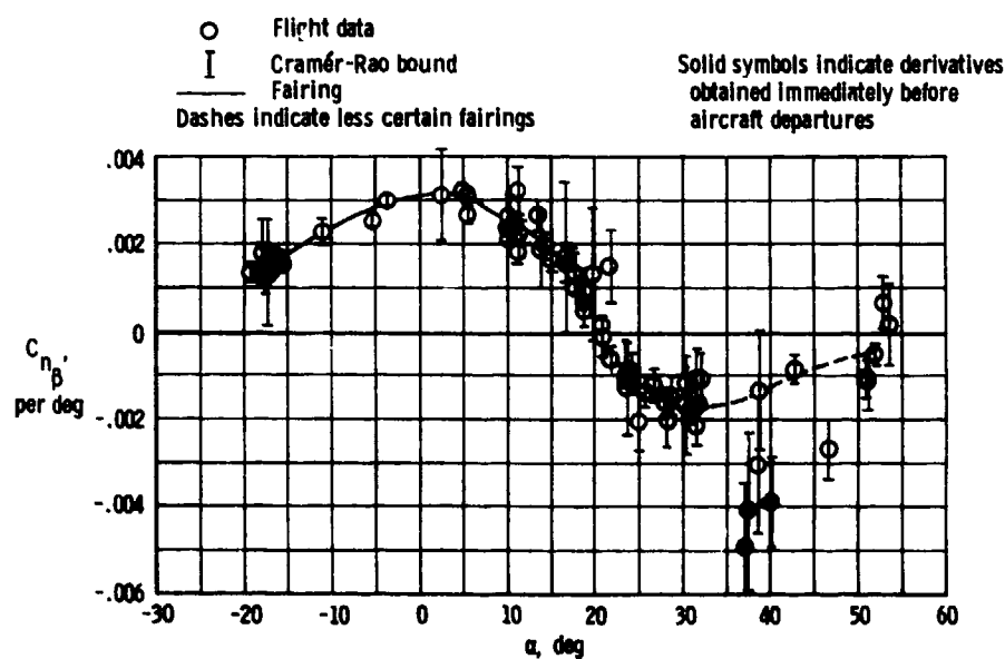
Figure 9.2-6. Estimates of C_{n_\beta} for 3/8-scale F-15 model.
