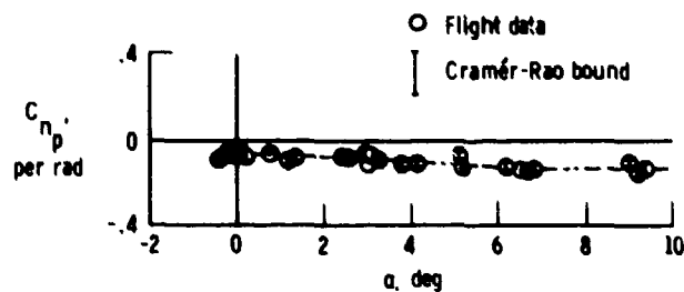
Figure 6.4-11. Estimates of C_{np} from multiple-maneuver analysis.
