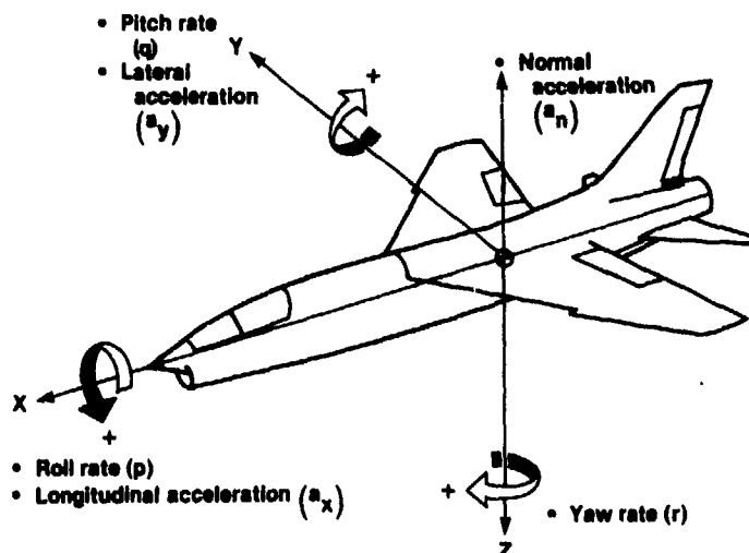
Figure 2.1-2. Body-axis system.
