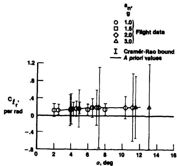
Figure 9.2-11. Estimates of C_{l_r} for F-111A airplane.
