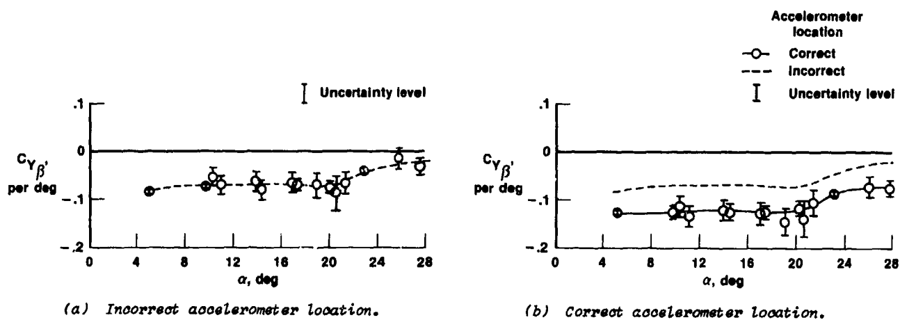
Figure 5.2-3. C_{Y\beta} estimates with incorrect and correct sensor positions.
