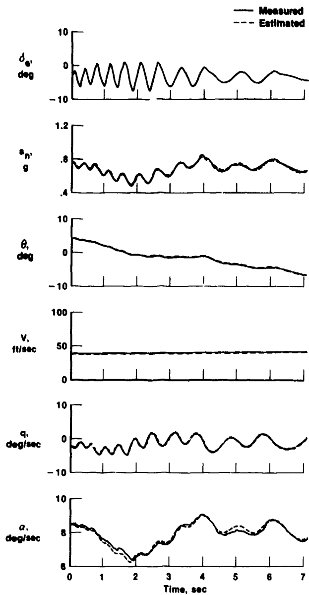
Figure 6.3-2. Frequency-sweep input.
