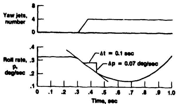
Figure 4.5-3. Examples of obtaining L_{y_j} by simple calculations for the shuttle data from Figure 4.5-2.
