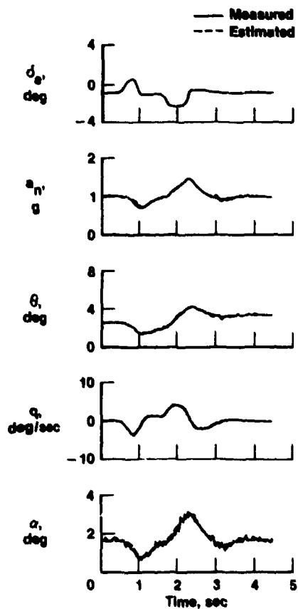
Figure 6.4-3. Longitudinal maneuver of a Beech-99 aircraft.
