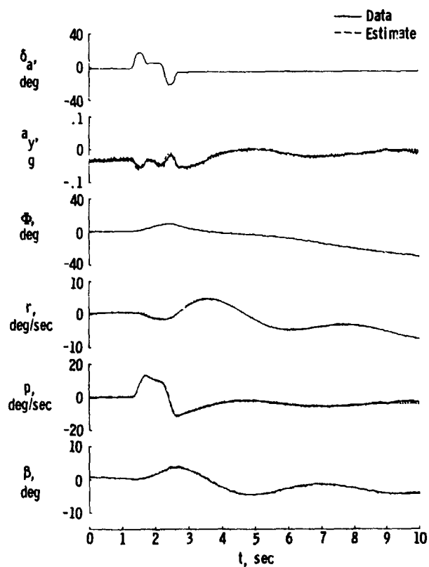
Figure 9.1-2. Time history of PA-30 flight maneuver.
