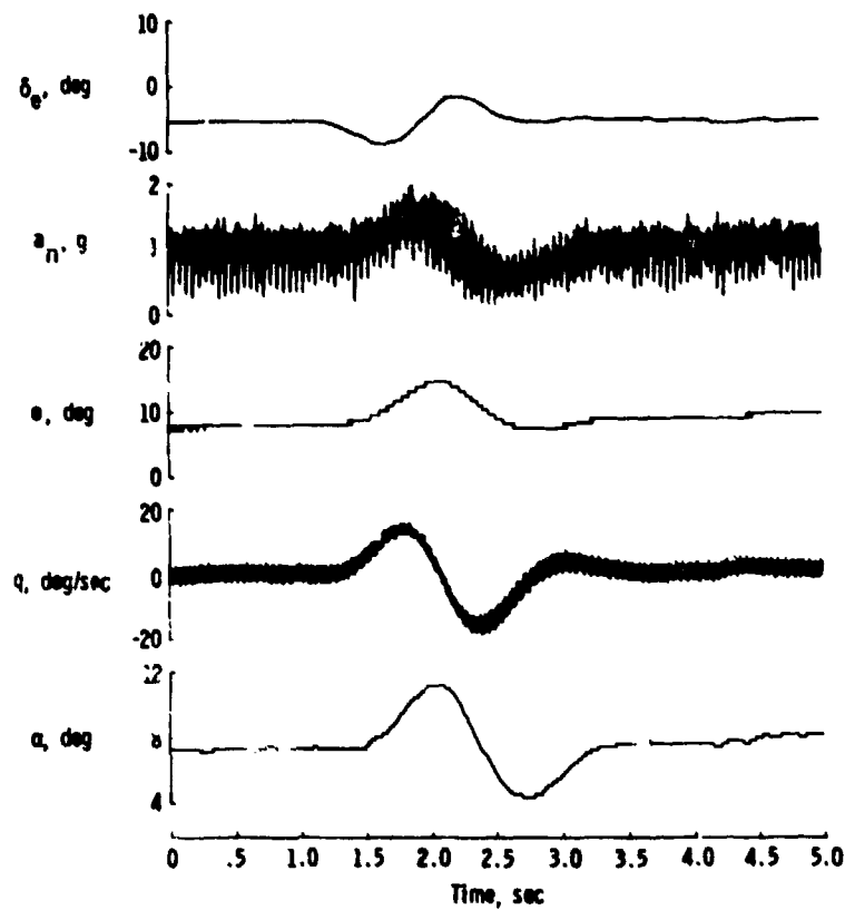
Figure 7.3-3. Oblique-wing 200-sample/sec data.
