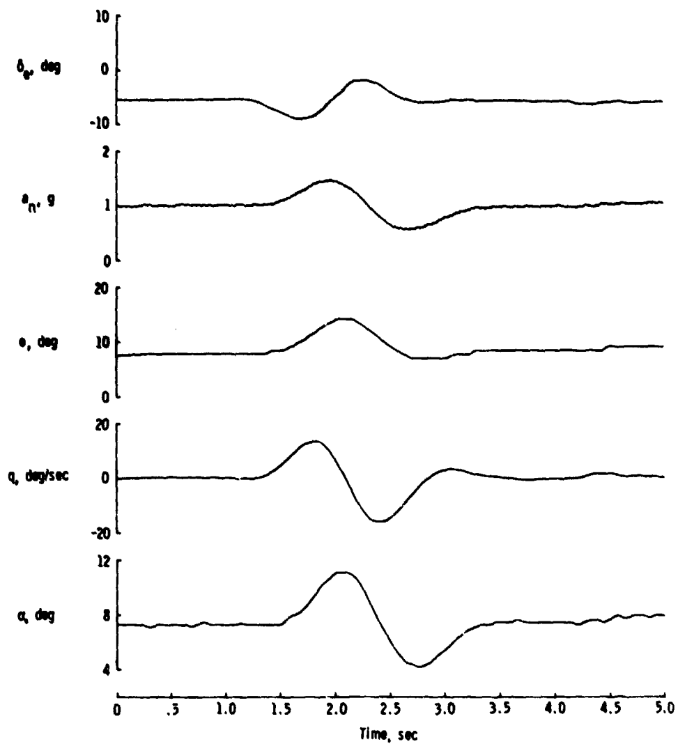
Figure 7.3-6. Time history of filtered data.
