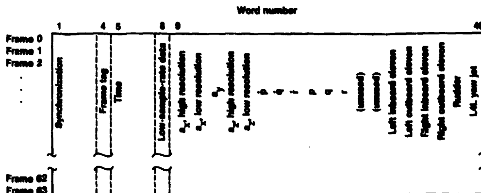
Figure 7.2-1. ACIP PCM system layout.
