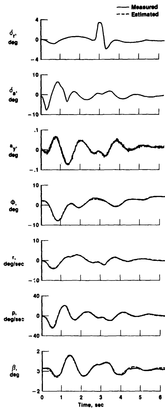
Figure 6.4-14. Lateral-directional maneuver of an HL-10 lifting body.
