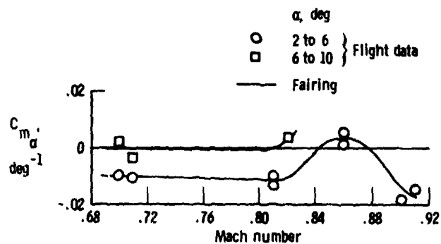
Figure 9.2-9. Estimates of C_{m_\alpha} as a function of Mach number for F-111A airplane.
