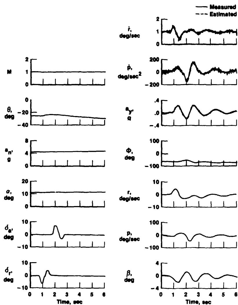
Figure 6.2-5. Maneuver at Mach 0.9, \alpha = 12^\circ .
