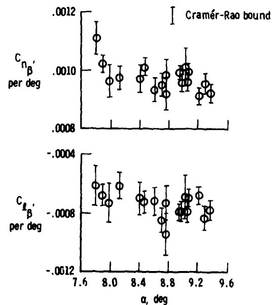
Figure 9.1-11. Estimates from flight data corrected using filter and empirical factor.
