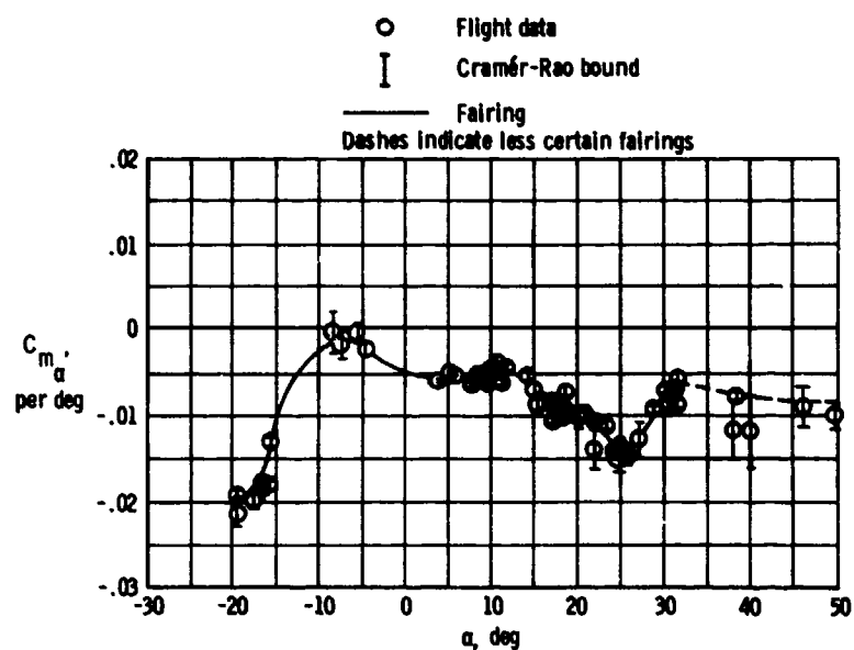
Figure 9.2-5. Estimates of C_{m_\alpha} for 3/8-scale F-15 model.
