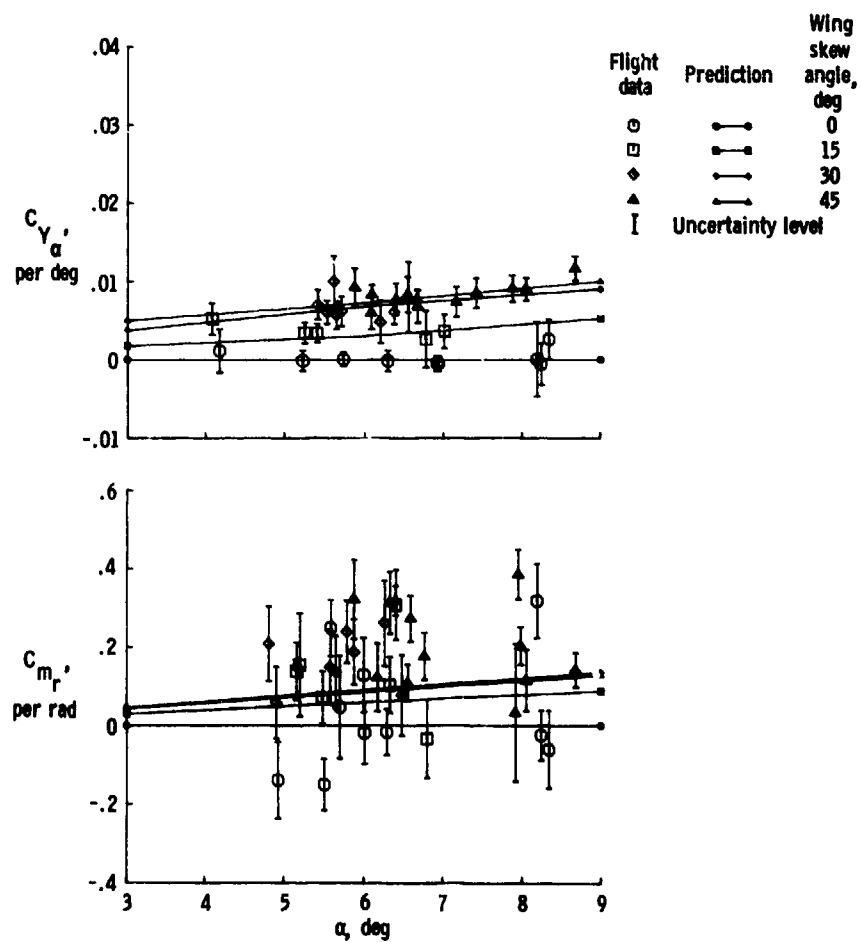
Figure 9.2-2. Estimates of C_{Y_{\alpha}} and C_{m_r} for oblique-wing aircraft.
