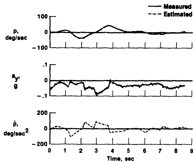
Figure 5.2-2. Time history match with correct sensor position.
