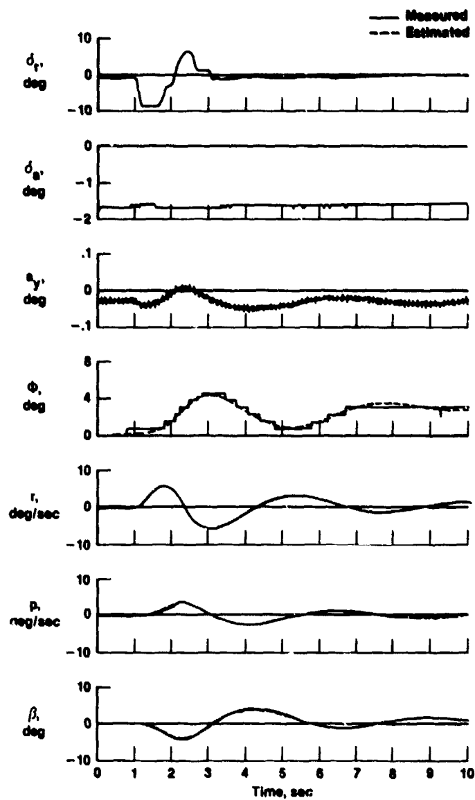
Figure 6.4-7. Rudder maneuver on a Piper PA-30 aircraft.
