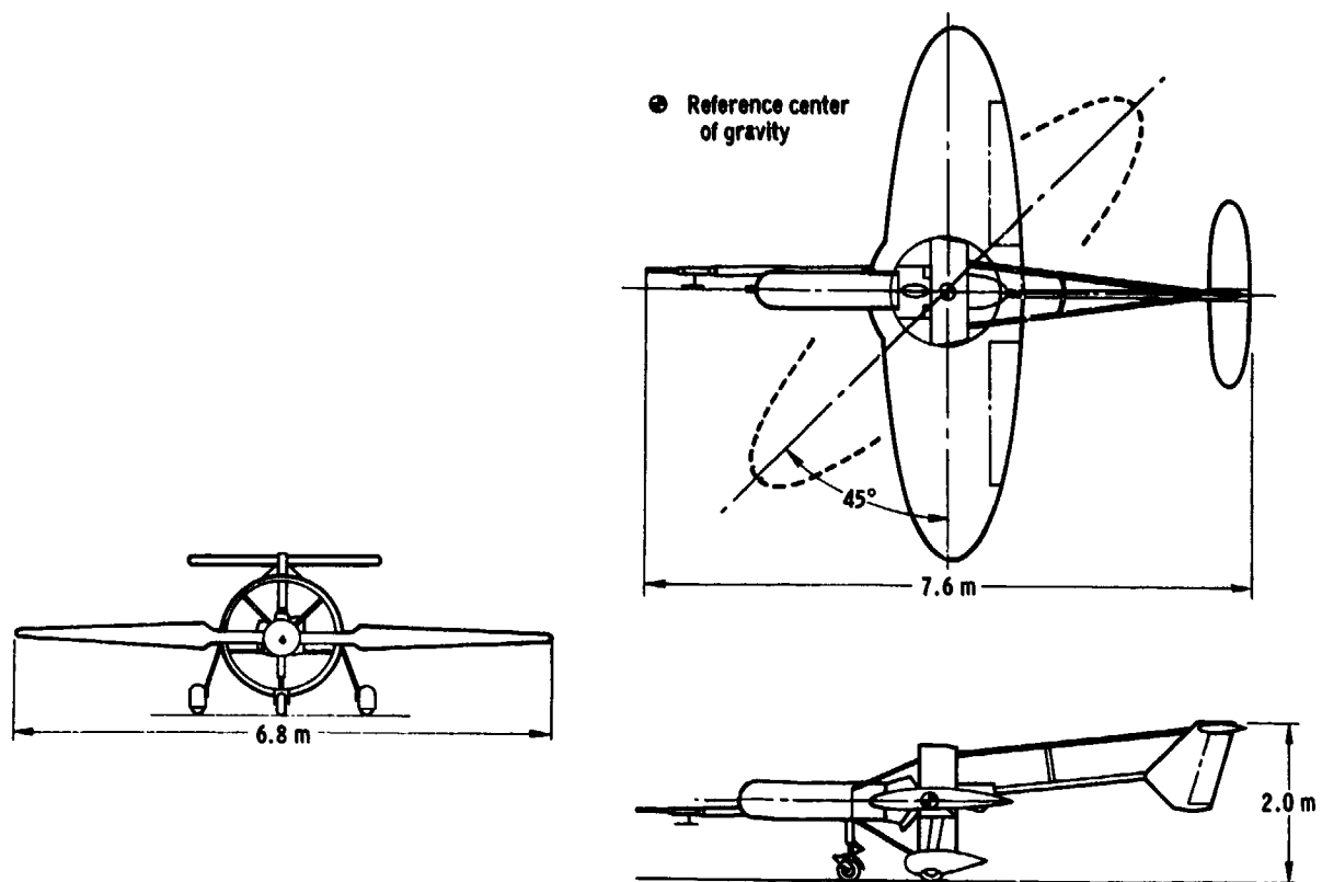
Figure 9.2-1. Oblique-wing aircraft.
