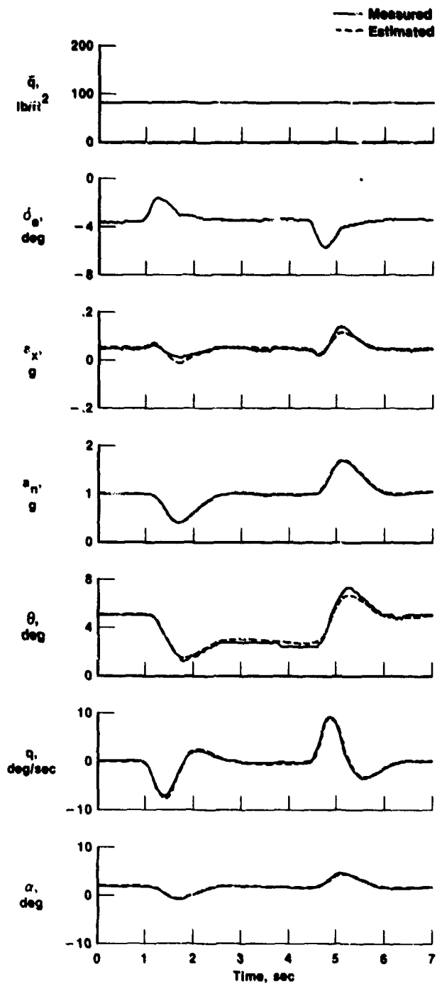
Figure 6.4-4. Longitudinal maneuver of a T-37 aircraft.
