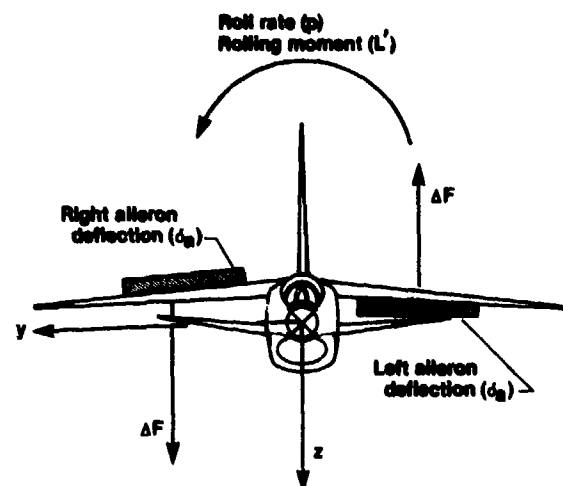
Figure 4.2-1. Simplified aircraft nomenclature.
