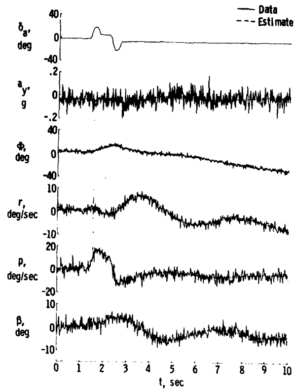
Figure 9.1-4. Time history of simulated data.
