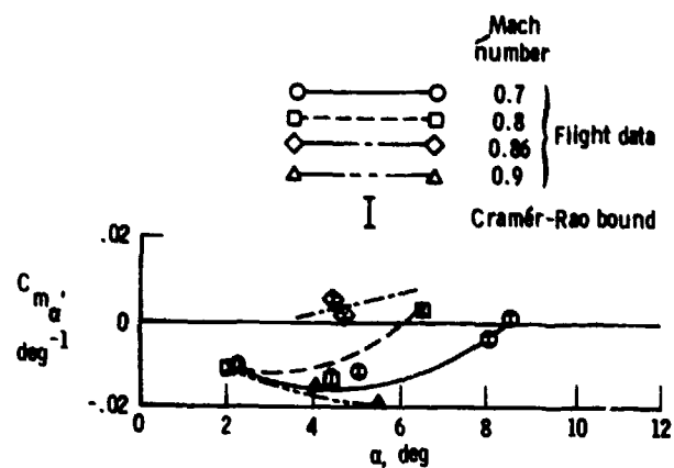
Figure 9.2-10. Estimates of C_{m_\alpha} for F-111A airplane.
