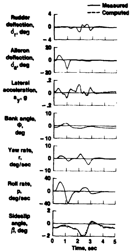
Figure 4.5-5. Lateral-directional maneuver from F-8 aircraft with yaw augmentation on.
