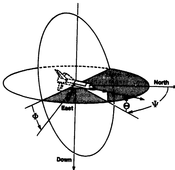
Figure 2.1-3. Euler angles.
