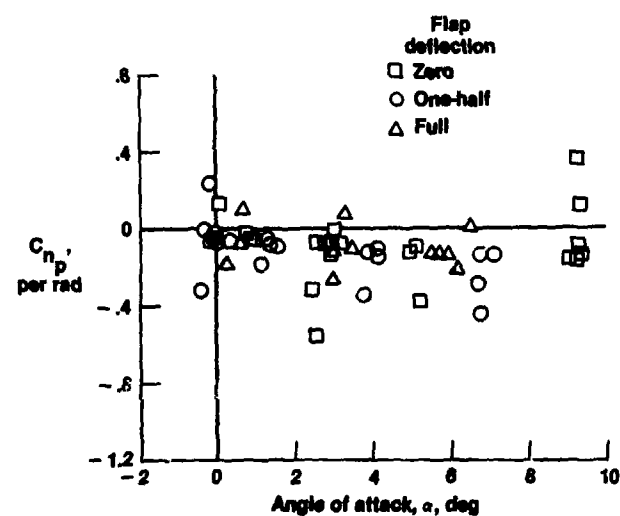
Figure 4.5-7. Variations of C_{n_p} with angle of attack.
