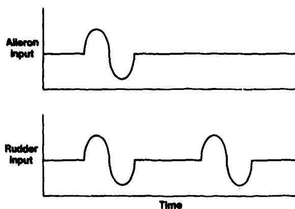
Figure 6.3-1. Combined aileron and rudder input.
