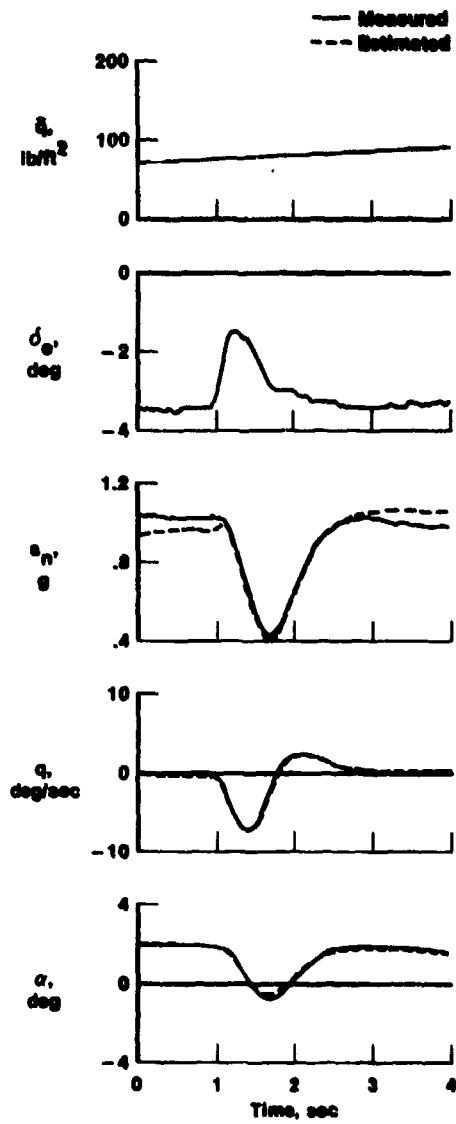
Figure 8.7-1. Fit neglecting dynamic pressure change.
