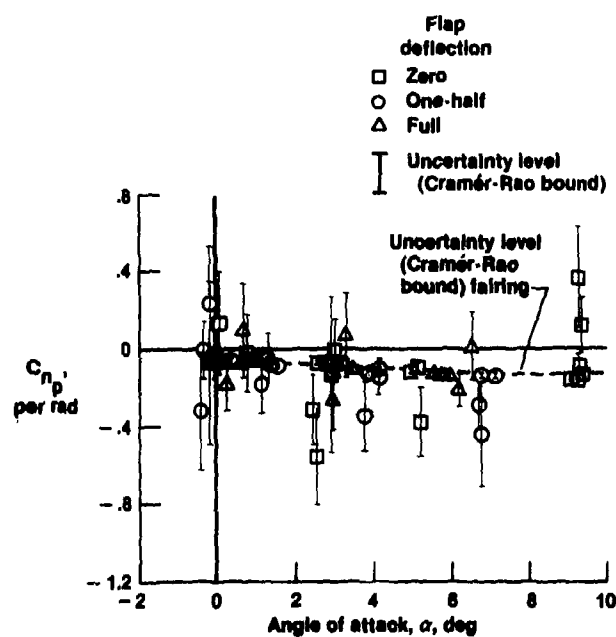
Figure 4.5-8. Variations of C_{n_p} with angle of attack, including uncertainty levels.
