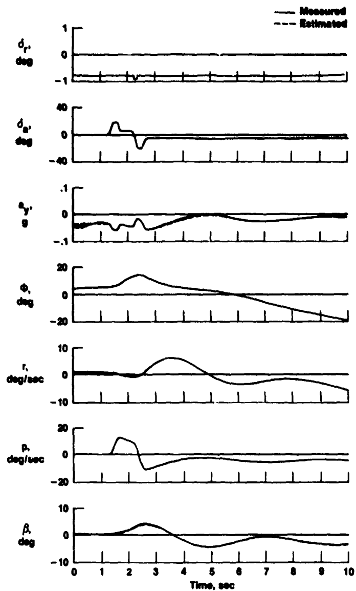
Figure 6.4-8. Aileron maneuver on a Piper PA-30 aircraft.
