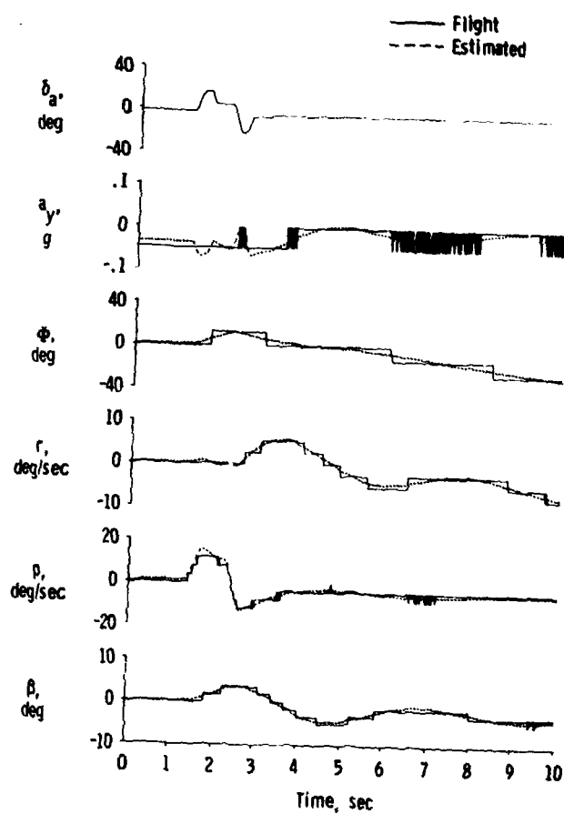
Figure 7.5-2. Resolution reduced by a factor of 16.
