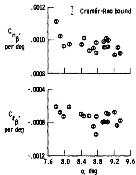
Figure 9.1-3. Estimates of C_{n\beta} and C_{l\beta} from flight data.
