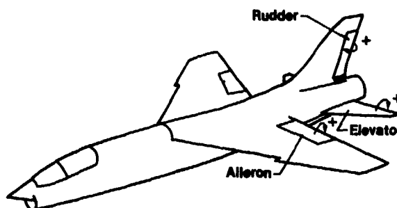
Figure 2.1-1. Control surfaces.
