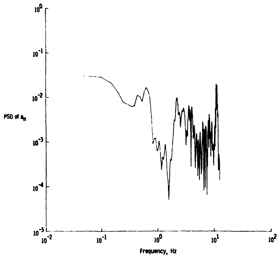
Figure 7.3-4. Power spectral density of 25-sample/sec thinned normal acceleration.
