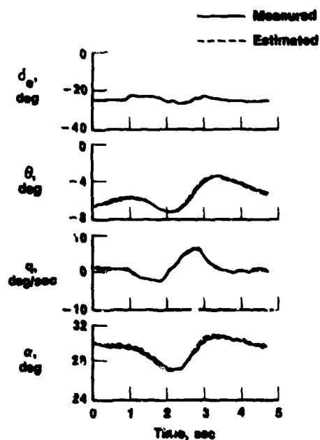
Figure 6.4-5. Longitudinal maneuver of a 3/8-scale F-15 model.
