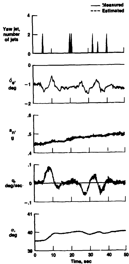
Figure 6.2-3. Tiny longitudinal maneuver of the space shuttle.
