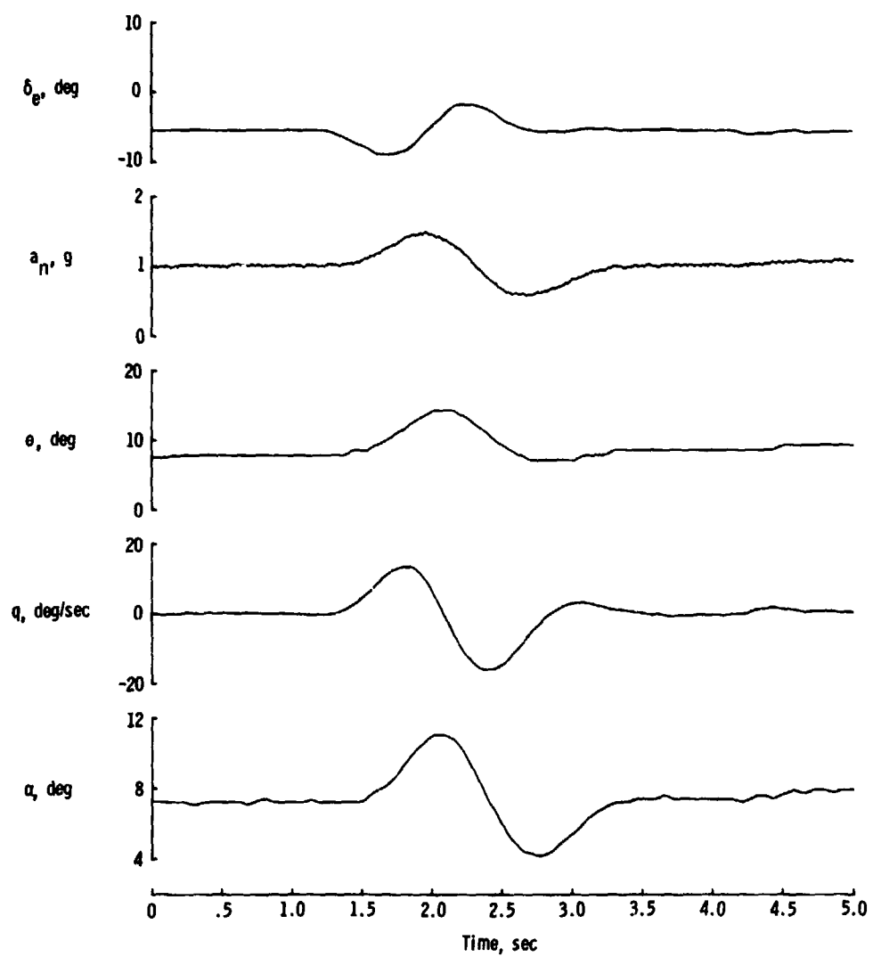
Figure 6.2-2. Time history of filtered data.
