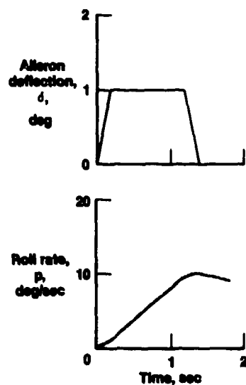
Figure 4.3-1. Time history with no measurement noise.
