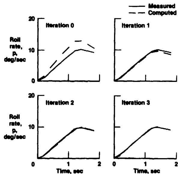
Figure 4.3-2. Comparison of measured and computed data for each of the first three iterations.
