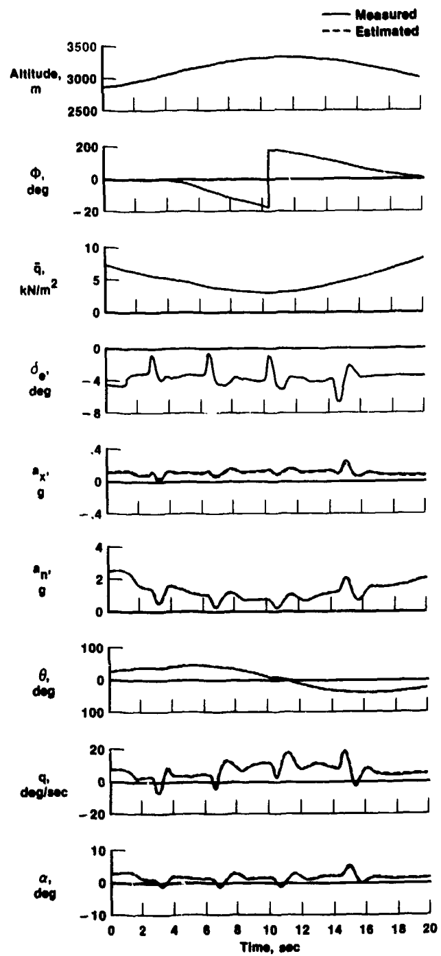
Figure 6.2-4. Small-perturbation maneuver for estimating C_{m\dot{\alpha}} .
