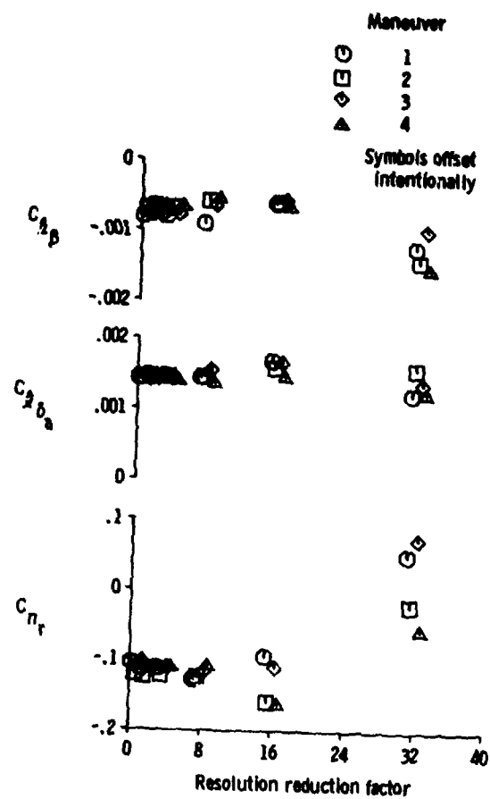
Figure 7.5-3. Derivative estimates as a function of resolution.
