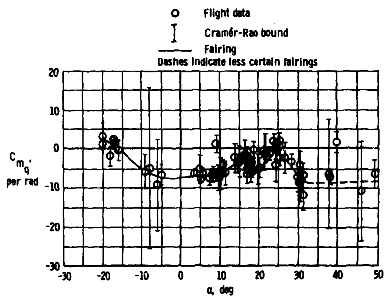
Figure 9.2-4. Estimates of C_{mq} for 3/8-scale F-15 model.
