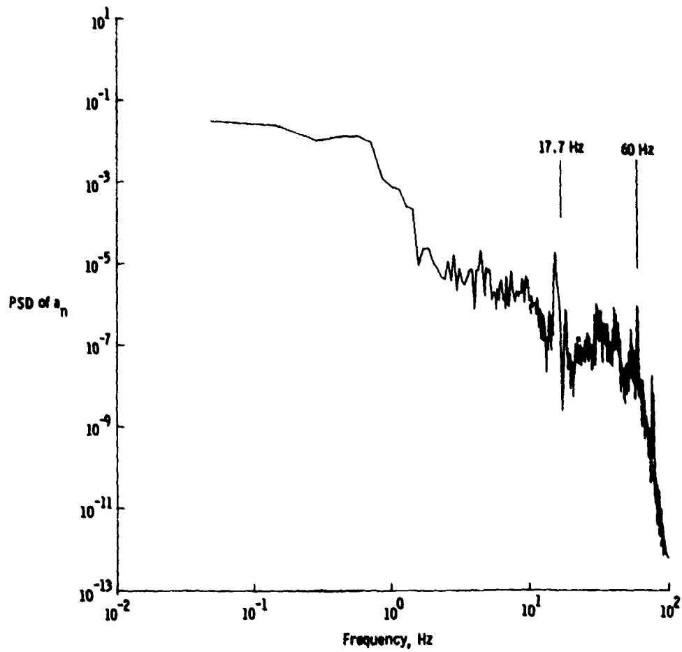
Figure 7.3-5. Power spectral density of filtered normal acceleration.
