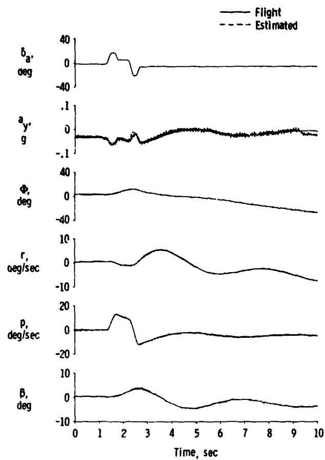
Figure 7.6-1. Piper PA-30 time history.
