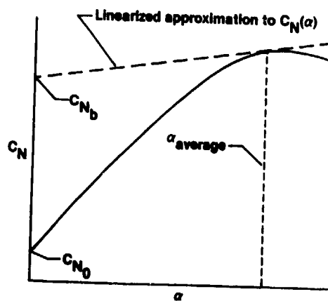
Figure 2.4-1. Relationship of C_{Nb} and C_{N0} .
