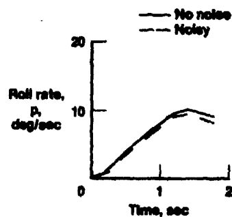
Figure 4.3-5. Comparison of estimated roll rate from no-noise and noisy cases.
