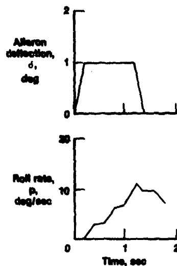
Figure 4.3-3. Time history with measurement noise.
