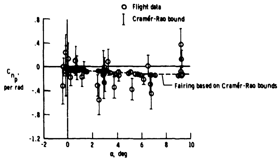
Figure 6.4-9. Estimates of C_{np} on a Piper PA-30 aircraft.
