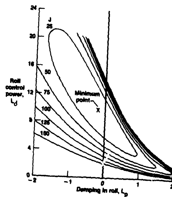
Figure 4.4-11. Isolines of constant cost of L_p and L_d for the no-noise case.
