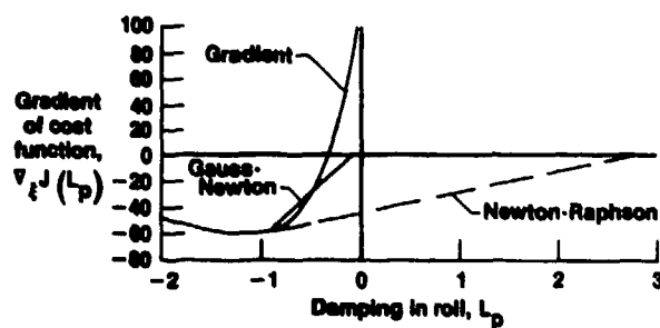
Figure 4.4-8. Comparison of first iteration step size for the Newton-Raphson and Gauss-Newton algorithms for the noisy case.
