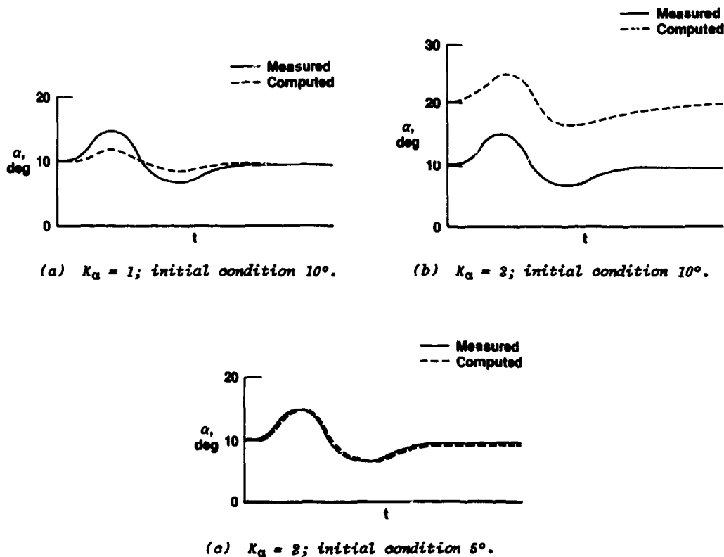
Figure 3.8-1. Angle-of-attack fit.
