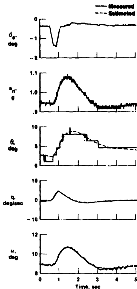
Figure 6.4-6. Longitudinal maneuver of a Piper PA-30 aircraft.
