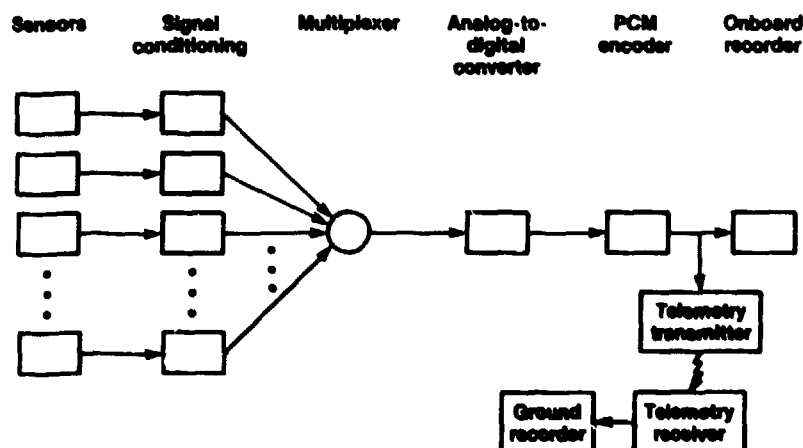
Figure 7.1-1. Simplified PCM system.
