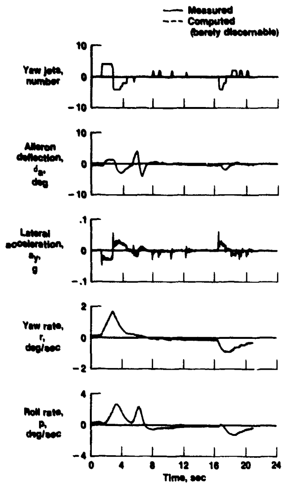
Figure 4.5-4. NNLES match of maneuver shown in Figure 4.5-2.
