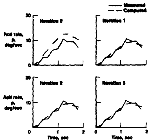
Figure 4.3-4. Comparison of measured and computed data for each iteration.
