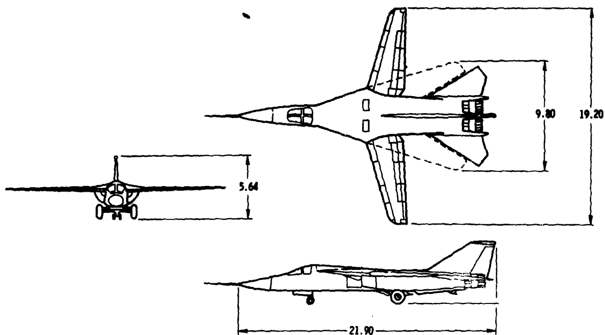
Figure 9.2-7. F-111A airplane (dimensions in meters).
