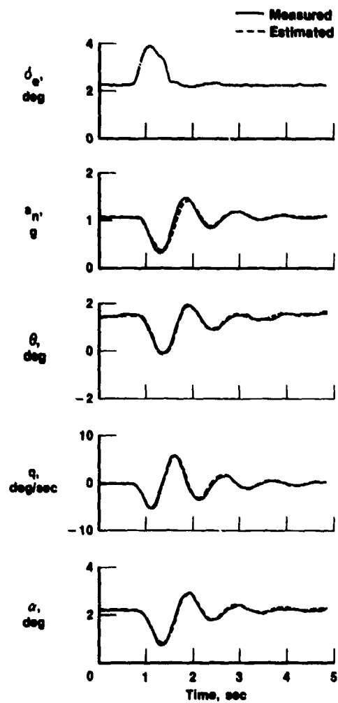
Figure 6.4-2. Longitudinal maneuver of an F-111A aircraft.
