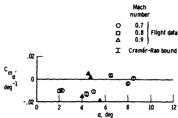
Figure 9.2-8. Estimates of C_{m_\alpha} for F-111A airplanes.
