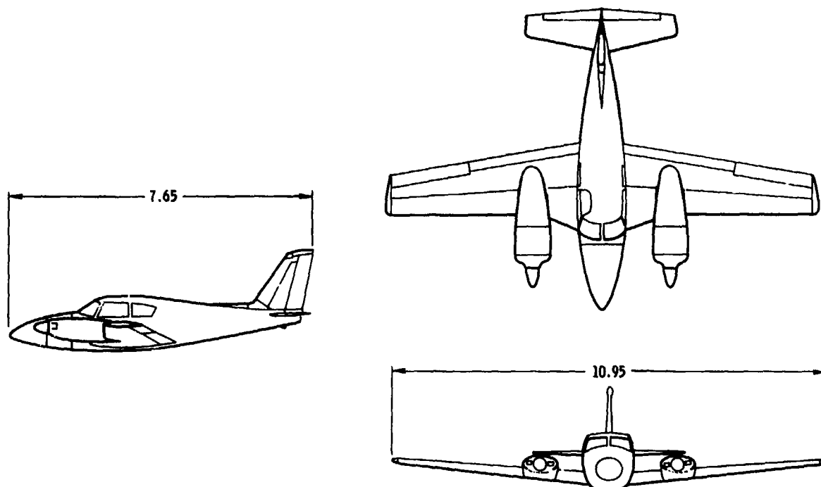
Figure 9.1-1. The PA-30 airplane (dimensions in meters).
