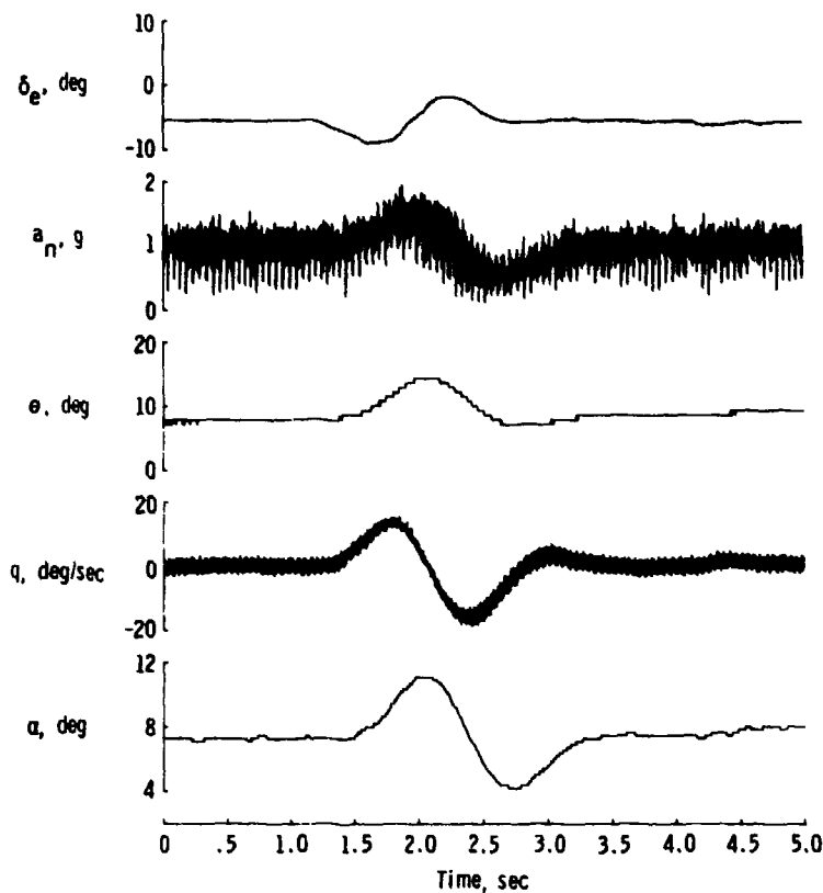
Figure 6.2-1. Oblique-wing 200-sample/sec data.
