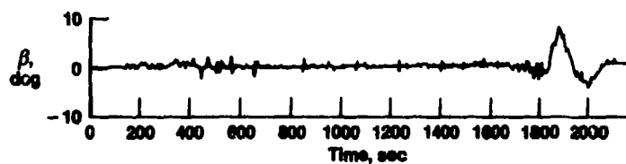
Figure 8.5-4. Inertial sideslip angle during second shuttle entry.
