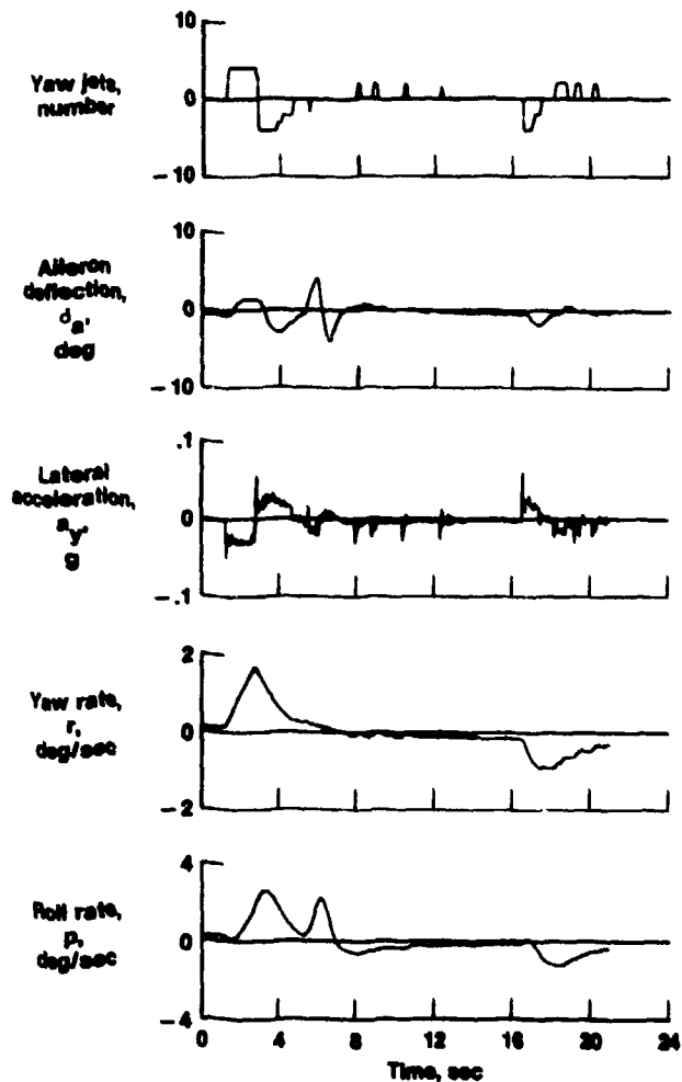
Figure 4.5-2. Lateral-directional space shuttle maneuver at a Mach number of 21.
