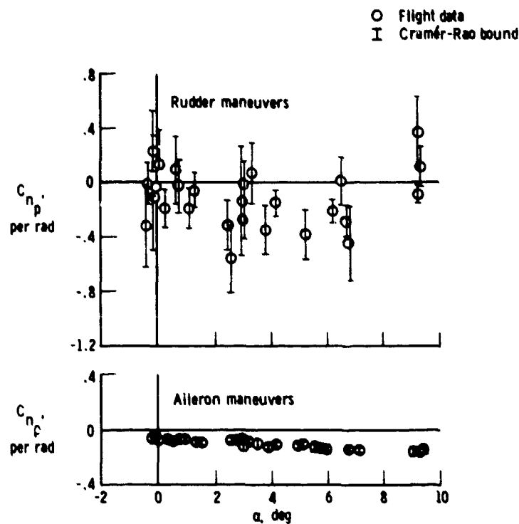
Figure 6.4-10. Estimates of C_{np} , segregated by maneuver type.
