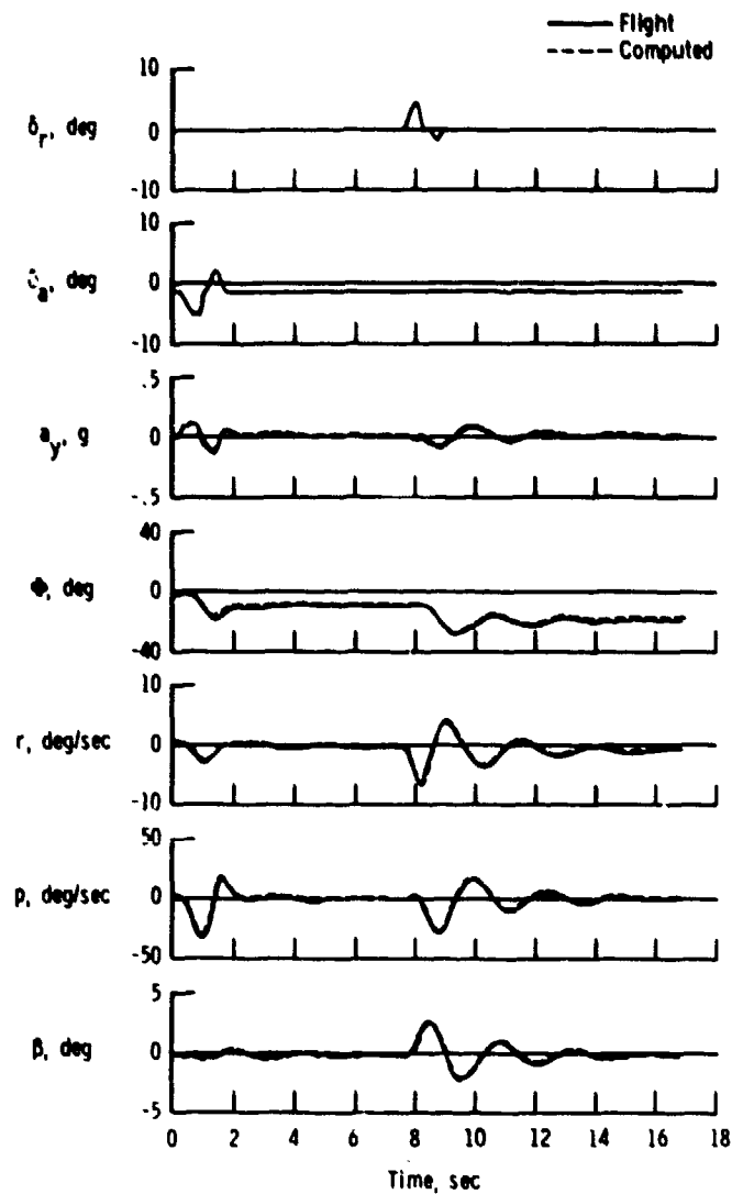
Figure 6.4-12. Lateral-directional maneuver of an F-8C aircraft.
