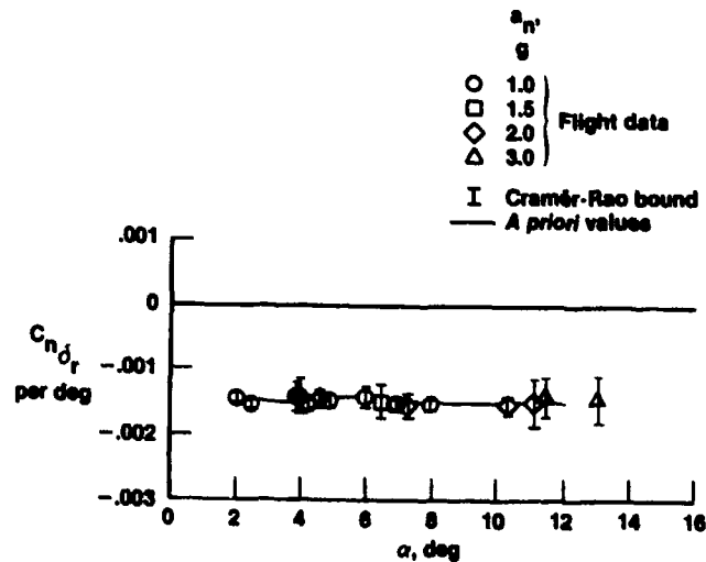
Figure 9.2-12. Estimates of C_{n_{\delta_r}} for F-111A airplane.
