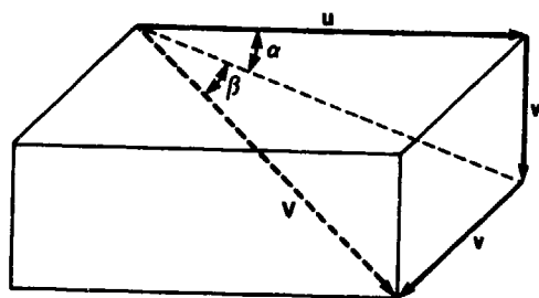
Figure 2.1-4. Flow angles.
