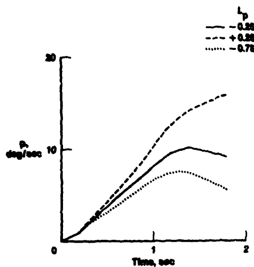
Figure 4.4-2. No-noise response for correct L_p ( -0.2500 ) compared with the response for L_p = -0.75 and L_p = 0.25 .
