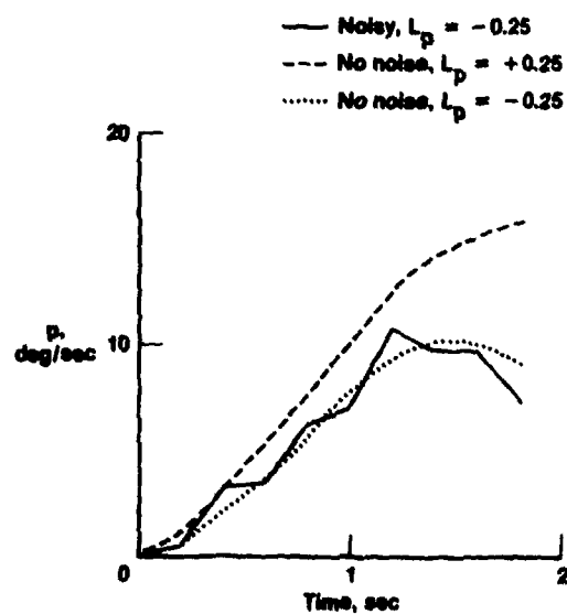
Figure 4.4-5. Response for an L_p of +0.25 compared with the no-noise and noisy response for L_p at the correct value of -0.25 .
