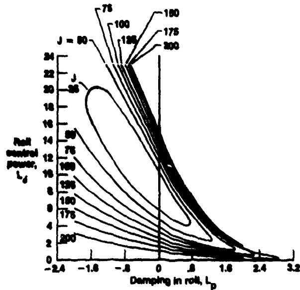
Figure 4.4-13. Isolines of constant cost in L_p and L_d for the noisy case.
