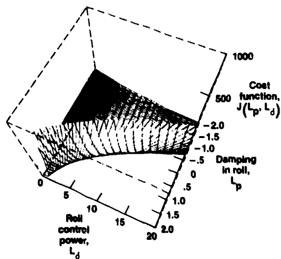
Figure 4.4-9. Large-scale view of cost function surface.
