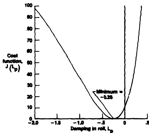
Figure 4.4-1. Cost function J(L_p) as a function of L_p for no-noise case.
