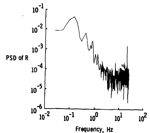
Figure 9.1-7. Noise spectra of flight data residuals.
