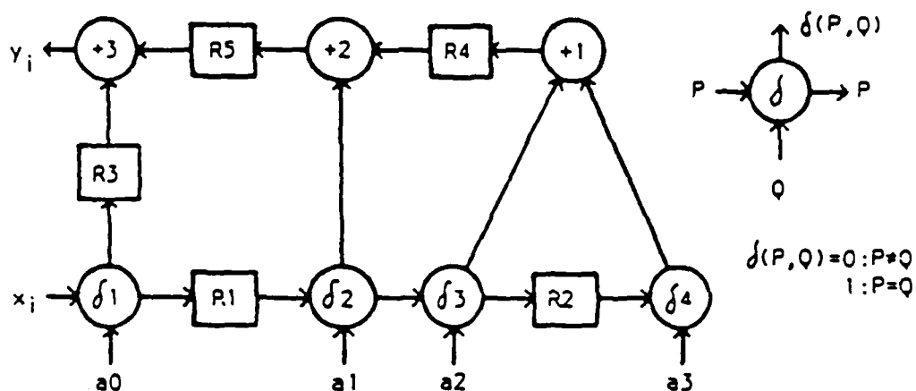
A systolic array evaluating \sum_{j=0}^3 x_{i,j} \cdot a_j .
