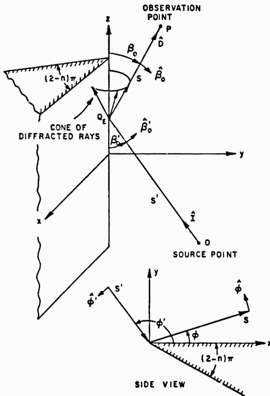
FIGURE 2-1. GEOMETRY FOR THREE-DIMENSIONAL WEDGE DIFFRACTION PROBLEM
