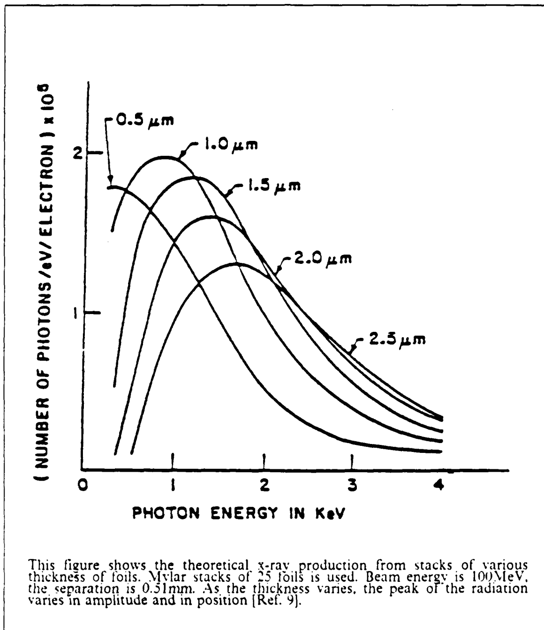
Figure 2.4 Theoretically predicted spectrum.
