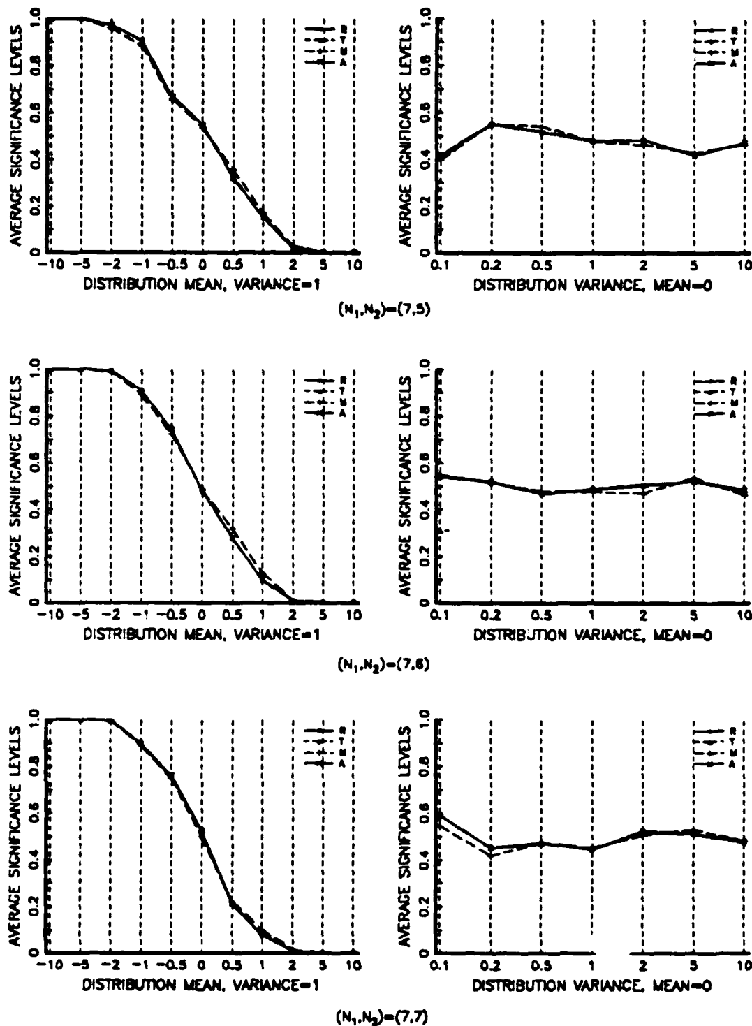
Figure 6. Two Sample Normal Distributional Changes
