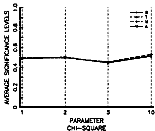
Figure 5. Two Sample Concurrent Changes in Continuous Distributions
