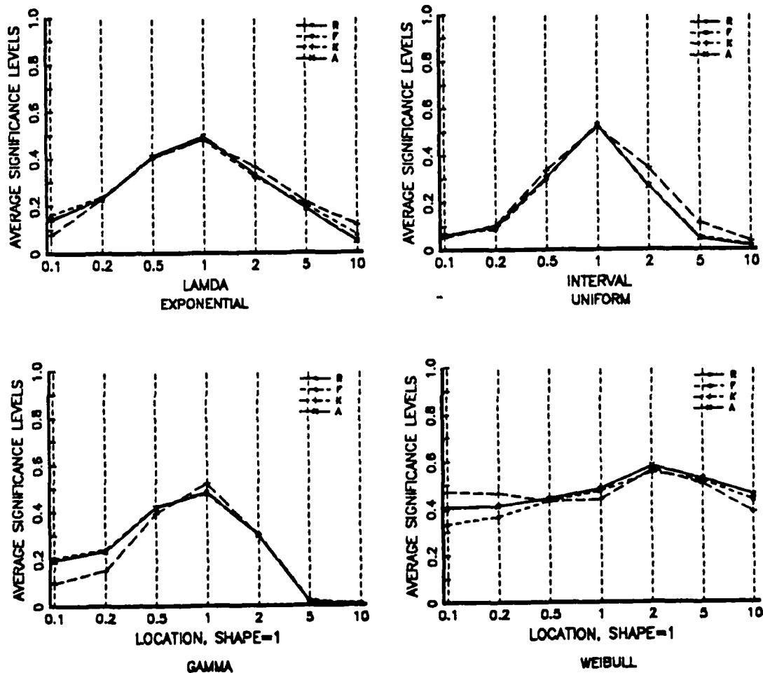
Figure 17. ANOVA Continuous Distributional Changes
