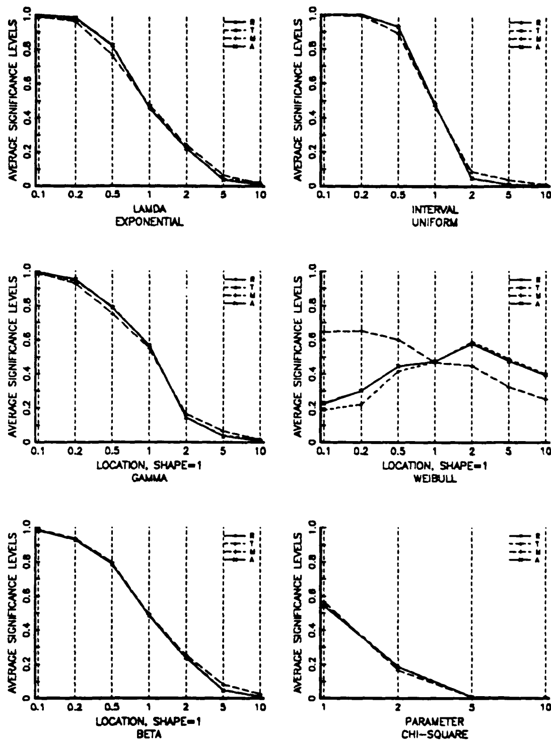
Figure 7. Two Sample Continuous Distributional Changes
