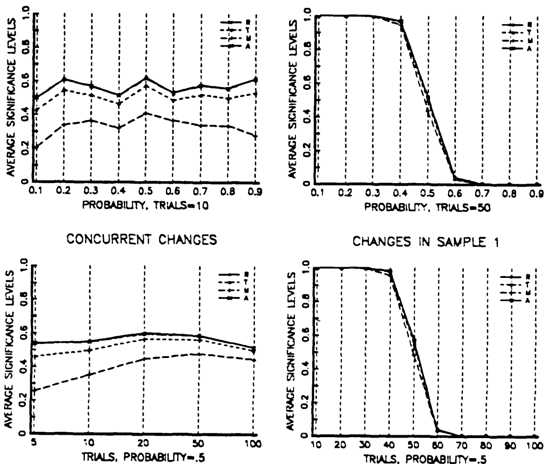
Figure 8. Two Sample Binomial Distributional Changes
