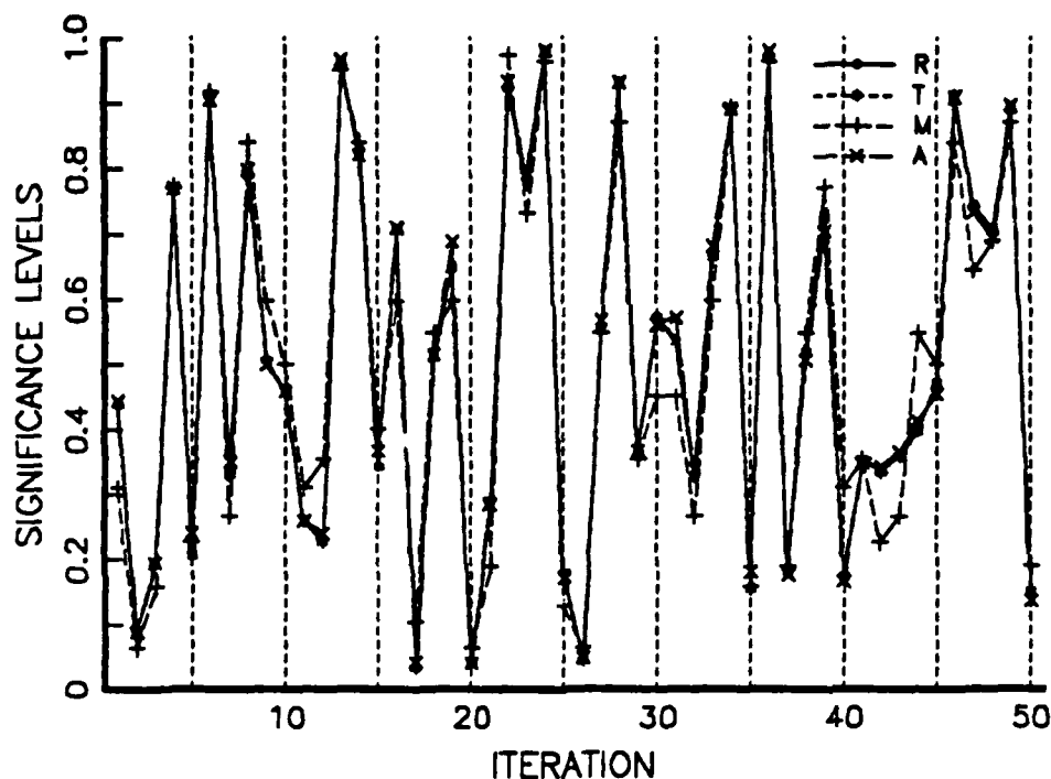
Figure 3. Two Sample Significance Levels by Iteration
