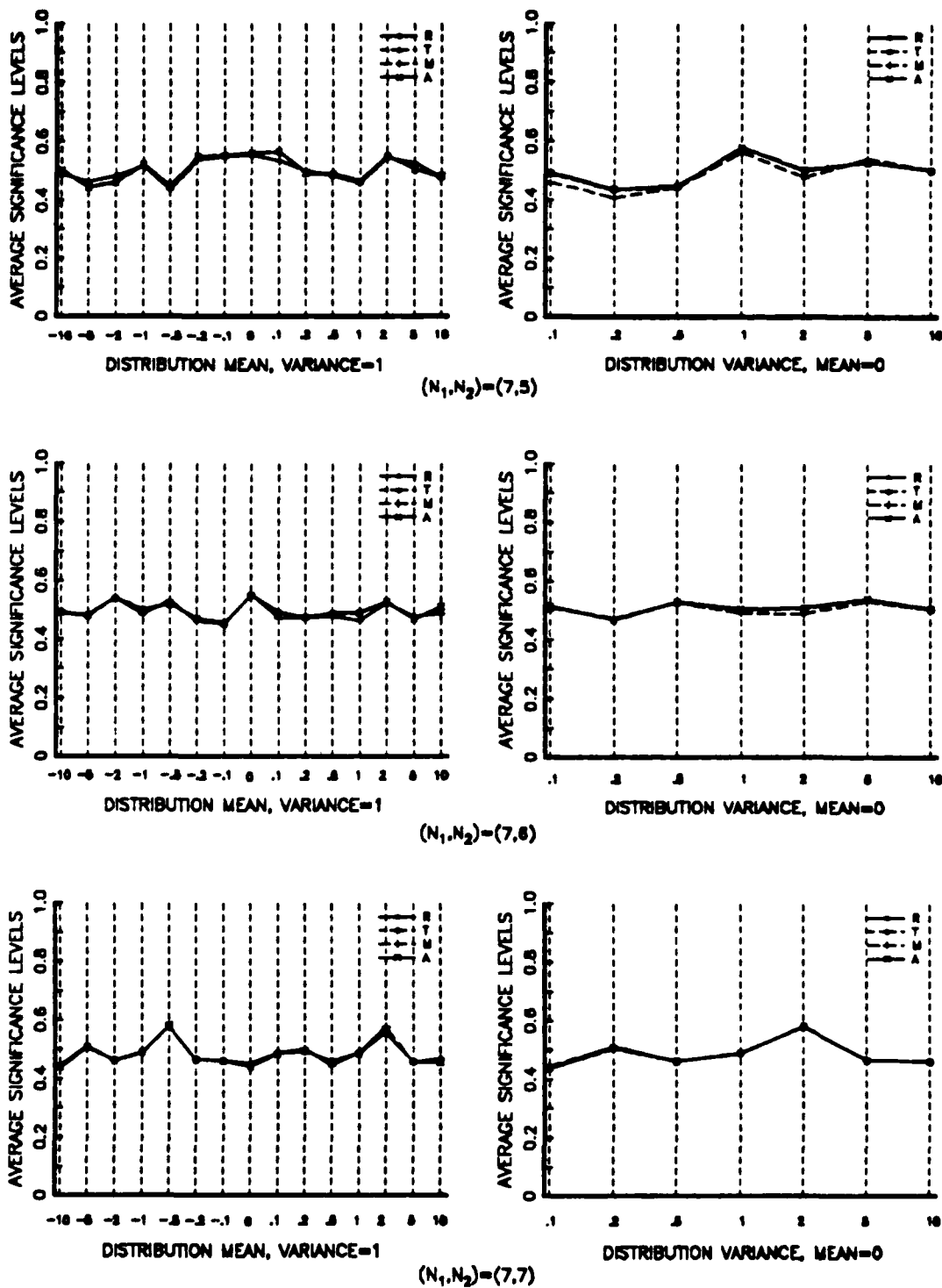
Figure 4. Two Sample Concurrent Changes in Normal Distributions
