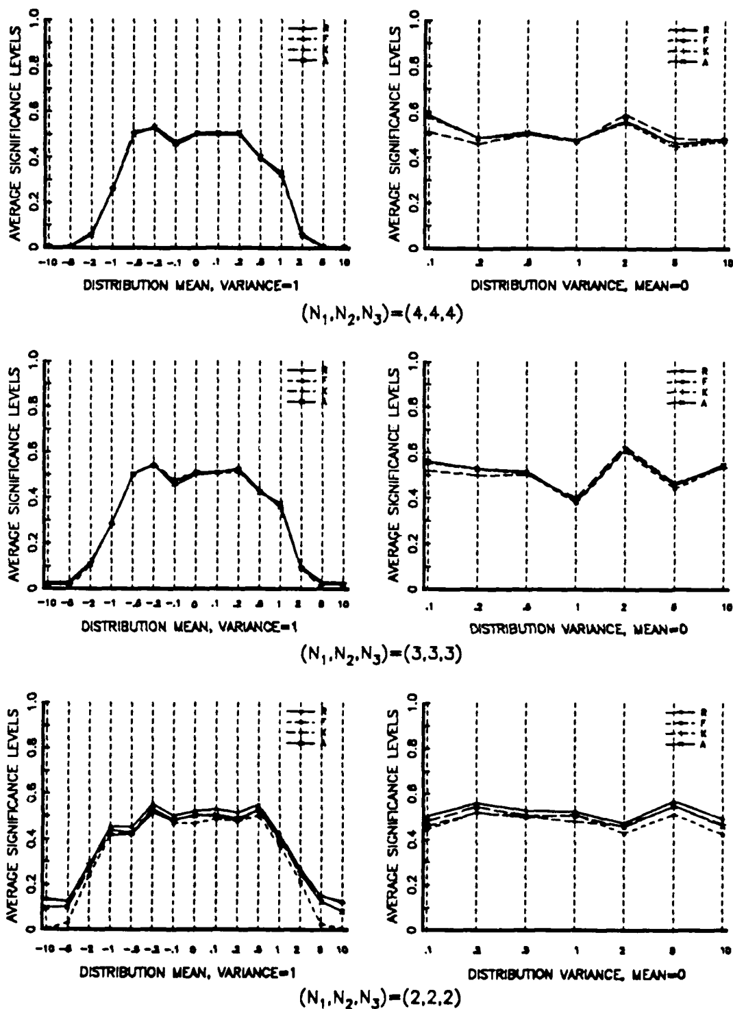
Figure 16. ANOVA Normal Distributional Changes
