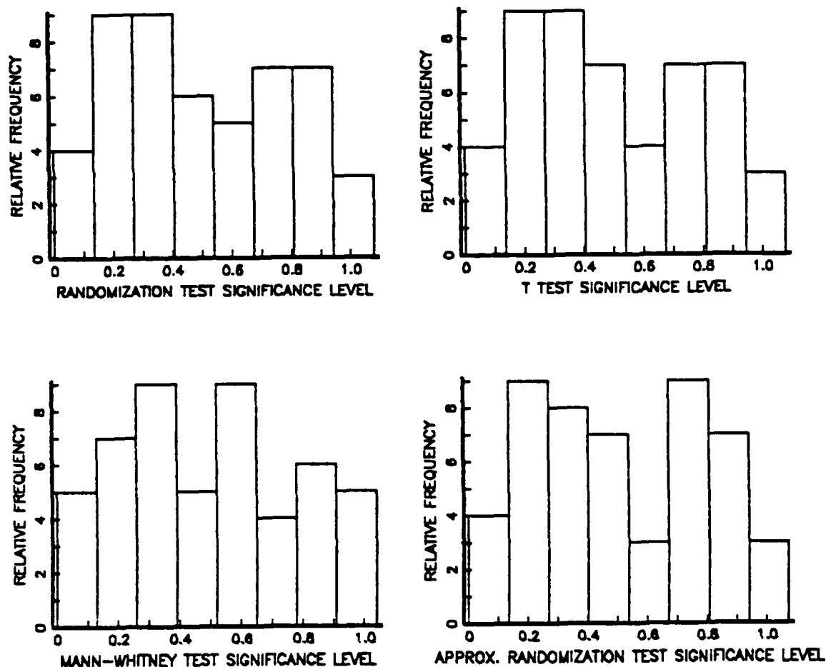
Figure 2. Two Sample Histograms for N(0,1) Samples
