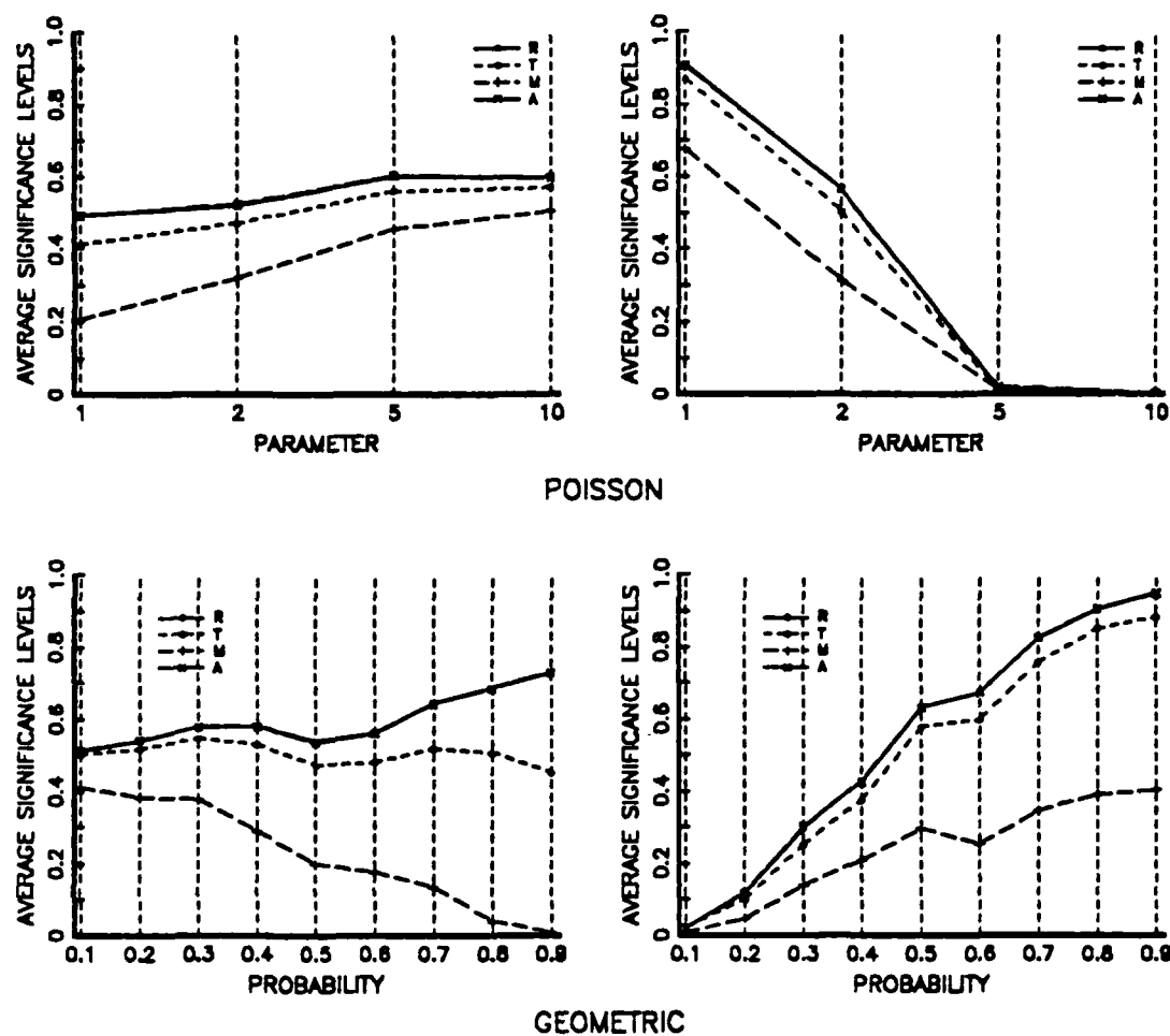
Figure 9. Two Sample Poisson and Geometric Distributional Changes
