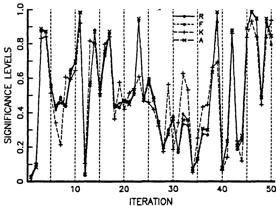
Figure 13. ANOVA Significance Levels by Iteration
