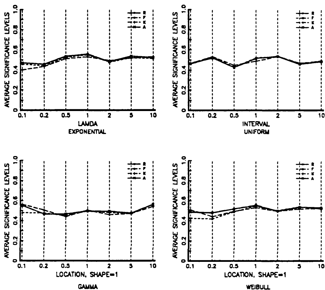
Figure 15. ANOVA Concurrent Changes in Continuous Distributions
