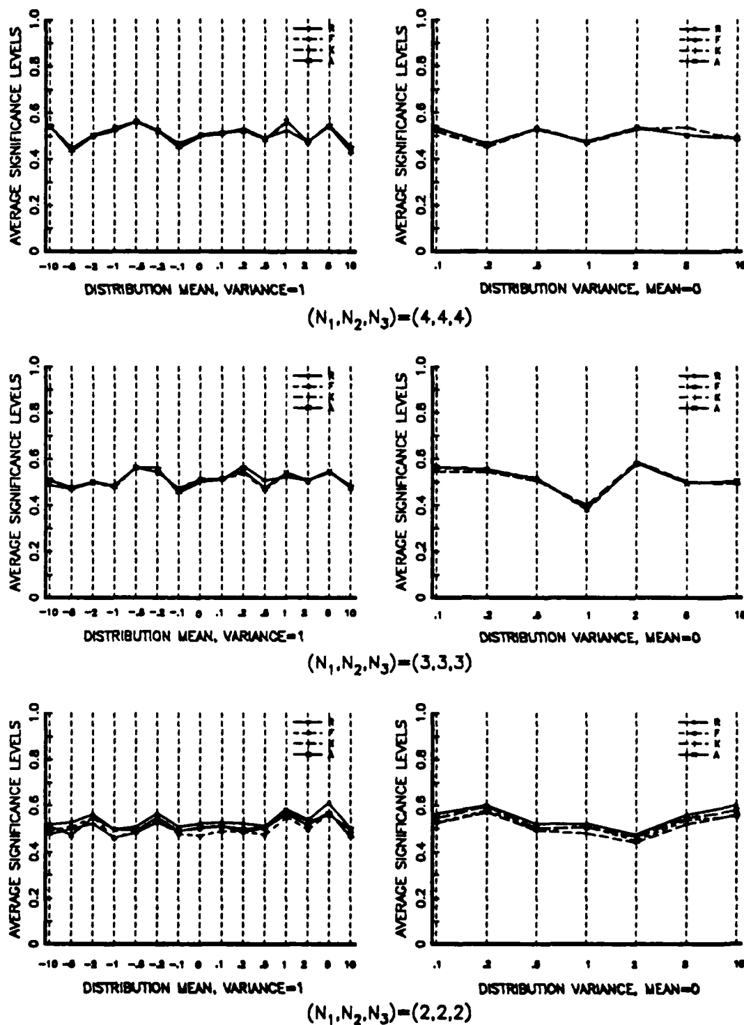
Figure 14. ANOVA Concurrent Changes in Normal Distributions
