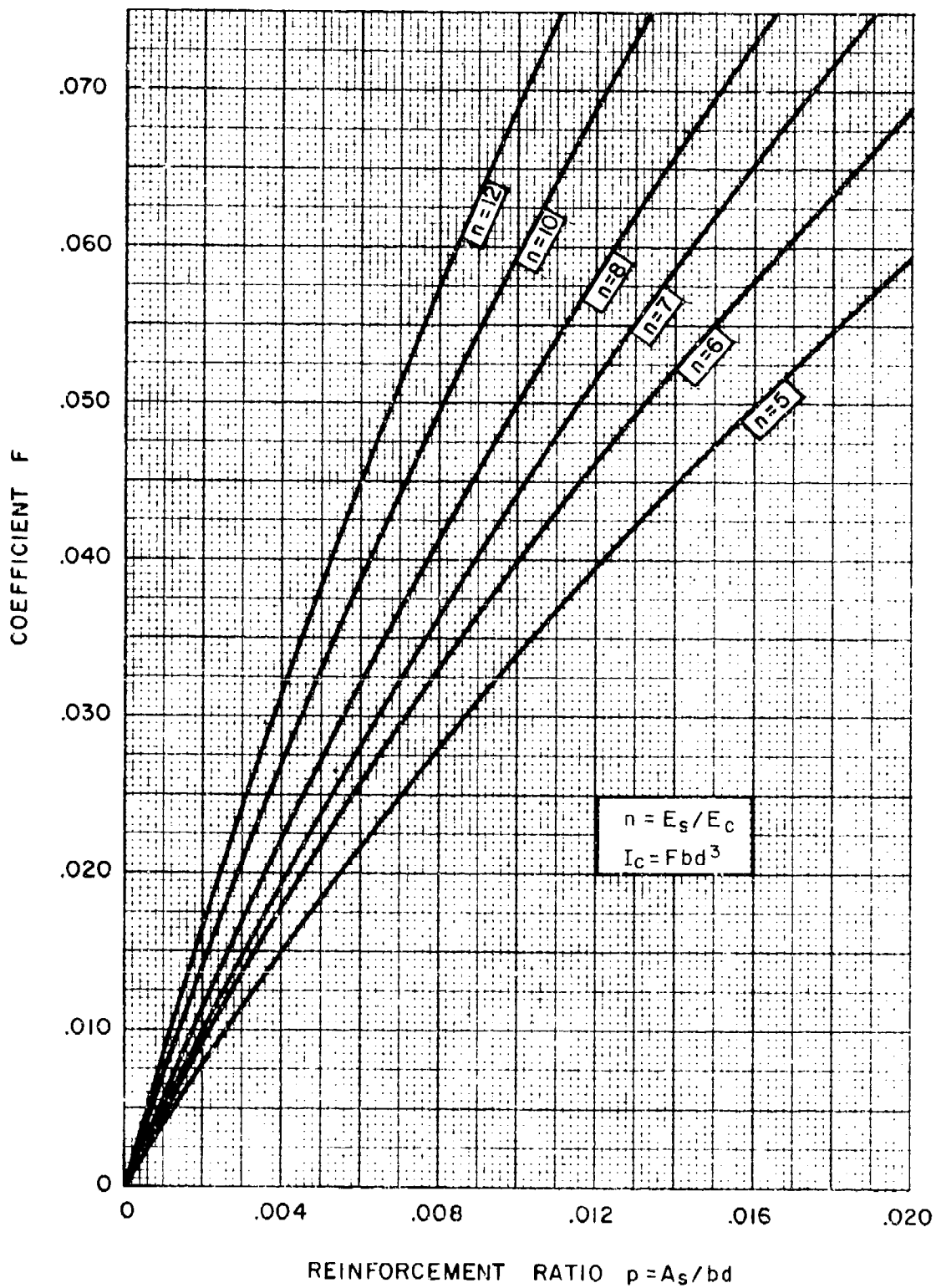
Figure 4-12 Coefficient for moment of inertia of cracked sections with equal reinforcement on opposite faces
