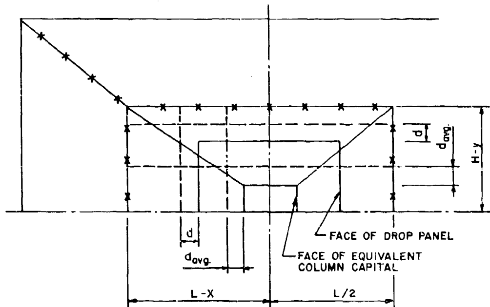
b. BEAM SHEAR
