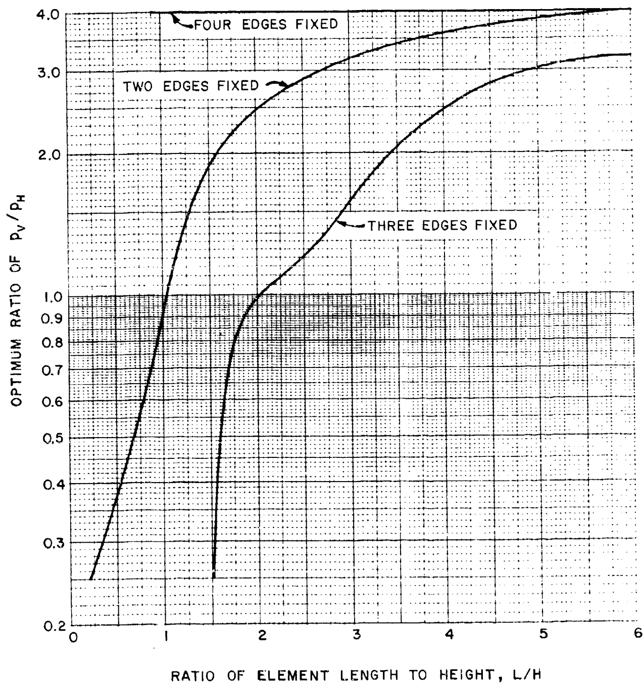
Figure 4-38 Optimum ratio of p_v/p_h for maximum capacity at incipient failure, x_u
