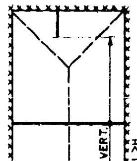
c) THREE SIDES SUPPORTED AND ONE SIDE FREE
