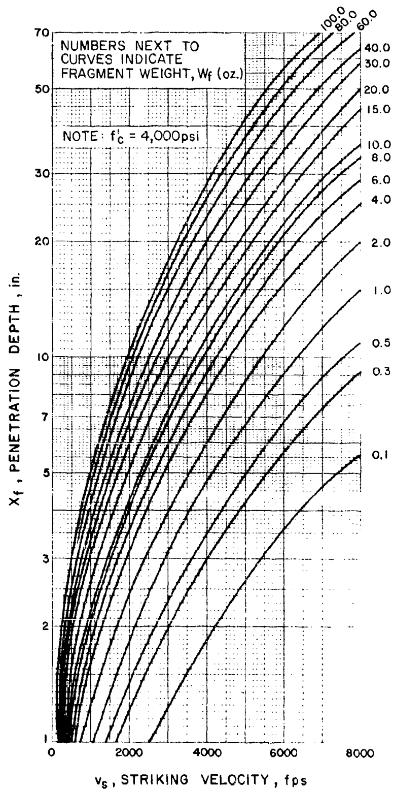
Figure 4-78 Concrete penetration chart for armor-piercing steel fragments
