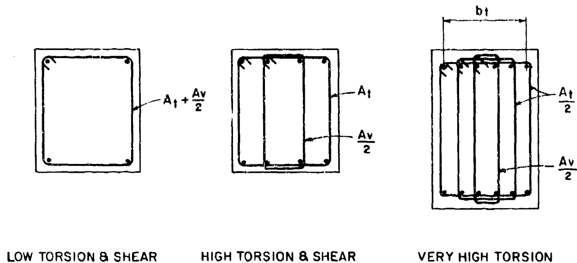
(a) Arrangement of Shear and Torsional Web Reinforcement
