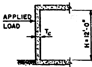
SECTION
