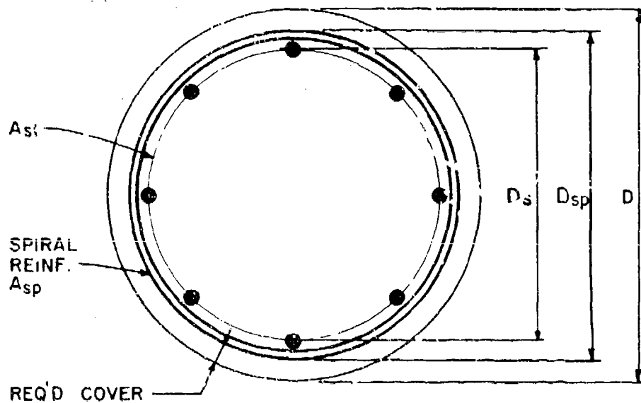
b) CIRCULAR SECTION WITH UNIFORMLY DISTRIBUTED REINFORCEMENT
