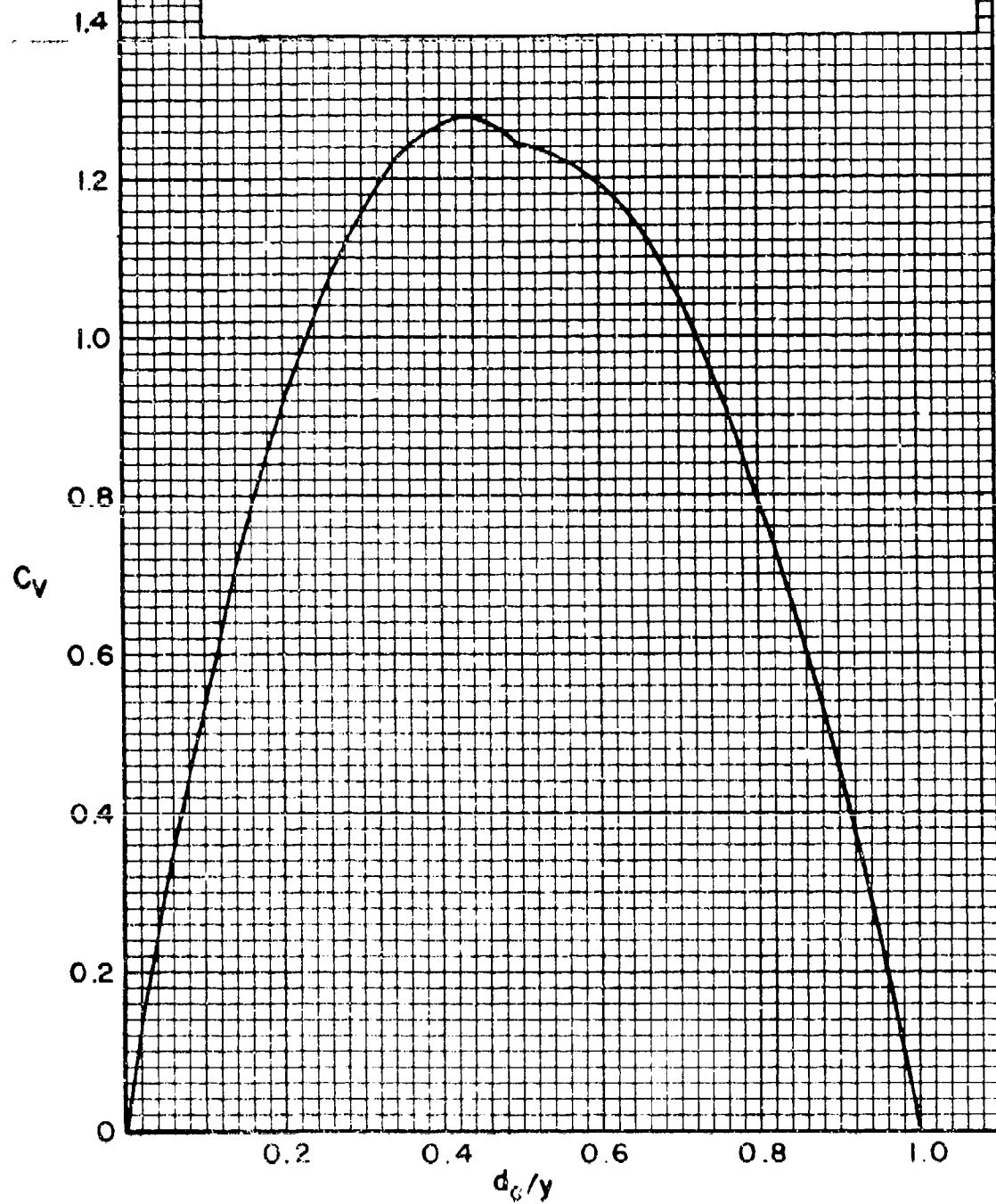
Figure 4-39 Vertical shear coefficients for ultimate shear stress at distance d_c from the support (cross section type 11 and 111)
