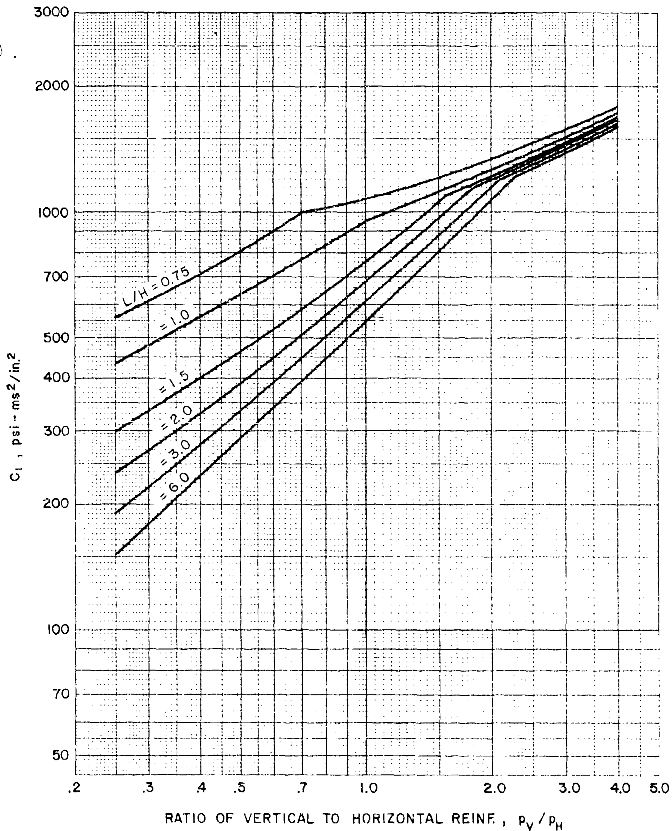
Figure 4-32 Impulse coefficient C_I for an element with four edges fixed
