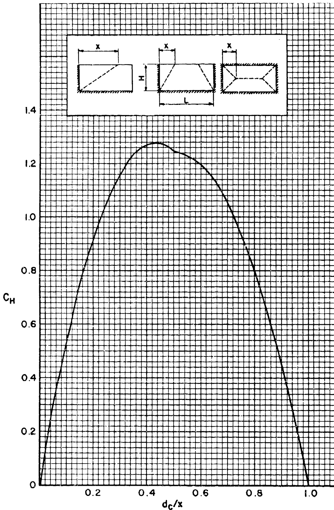
Figure 4-40 Horizontal shear coefficients for ultimate shear stress at distance d_c from the support (cross section type 11 and 11i)
