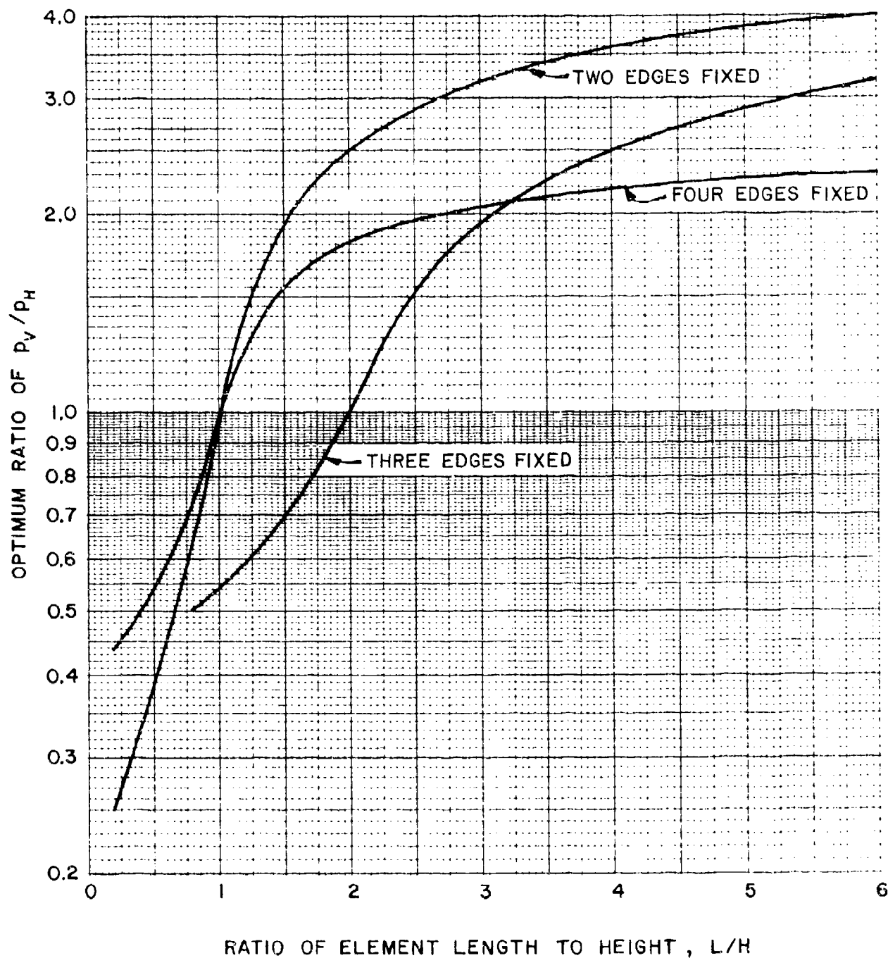
Figure 4-37 Optimum ratio of p_v/p_h for maximum capacity at partial failure deflection, x_1
