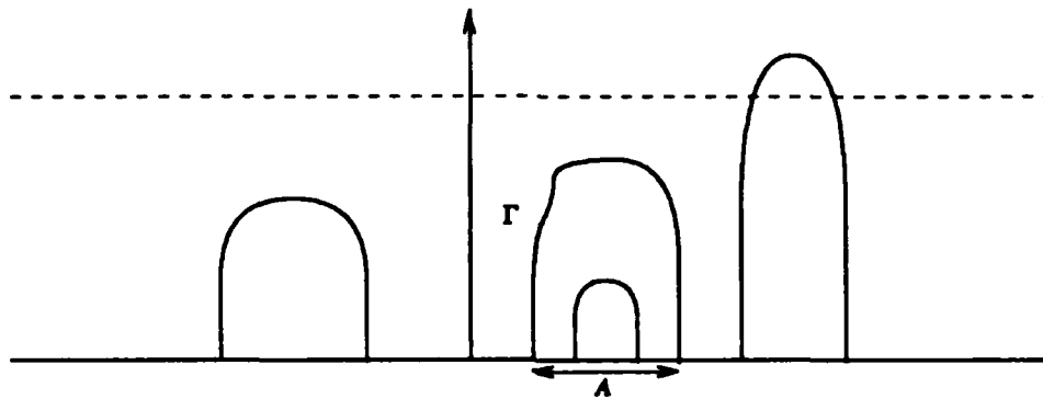
Figure 5. Reconstruction of data on segment A is theoretically possible given the gradient data on the zero-crossing curve \Gamma . The reconstruction requires deblurring data that is computed along the dashed line.
