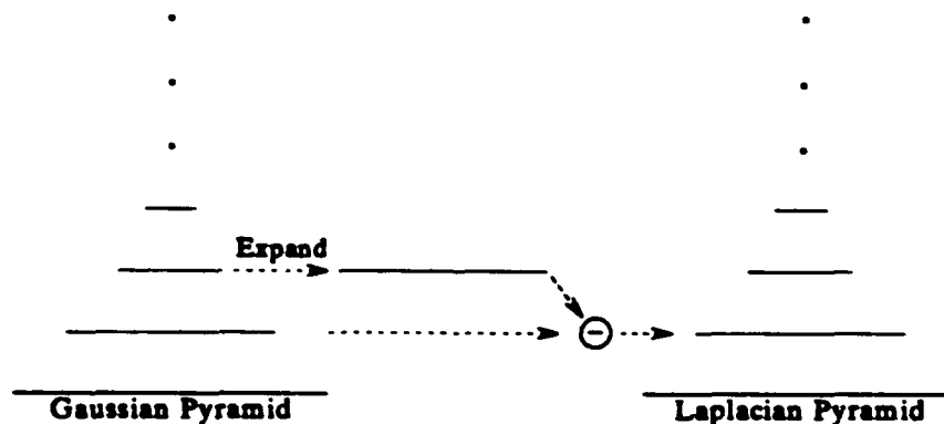
Figure 2. The Burt construction of the Laplacian pyramid.
