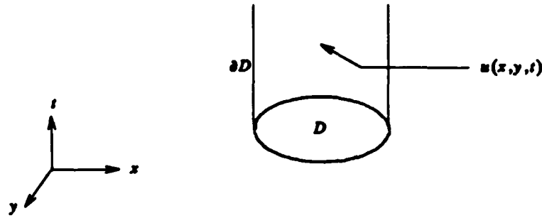
Figure 1. Scale-space for a bounded domain D .
