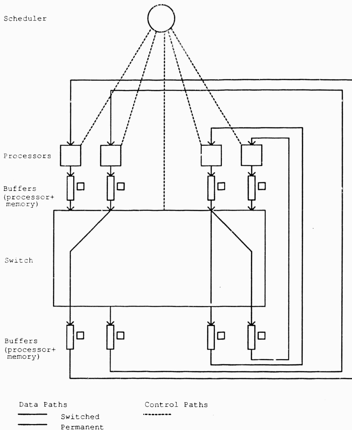
Figure 1 -- Physical Components
