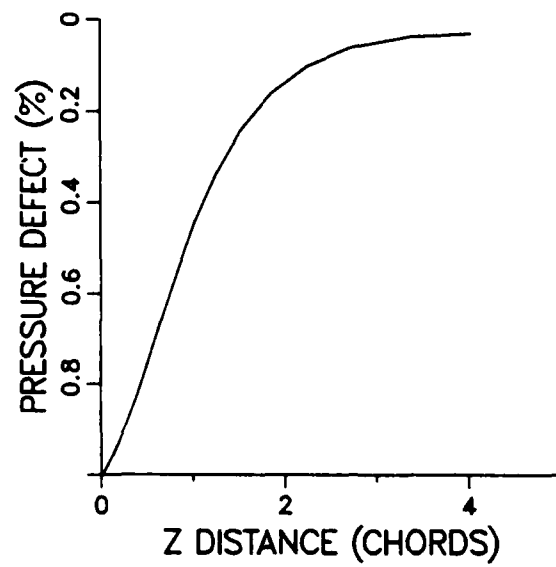
Fig. 5 Pressure prediction in the x direction. Pressure location is on the sonic cylinder at midchord.
