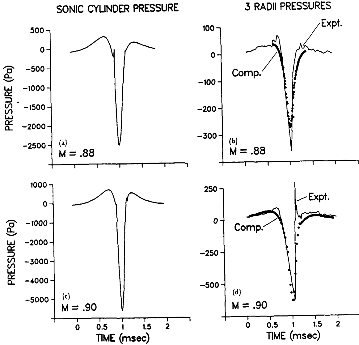
Fig. 4 Acoustic pressure predictions for two hover tip Mach numbers, M = .8 and M = .9 .
