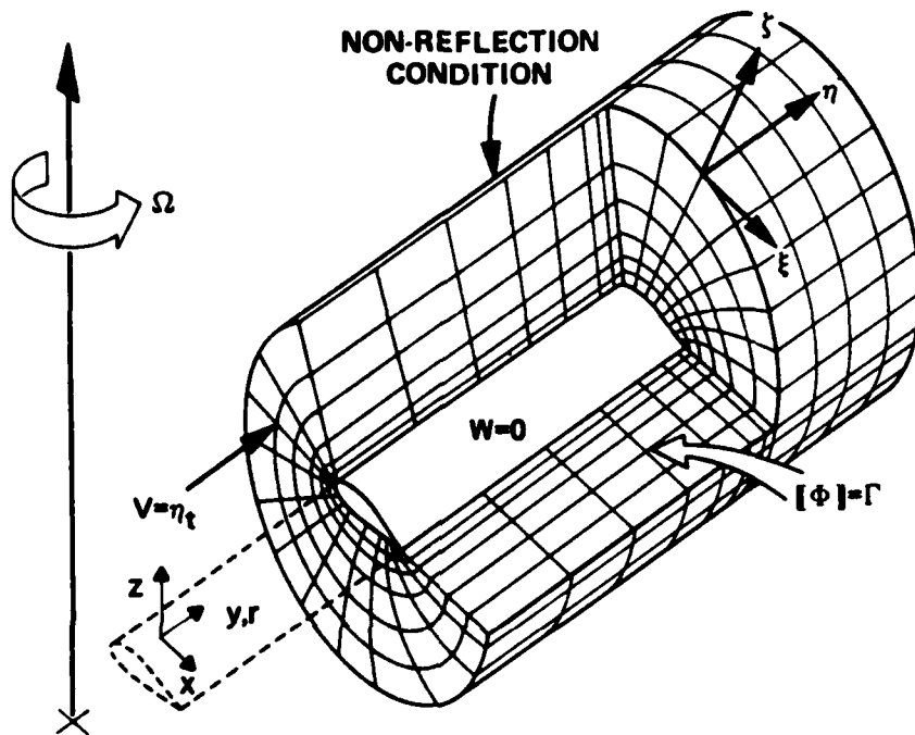
Fig. 1 Grid and boundary conditions for the FPR code.
