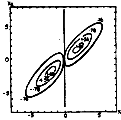
(b) \rho = .9
