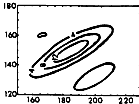
(b) \lambda = 1
