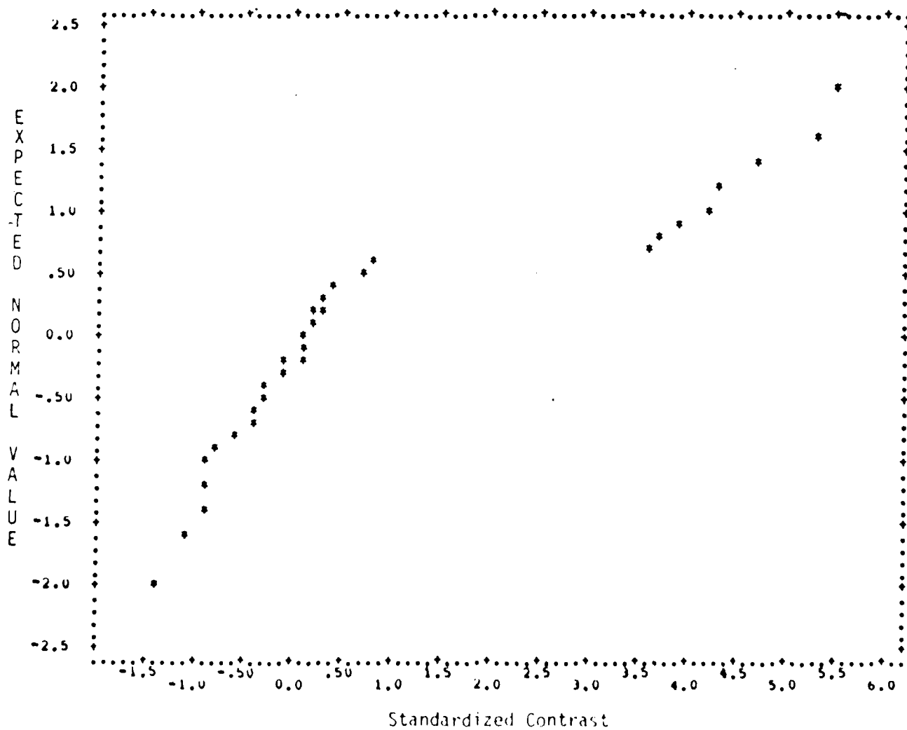
Figure 8 b. Individual Plots for Situation: n=32 , k=31 , r=8\% , d=1.67\sigma
