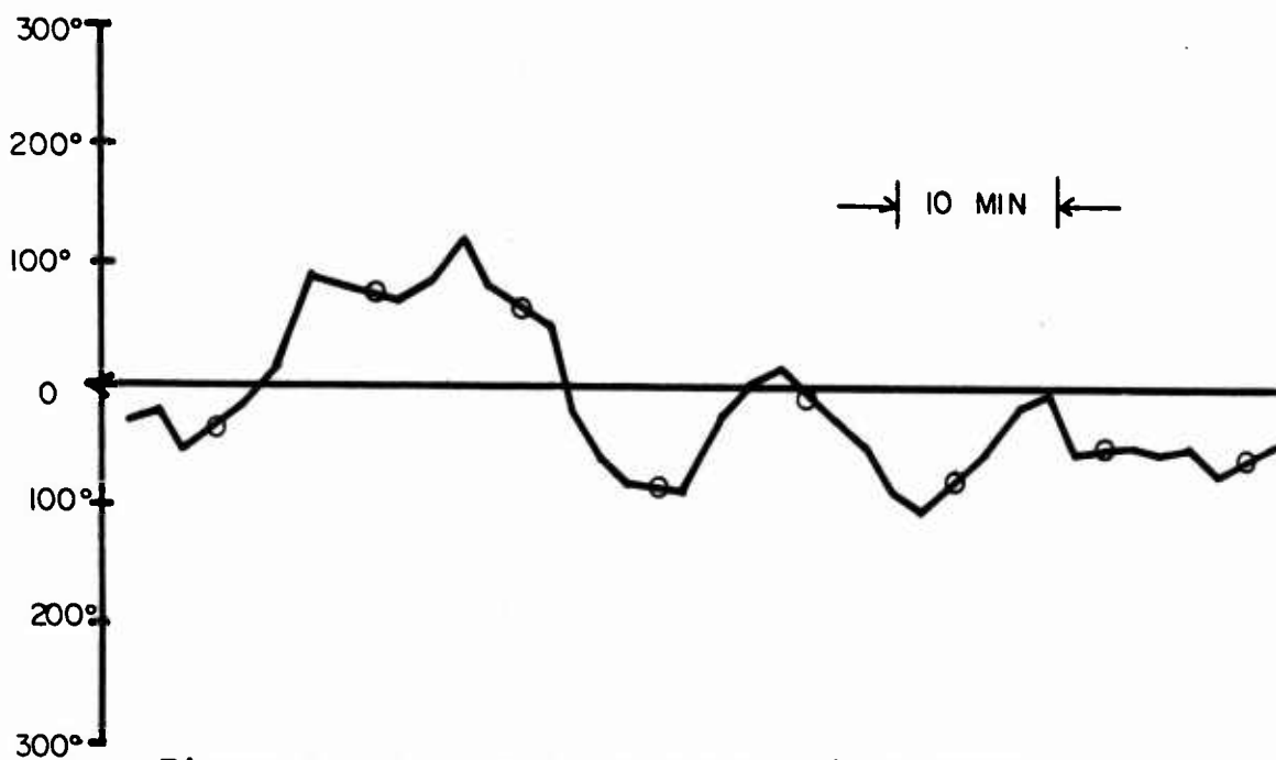
Figure 6. Averaged phase variations over a one hour period
