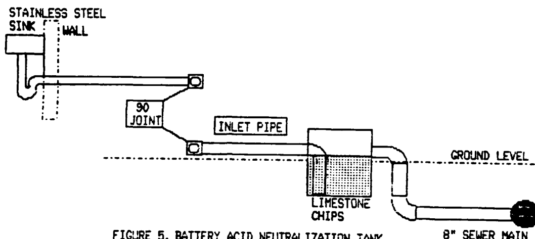
FIGURE 5. BATTERY ACID NEUTRALIZATION TANK PATRICK AFB
