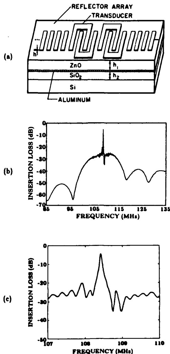
Fig. 1. (a) Schematic of a typical two-port ZnO/SiO 2 /Si SAW resonator. (b) Two-port transmission response for a ZnO-on-Si SAW resonator. (c) Two-port transmission response without transverse modes.
