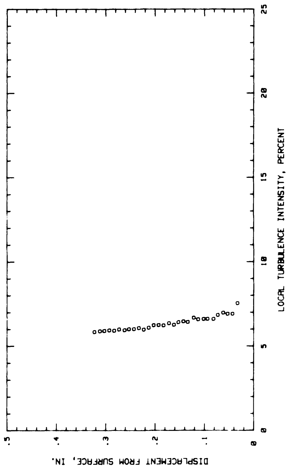
Fig. 82. Boundary Layer Turbulence Intensity Profile, Conf. #2 at 29.68 % Chord
