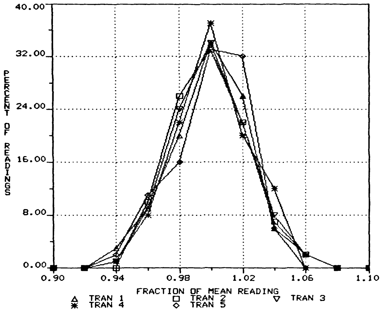
Figure 7. Scatter in Transducer Readings for Pressure Transducers 1 through 5
