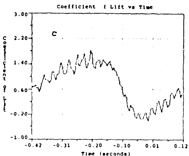
Figure 33. Results from Run KK \alpha_{ND, up} = .0195 , \alpha_{ND, down} = .0524
