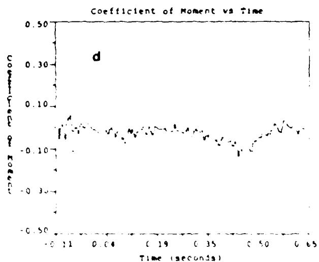
Figure 25. Results from Run CC \dot{\alpha}_{ND,up} = .0109 , \dot{\alpha}_{ND,down} = .0368 a) Angle of Attack Profile, b) Effect on C_L c) Effect on C_D , d) Effect on C_M
