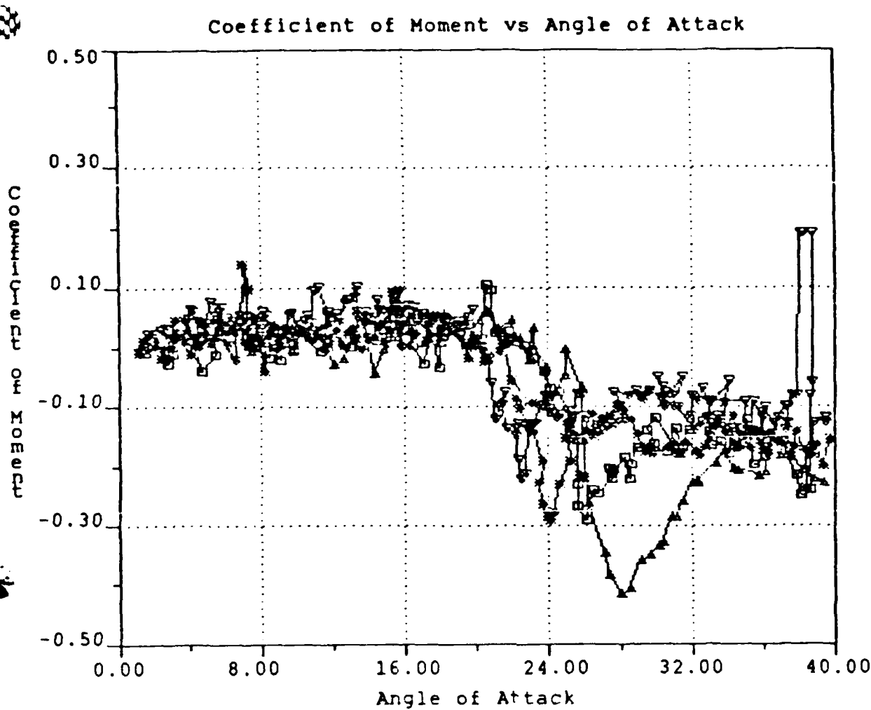
Figure 6. Effect of Pitch Rate on the Moment Curve \dot{\alpha}_{ND} = 0.0097, 0.0134, 0.0224, 0.0297
