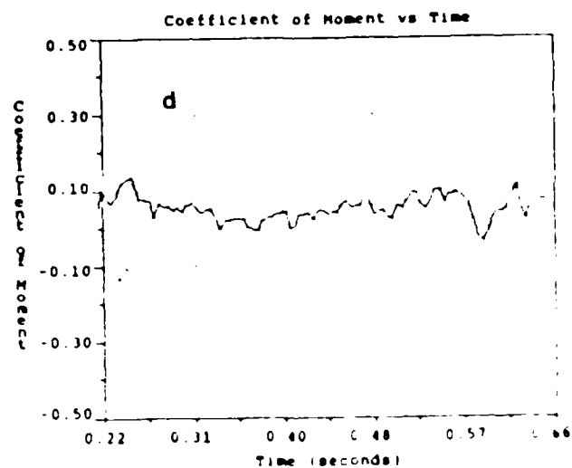
Figure 38. Results from Run PF \alpha_{ND_{up}} = .0320 , \alpha_{ND_{down}} = .0663 a) Angle of Attack Profile, b) Effect on C_L c) Effect on C_D , d) Effect on C_M
