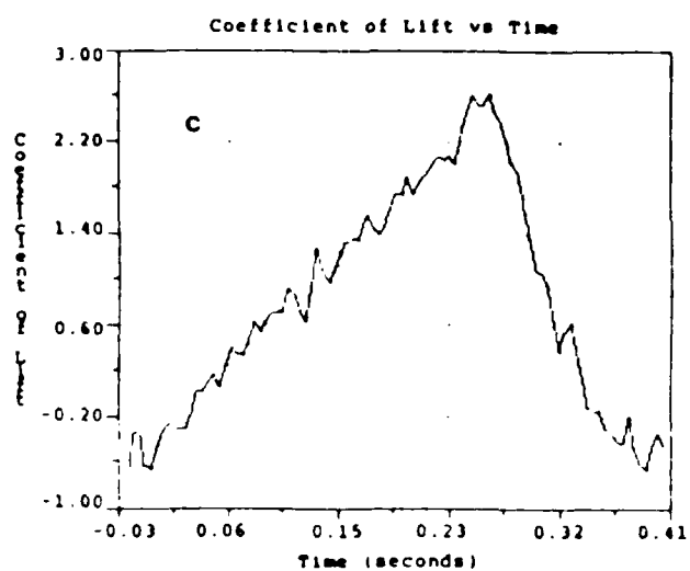
Figure 40. Results from Run RR \dot{\alpha} = .0384 , \dot{\alpha} = .0928 a) Angle of Attack Profile, b) Effect on C_D , c) Effect on C_L , d) Effect on C_M
