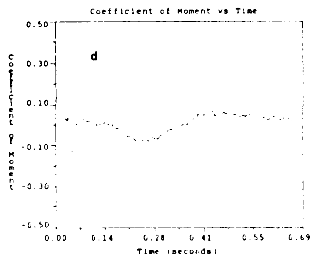
Figure 20. Results from Run J \dot{\alpha}_{ND,up} = .0187 , \dot{\alpha}_{ND,down} = .0244 a) Angle of Attack Profile, b) Effect on C_L c) Effect on C_D , d) Effect on C_M
