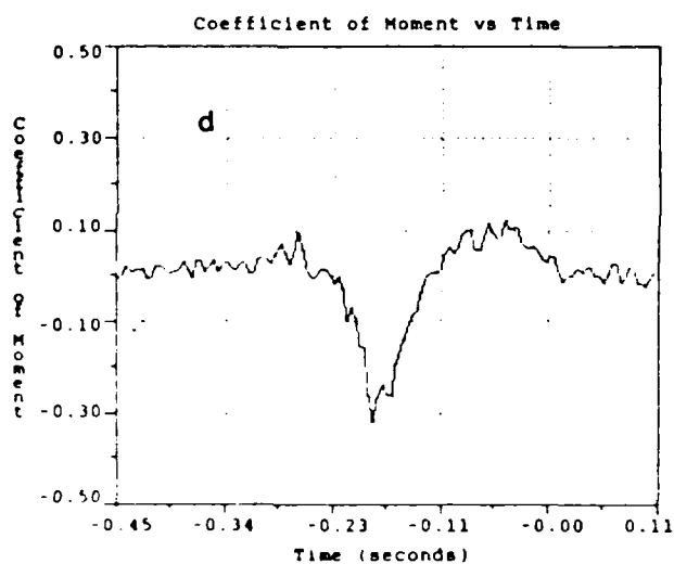
Figure 3b. Results from Run NN \dot{\alpha}_{ND\uparrow} = .0312, \dot{\alpha}_{ND\downarrow} = .0703 a) Angle of Attack Profile, b) Effect on C_L , c) Effect on C_D , d) Effect on C_M
