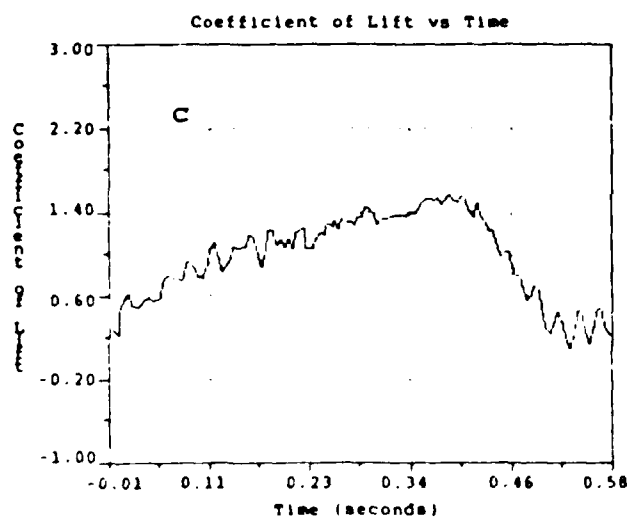
Figure 29. Results from Run GG \dot{\alpha}_{ND}^{up} = .0128 , \dot{\alpha}_{ND}^{down} = .0383
