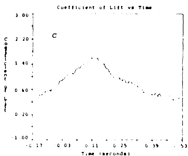
Figure 16. Results from Run F \alpha_{ND}^{up} = .0217 , \alpha_{ND}^{down} = .0269 a) Angle of Attack Profile, b) Effect on C_L c) Effect on C_D , d) Effect on C_M
