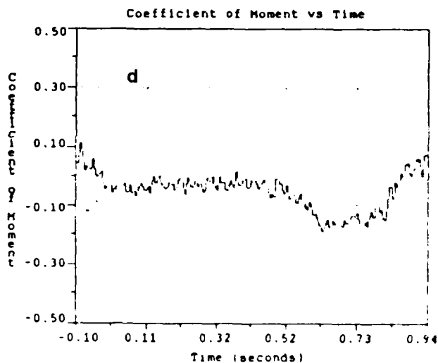
Figure 24. Results from Run BB \dot{\alpha}_{up} = .0110 , \dot{\alpha}_{ND, down} = .0652 a) Angle of Attack Profile, b) Effect on C_L c) Effect on C_D , d) Effect on C_M
