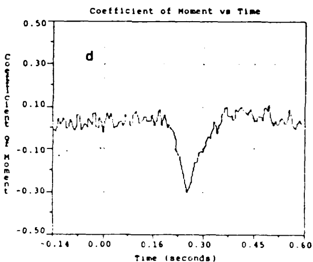
Figure 34. Results from Run LL \dot{\alpha}_{ND,up} = .0189 , \dot{\alpha}_{ND,down} = .0582 a) Angle of Attack Profile, b) Effect on C_L c) Effect on C_D , d) Effect on C_M
