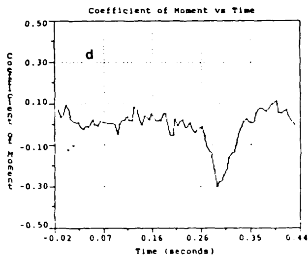
Figure 37. Results from Run 00 \dot{\alpha}_{ND_{up}} = .0322 , \dot{\alpha}_{ND_{down}} = .0798 a) Angle of Attack Profile, b) Effect on C_L c) Effect on C_D , d) Effect on C_M
