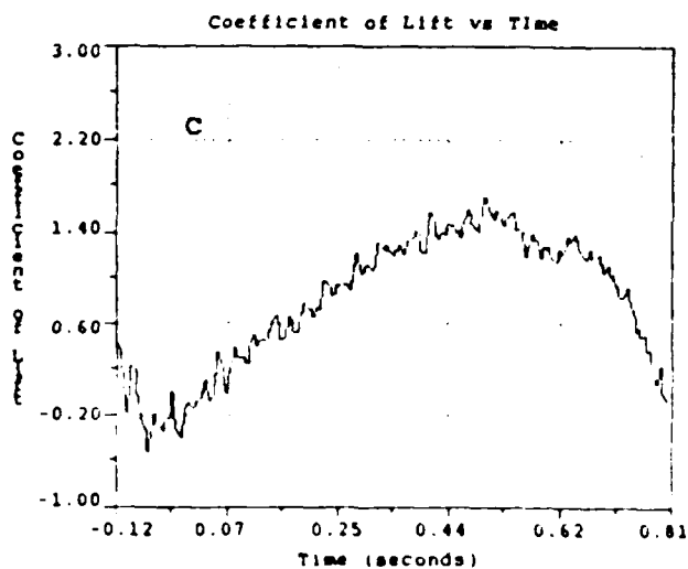
Figure 28. Results from Run FF \alpha_{ND}^{up} = .0138 , \alpha_{ND}^{down} = .0718 a) Angle of Attack Profile, b) Effect on C_D , c) Effect on C_L , d) Effect on C_M
