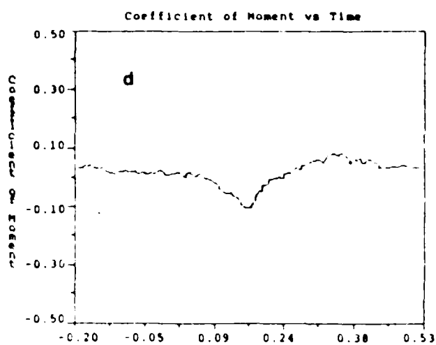
Figure 18. Results from Run H \dot{\alpha}_{ND,up} = .0251 , \dot{\alpha}_{ND,down} = .0230 a) Angle of Attack Profile, b) Effect on C_L c) Effect on C_D , d) Effect on C_M
