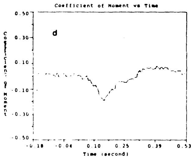
Figure 17. Results from Run G \dot{\alpha}_{NI} = .0241 , \dot{\alpha}_{ND} = .0276 a) Angle of Attack Profile, b) Effect on C_L c) Effect on C_D , d) Effect on C_M
