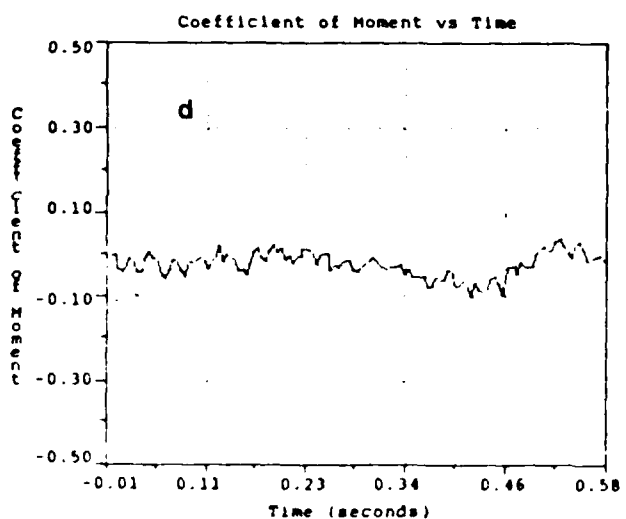
Figure 29. Results from Run GG \dot{\alpha}_{ND}^{up} = .0128 , \dot{\alpha}_{ND}^{down} = .0383
