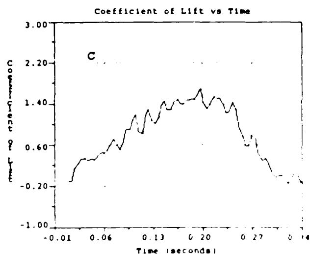
Figure 35. Results from Run MM \alpha = 0.0327 , \beta = 0.0015 a) Angle of Attack Profile, \beta = 0.0015 b) Effect on C_D , \beta = 0.0015 c) Effect on C_L , \beta = 0.0015 d) Effect on C_M , \beta = 0.0015
