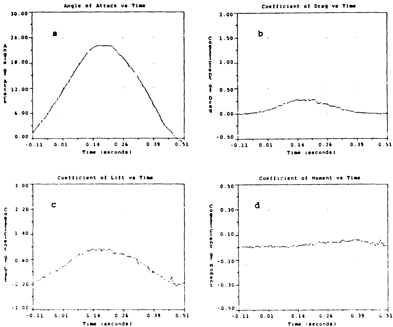
Figure 13. Results from Run C \dot{\alpha}_{ND}^{up} = .0264 , \dot{\alpha}_{ND}^{down} = .0279 a) Angle of Attack Profile, b) Effect on C_D , c) Effect on C_L , d) Effect on C_M
