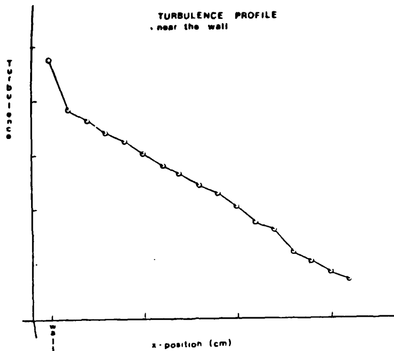
Figure 10. Turbulence Profile Near the Wall for the Modified L-2A
