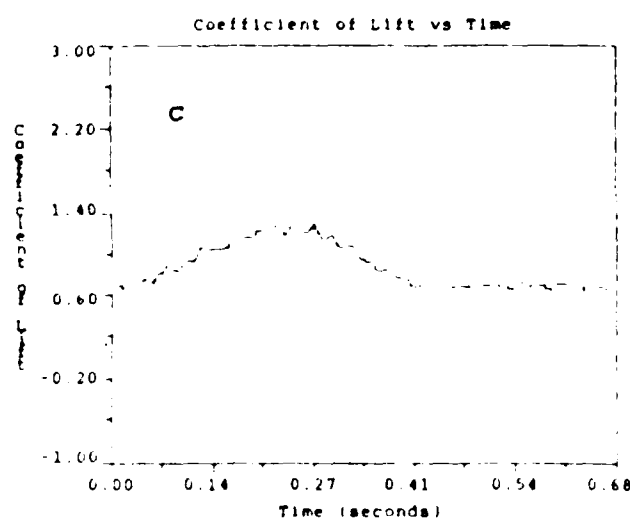
Figure 19. Results from Run 1 \dot{\alpha}_{D,up} = .0146 , \dot{\alpha}_{D,down} = .0206
