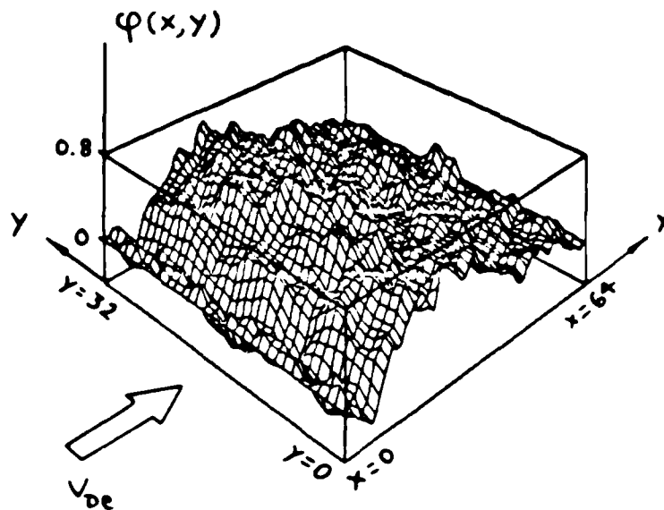
Fig.(3): Electrostatic potential at \omega_{pe}t=100 (time-averaged over 1.5 \omega_{pe}^{-1} ) from an ES2 simulation, with drifting electrons and constant injection at the walls. Parameters v_{de}=1.0 , v_{di}=1.0 , v_{di}=-0.01 , \omega_{pe}=1.0 , m_i/m_e=100 , \omega_{pi}=0.1 , L_x=2L_y=64 , and no magnetic field.
