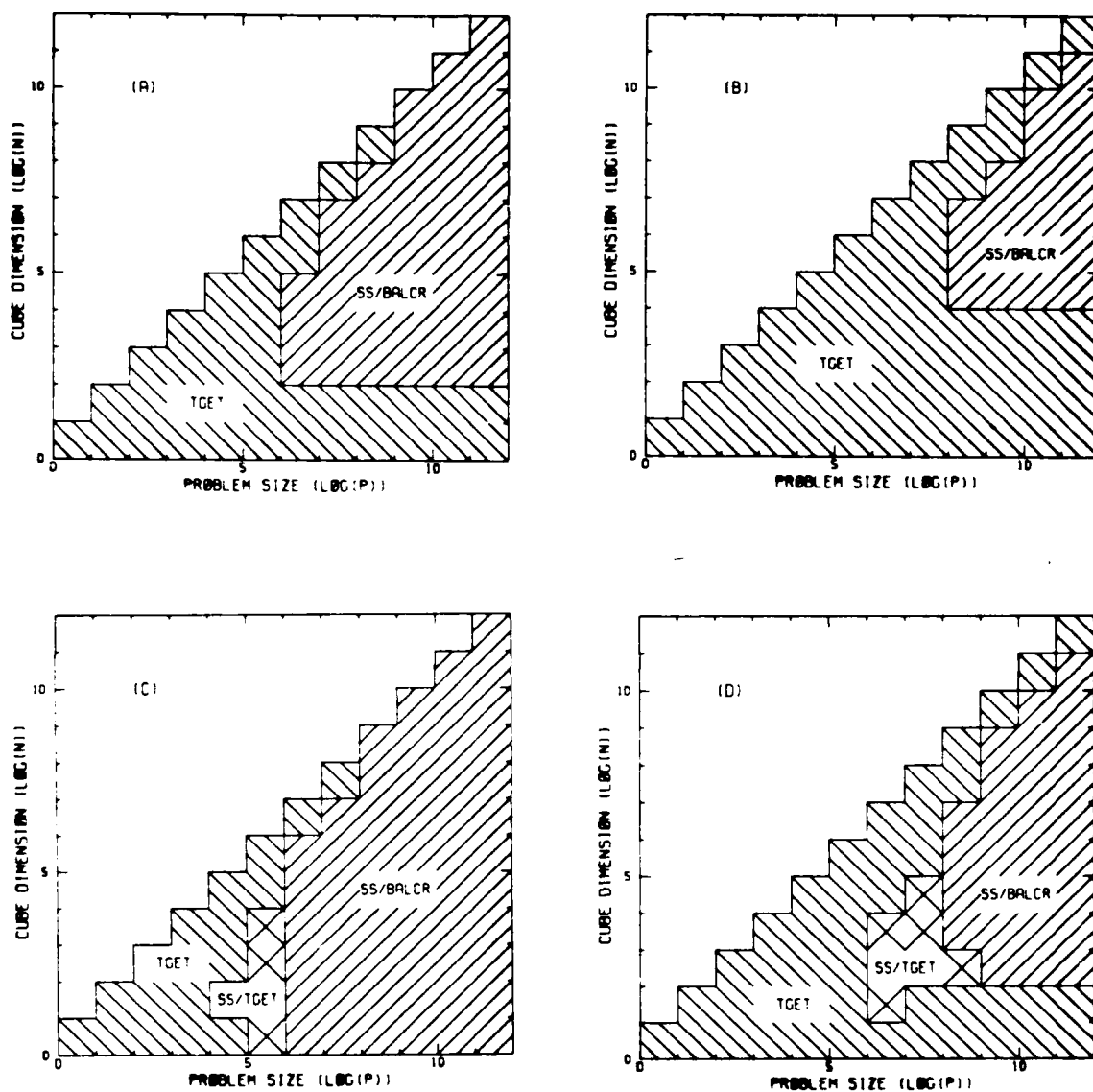
Figure 2: Comparison of TGET, SS/TGET and SS/BalCR based on model times for solving P tridiagonal systems of order P , on N processors. N \leq P , \tau = 1000 and t_c = 1 . (A): t_a = 25, t_{copy} = 10 , (B): t_a = 25, t_{copy} = 5 , (C): t_a = 5, t_{copy} = 5 , (D): t_a = 5, t_{copy} = 1 .
