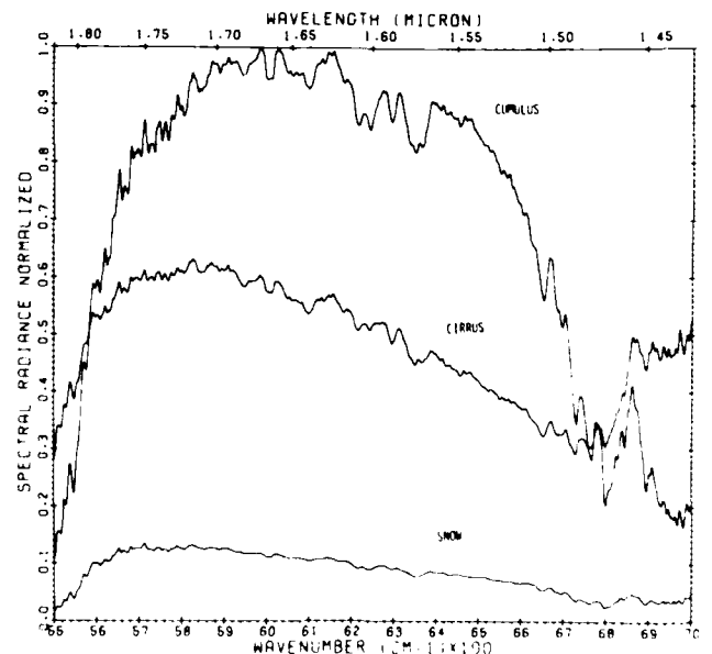
Figure 2. Average Spectral Radiance for 36 Cases of Cumulus, 32 Cases of Cirrus, and 56 Cases of Snow Obtained from Valovcin (1978). The plots are normalized such that the maximum radiance has a value of 1.0.
