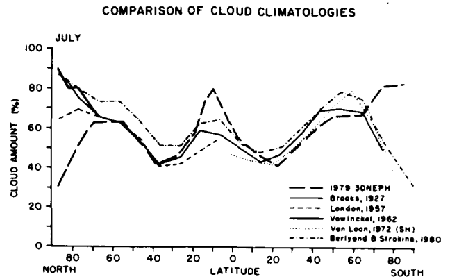
Figure 1. Comparison of Average Cloud Amount (%) of total cloud cover from various sources for the month of July with the July 1979 3DNEPH Archive. For this comparison, all data sources are averaged over latitudinal bands. Data were obtained from Hughes (1984) and Henderson-Sellers (1986).
