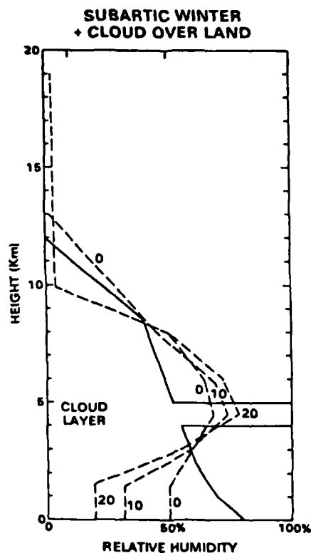
Figure 8. Simulated Retrieval of Relative Humidity in the Presence of a Cloud. The solid curve is the actual relative humidity profile and the dashed curves are the retrieved profiles for cloud water contents of 0, 10, and 20 mg/cm 2 throughout the 1-km depth of the cloud.
