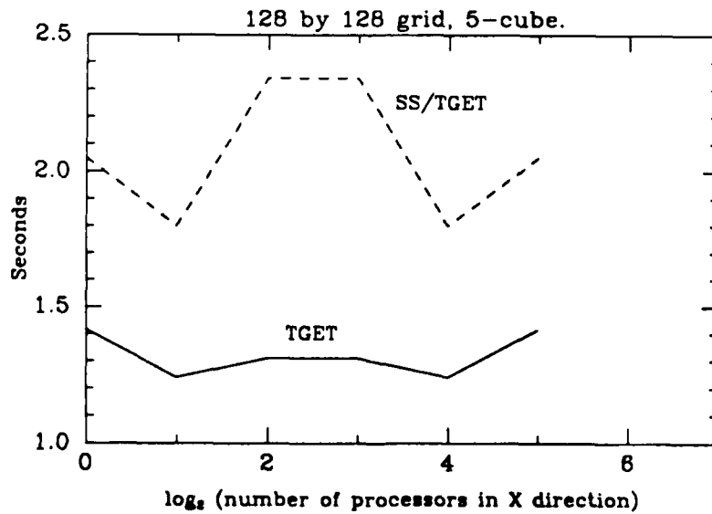
Figure 5: Effect of varying the aspect ratio of the processor mesh for a 5-cube. Time for one ADM step vs. N_x . Solid line: Using TGET, Dashed line: Using SS/TGET
