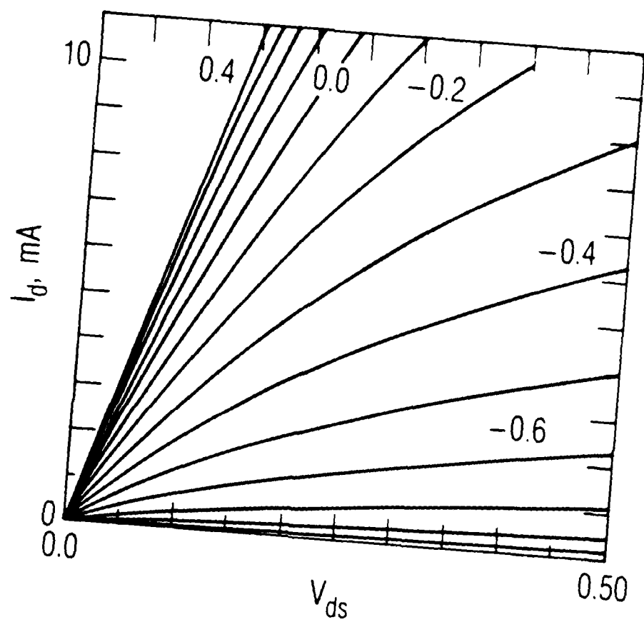
Fig. 1. I/V characteristic of an Avantek AT10650-5 GaAs MESFET in its linear region
