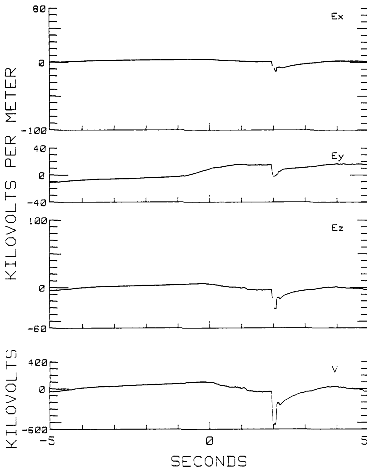
Fig. 62 — Cartesian vector field and aircraft potential
