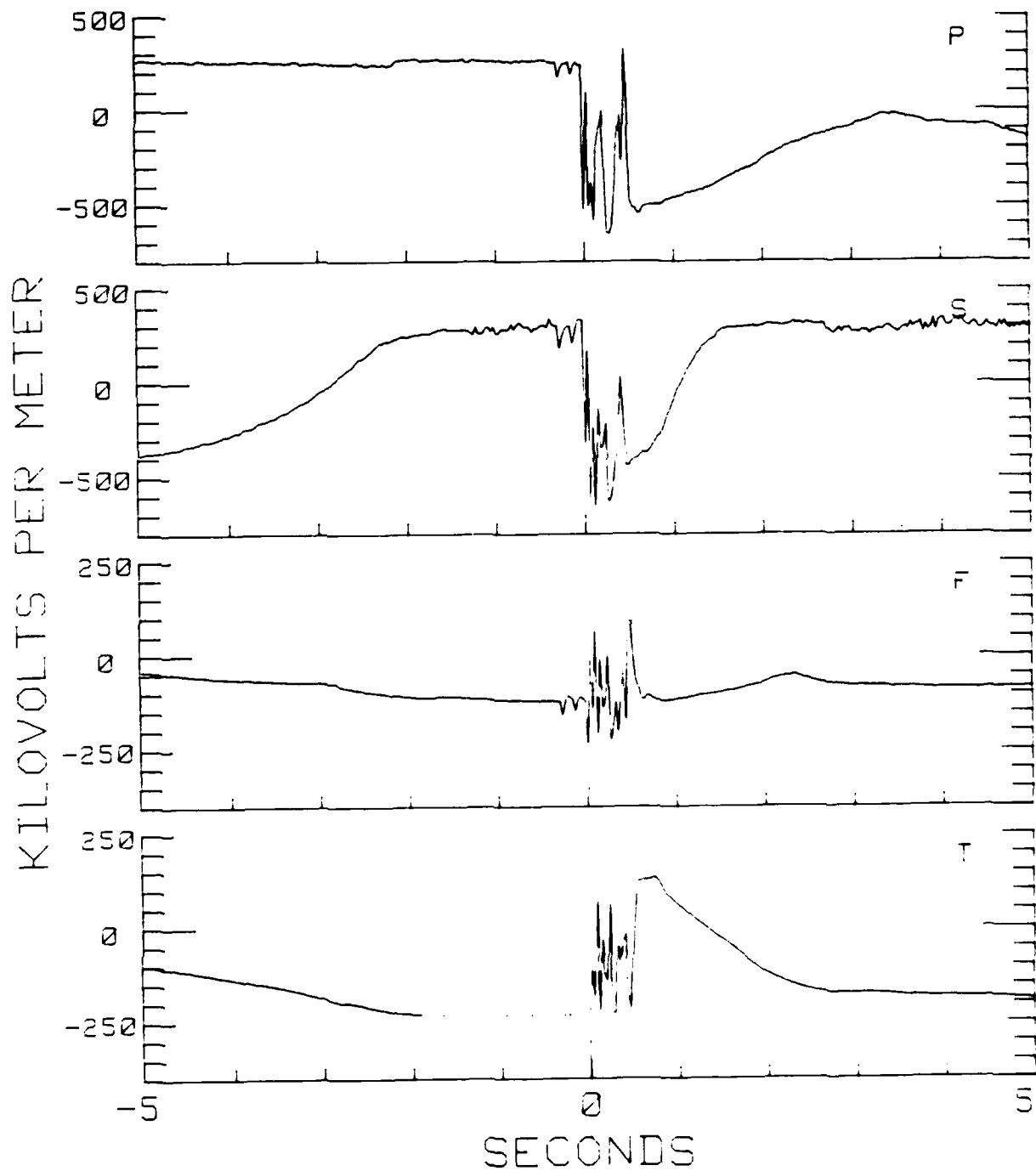
Fig. 19 — Field values at Port, Starboard, Forward, and Tail meters
