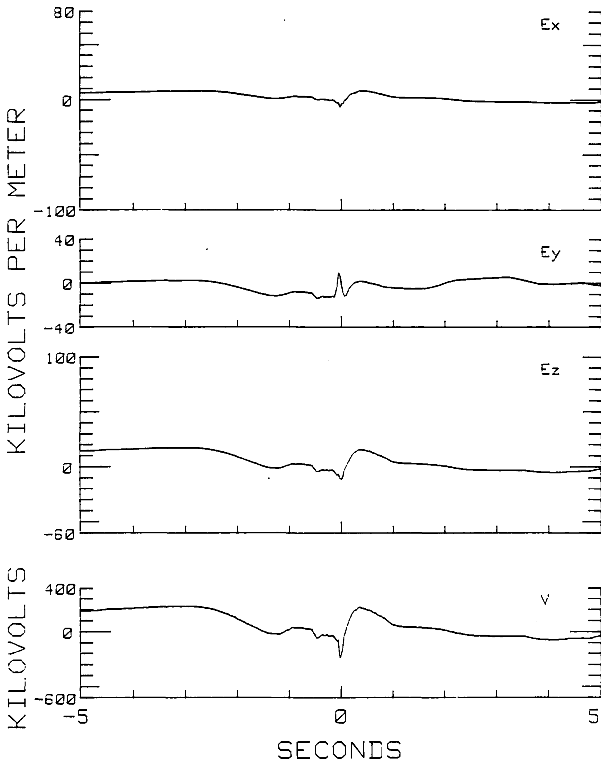
Fig. 65 — Cartesian vector field and aircraft potential
