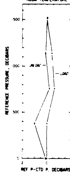
PRECRUISE PRESSURE SENSOR HYSTERESIS CTD no 2 12 MAR 84 ROOM TEMPERATURE
