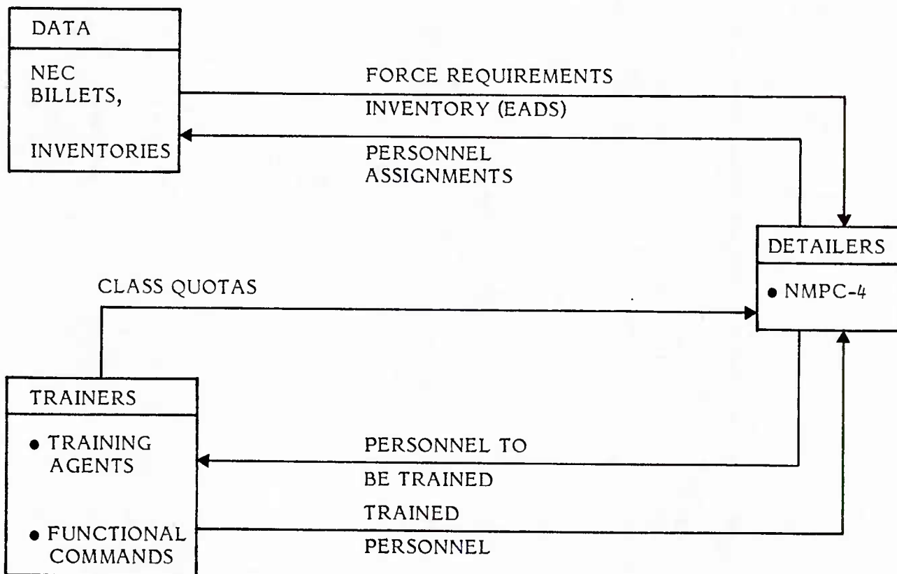
Figure 9. Plan execution.
