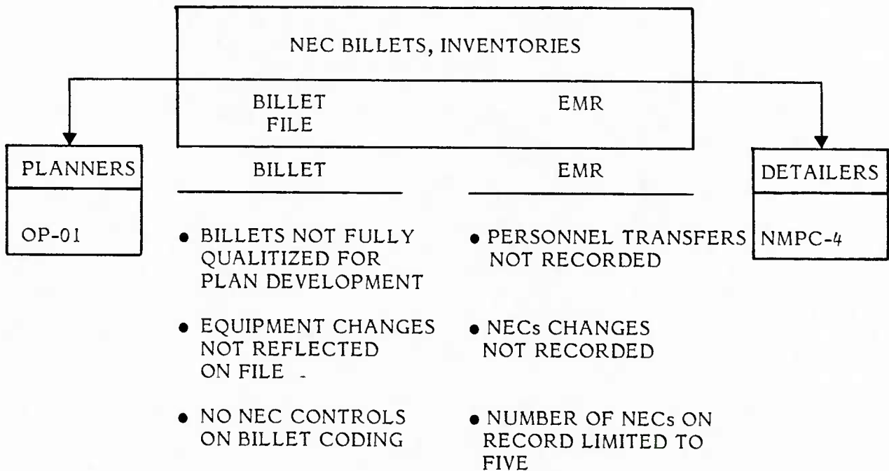
Figure 11. Data problems.
