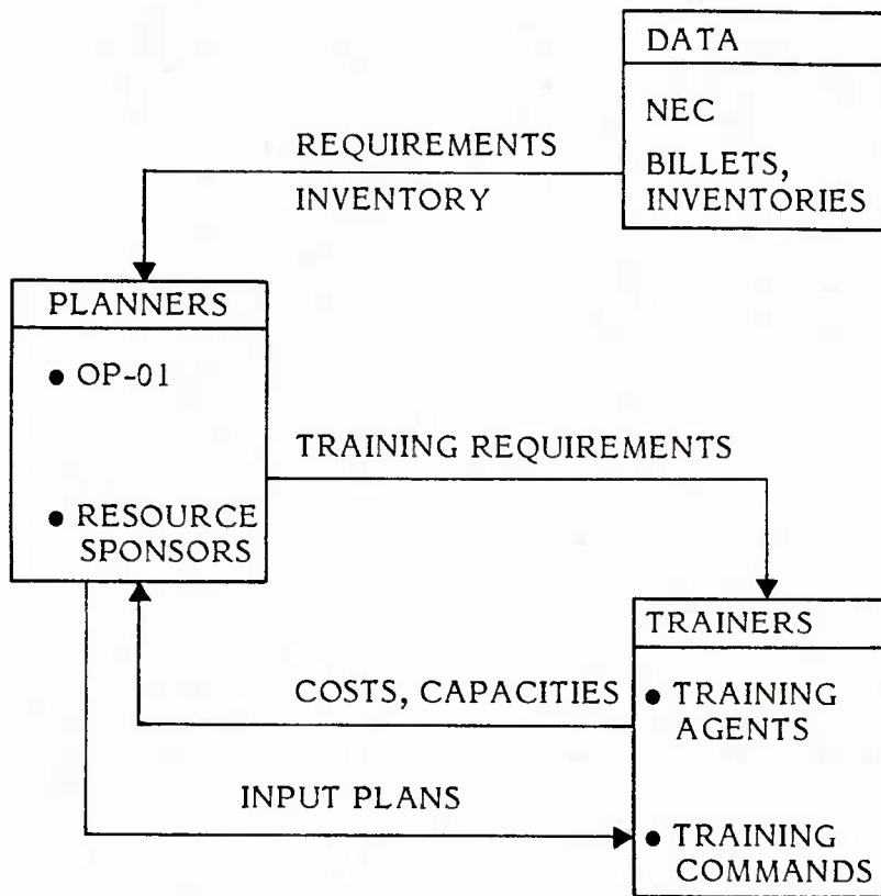
Figure 5. Planning.
