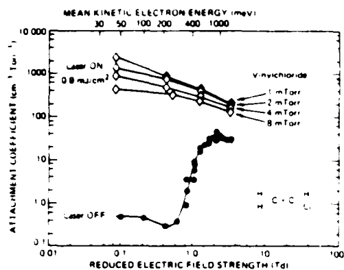
FIG. 2. Attachment coefficient for vinylchloride in helium buffer (500 Torr). The solid points represent the data for unexcited mixtures, obtained at vinylchloride pressures ranging from 50 to 500 mTorr. The photoenhanced attachment coefficient (open points) is expressed in terms of the unexcited vinylchloride concentration.
