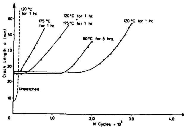
FIG.9.35 CRACK GROWTH CURVES FOR SPECIMENS SUBJECTED TO DIFFERING HEAT-TREATMENT DURING PATCH APPLICATION
