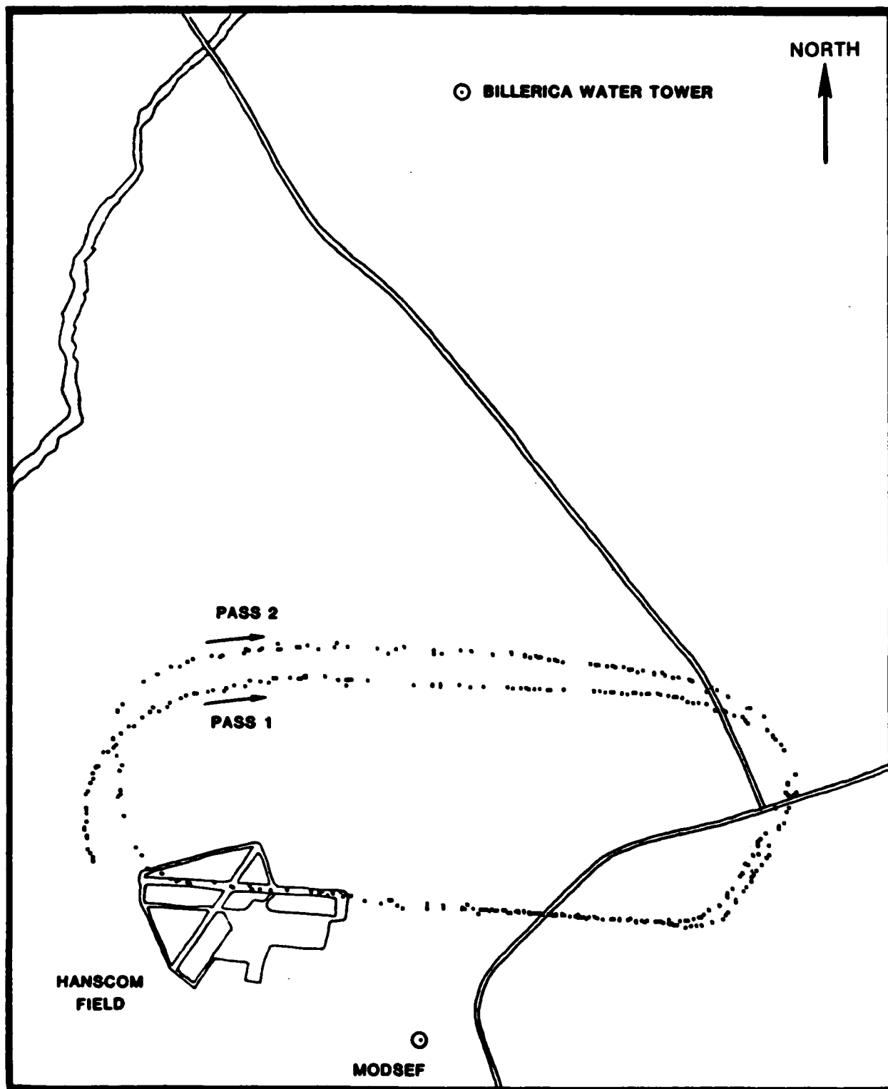
Fig. 4-2. Flight path.
