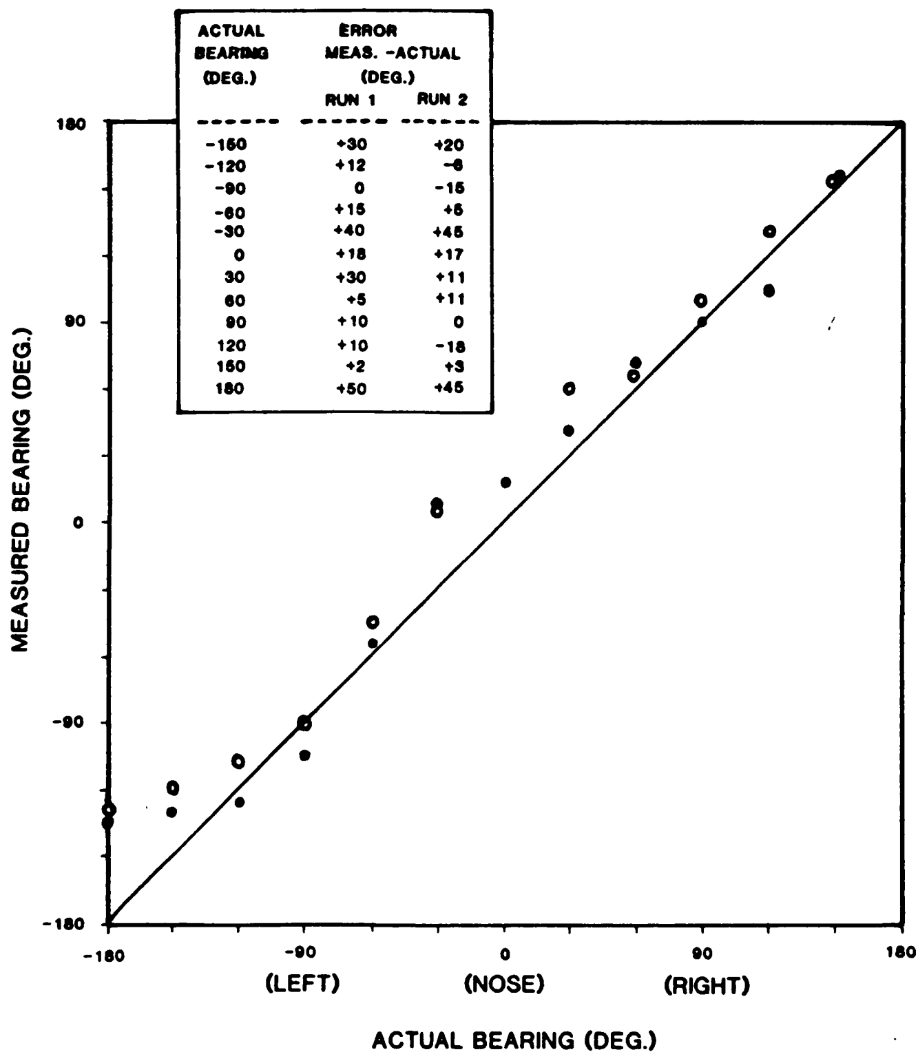
Fig. 4-1. Bearing calibration check, on the ground.
