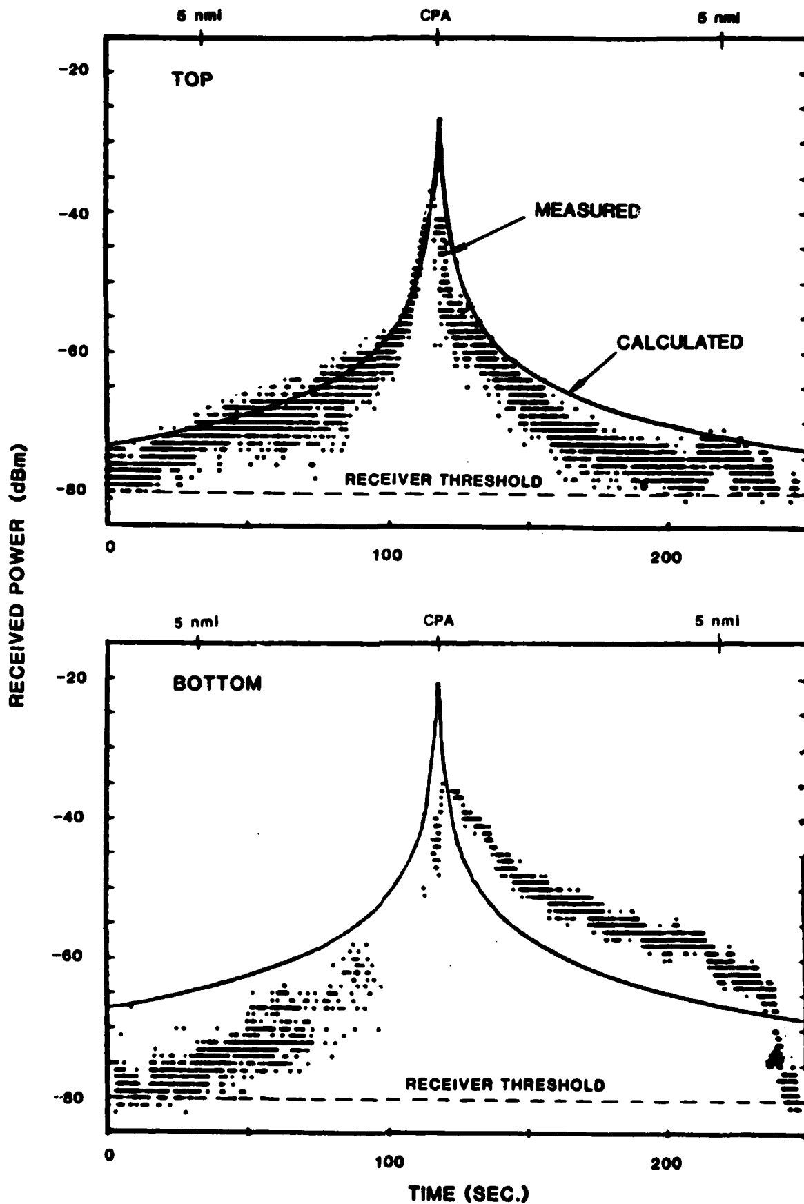
Fig. 3-4. Received power, encounter no. 1.
