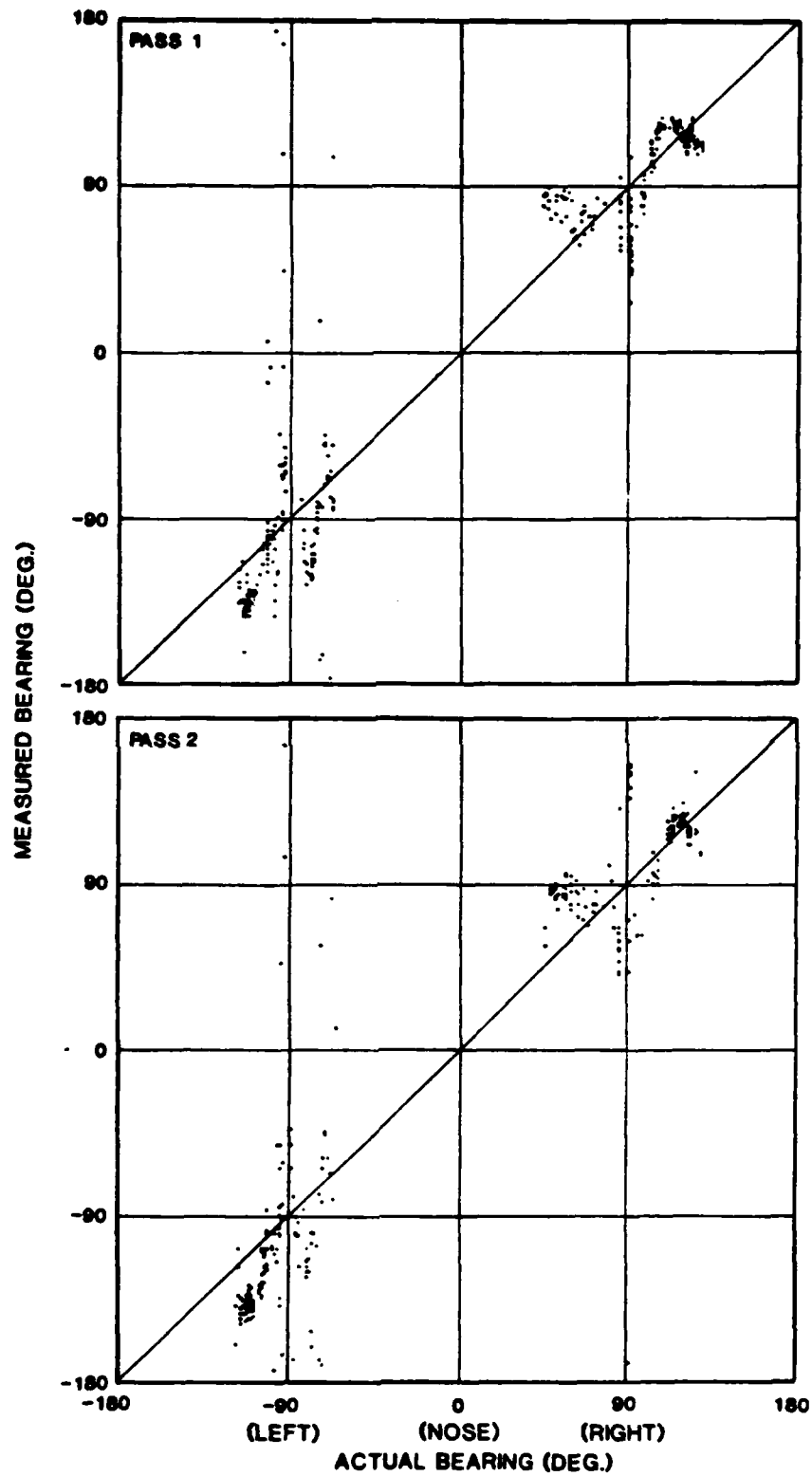
Fig. 4-3. AOA transfer function, two westbound passes.
