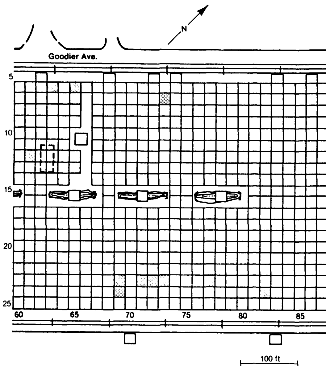
Figure 20. Original Expansion Area--TCDD Concentrations in Compositd Surface Soils, >50 ppb through 100 ppb.
