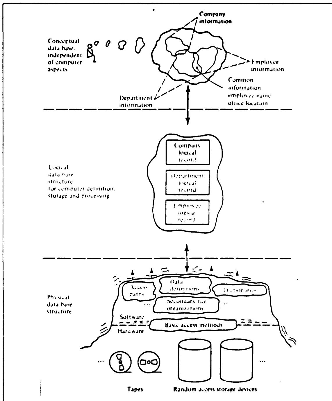
Figure 2.2 Realms of a data base management system.
