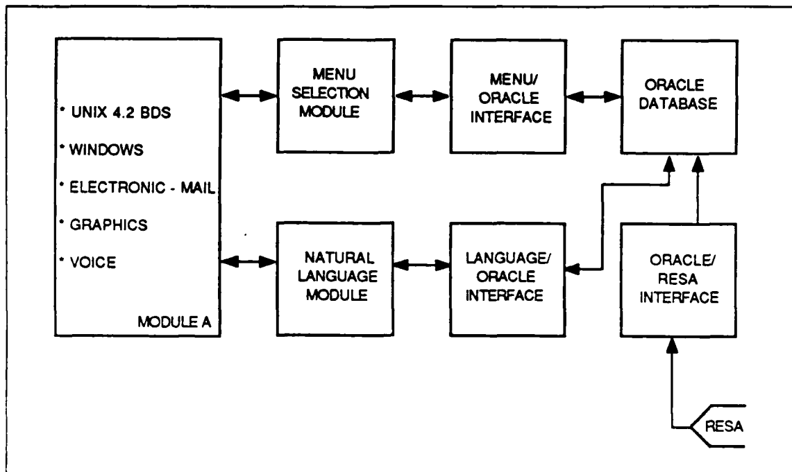
Figure 1.1 Concept of a C2 workstation as a DSS.
