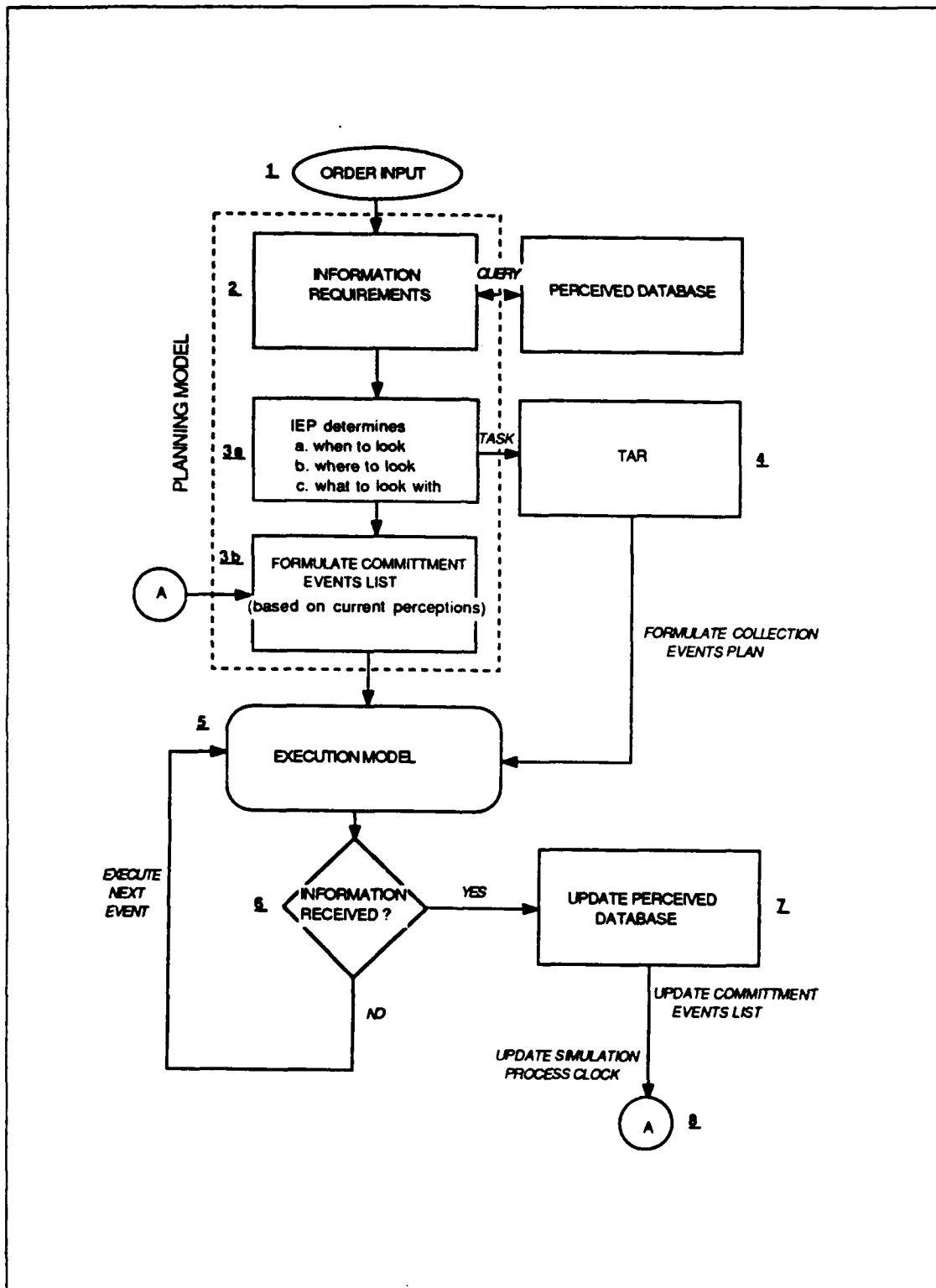
Figure 5.3 Process Flow.
