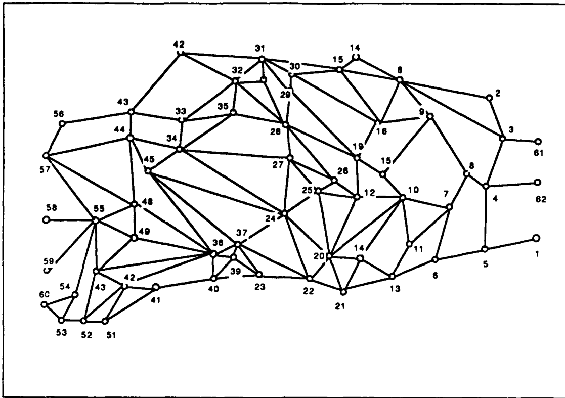
Figure 4.6 Simple Network.
