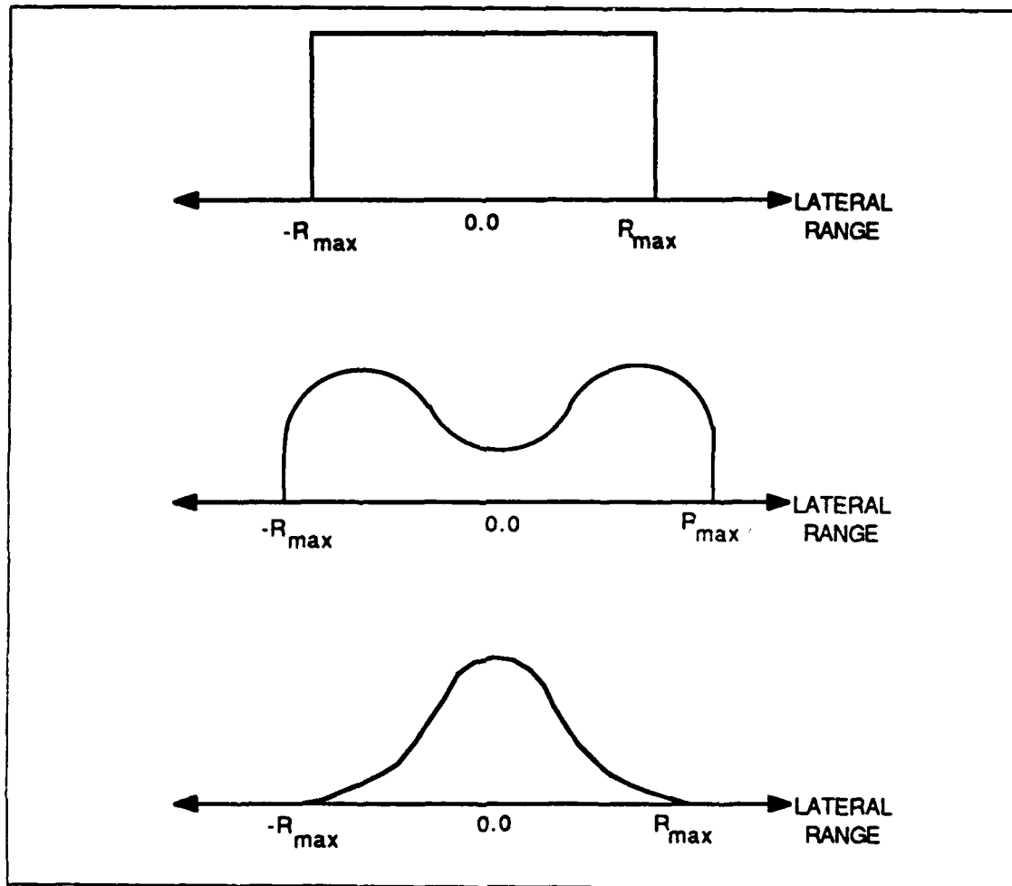
Figure 4.14 Typical Lateral Range Curves.
