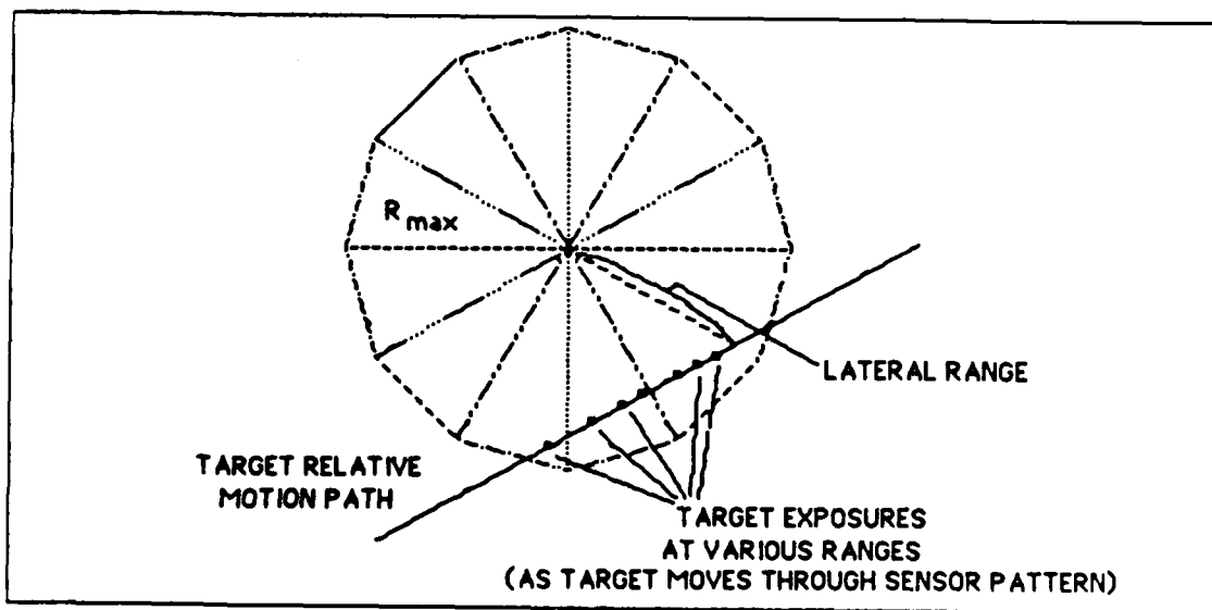
Figure 4.13 PBAR for an Arbitrary Sensor.
