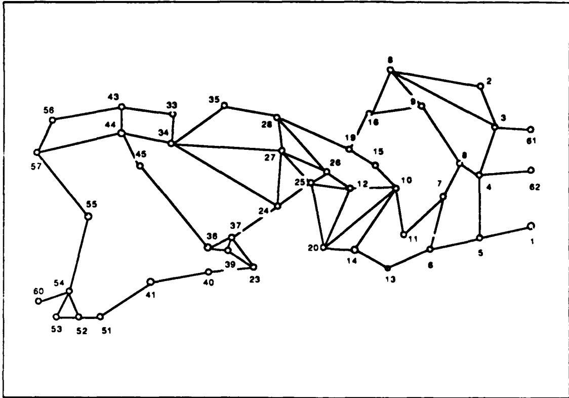
Figure 4.7 Connected Network.
