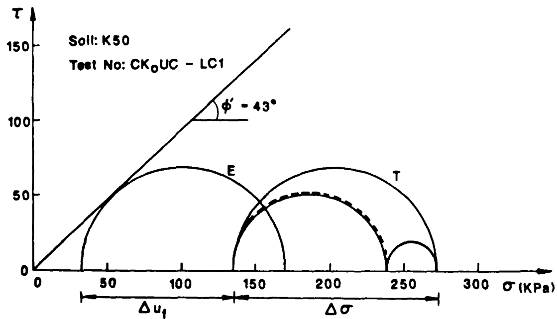
Figure 3.10 Mohr Circles for CK 0 UC-AC and CK 0 UC-LC for K50
