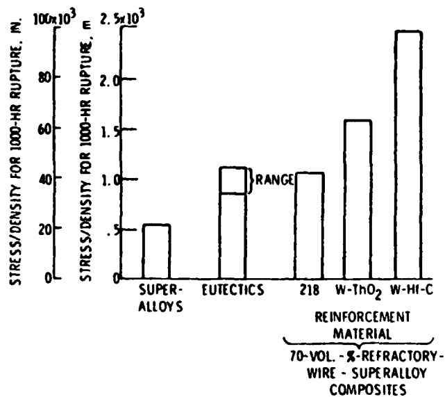
Figure 2: 1000 hours stress rupture properties of refractory wire superalloy composites at 1090 C (12).
