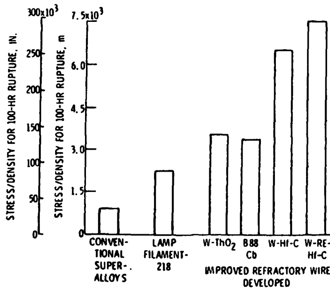
Figure 4: 100 hours stress rupture properties of refractory alloy fibres at 1090 C (12).
