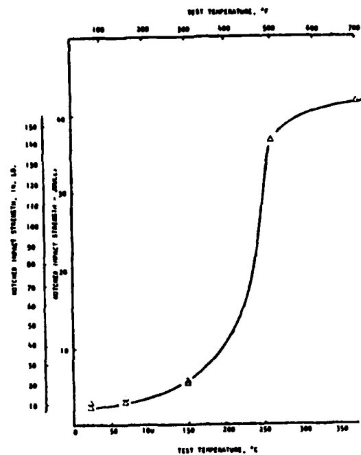
Figure 8: Notched impact strength versus temperature for W/FeCrAlY (58).
