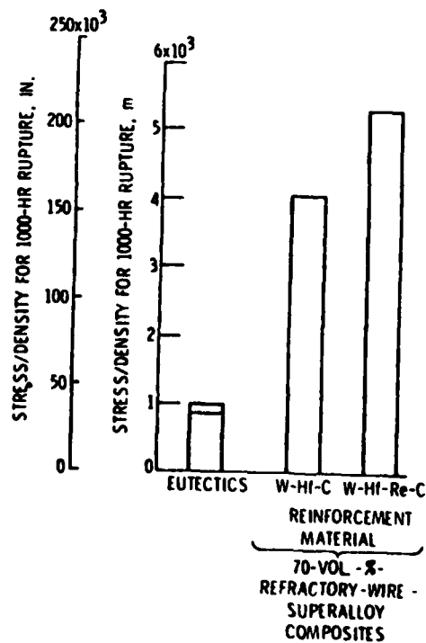
Figure 3: Projected 1000 hours composite rupture properties with diffusion barrier at 1090 C (12).
