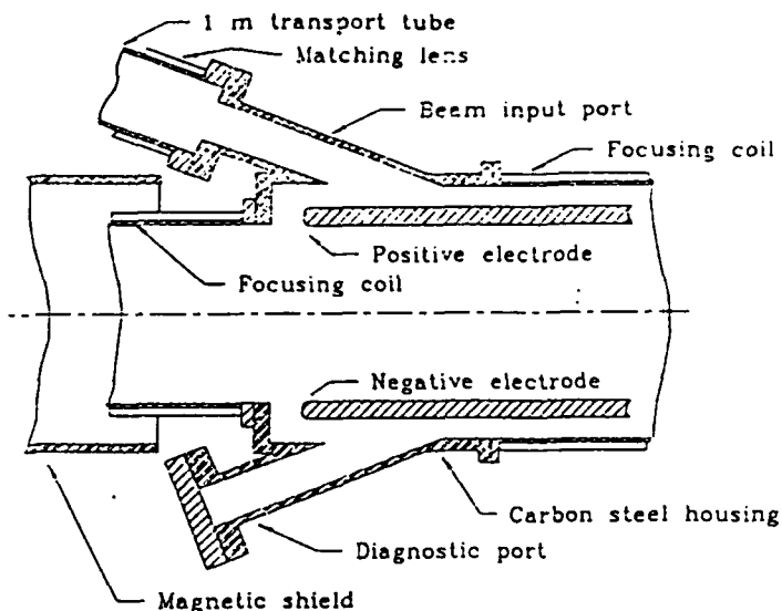
Fig. 3. Inflector assembly
