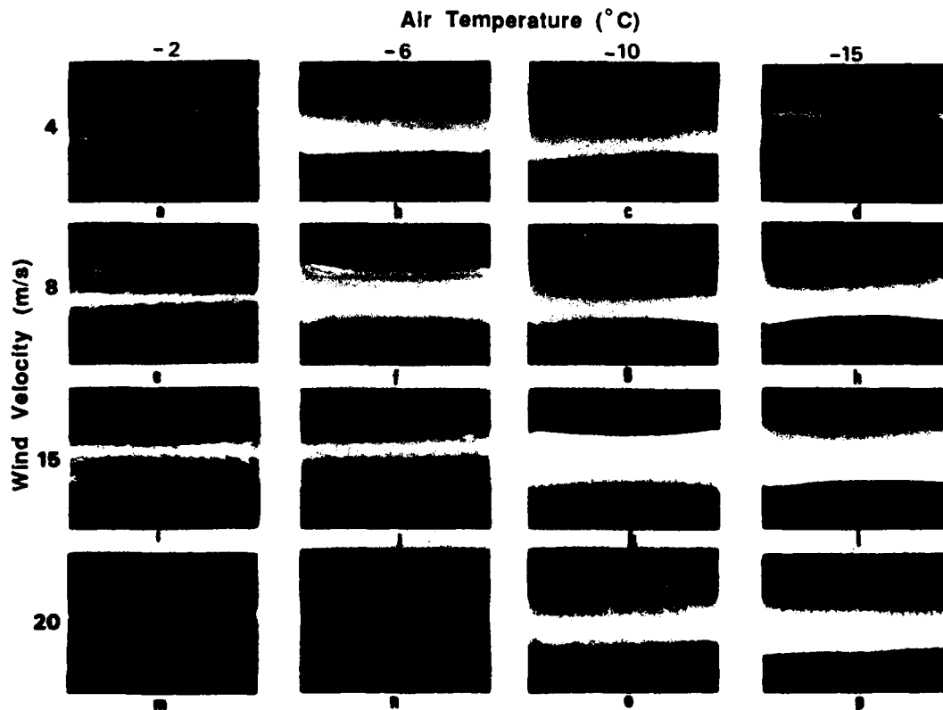
Figure 3. Ice accretions grown under different ambient temperatures and air velocities. (From Laforte et al. 1983.)
