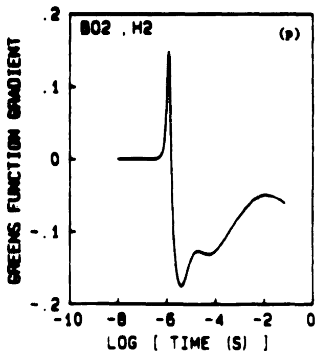
Figure 3.15. (Continued) Sensitivity of B_{O_2} Concentration Versus Time to Variations in the Concentration of Several Reactants in an Isothermal, Constant Volume Mixture of H_2O , H_2 , CO_2 , O_2 and N_2
