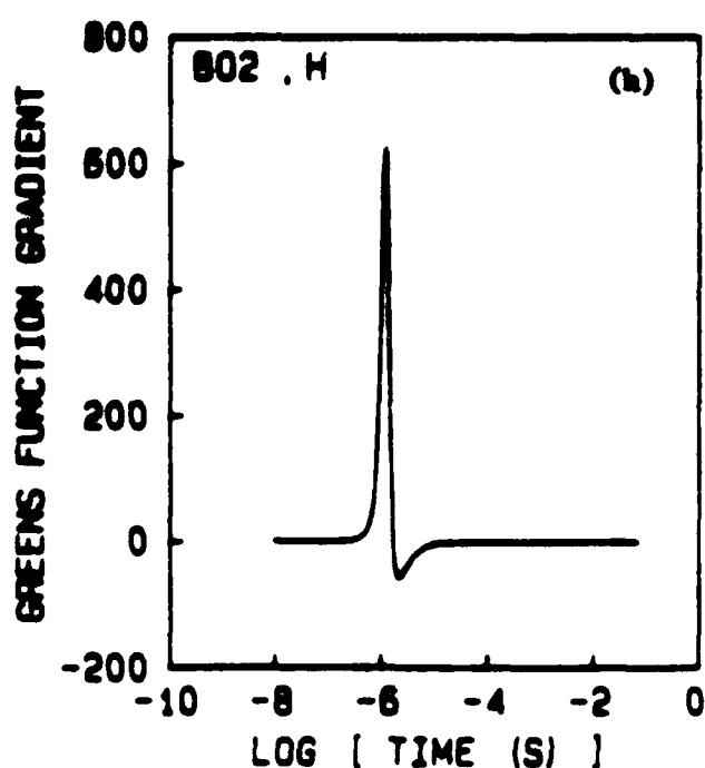
Figure 3.15. (Continued) Sensitivity of \text{SO}_2 Concentration Versus Time to Variations in the Concentration of Several Reactants in an Isothermal, Constant Volume Mixture of \text{H}_2\text{O} , \text{H}_2 , \text{CO}_2 , \text{O}_2 and \text{H}_2
