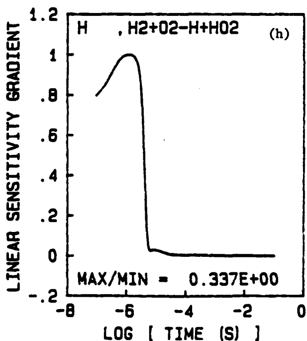
Figure 3.23. (Continued) Sensitivity of H Concentration Versus Time to Variations in Kinetic Rate Constants for an Oxygen Deficient Mixture of HB0 and Hydrocarbon Combustion Products
