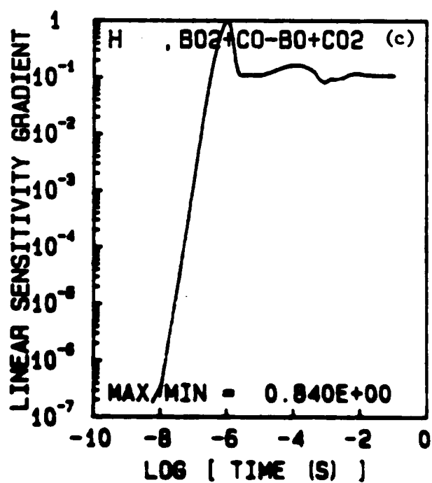
Figure 3.21. Sensitivity of H Concentration versus Time for Kinetic Rate Constants for an Equimolar Mixture of H_2O , Hydrocarbon, and Oxygen
