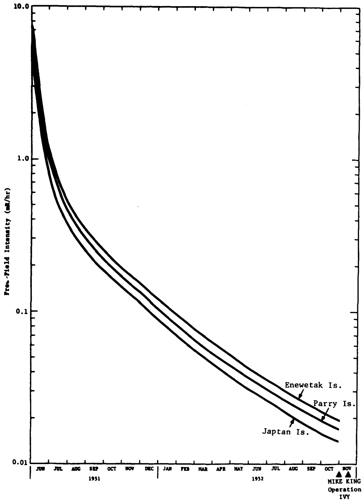
Figure 2. Post-GREENHOUSE radiation environments on the residence islands of Enewetak Atoll.
