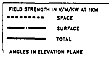
Figure A.35 Radiation Pattern - 90 Deg. Monopole over Perfect Ground.
