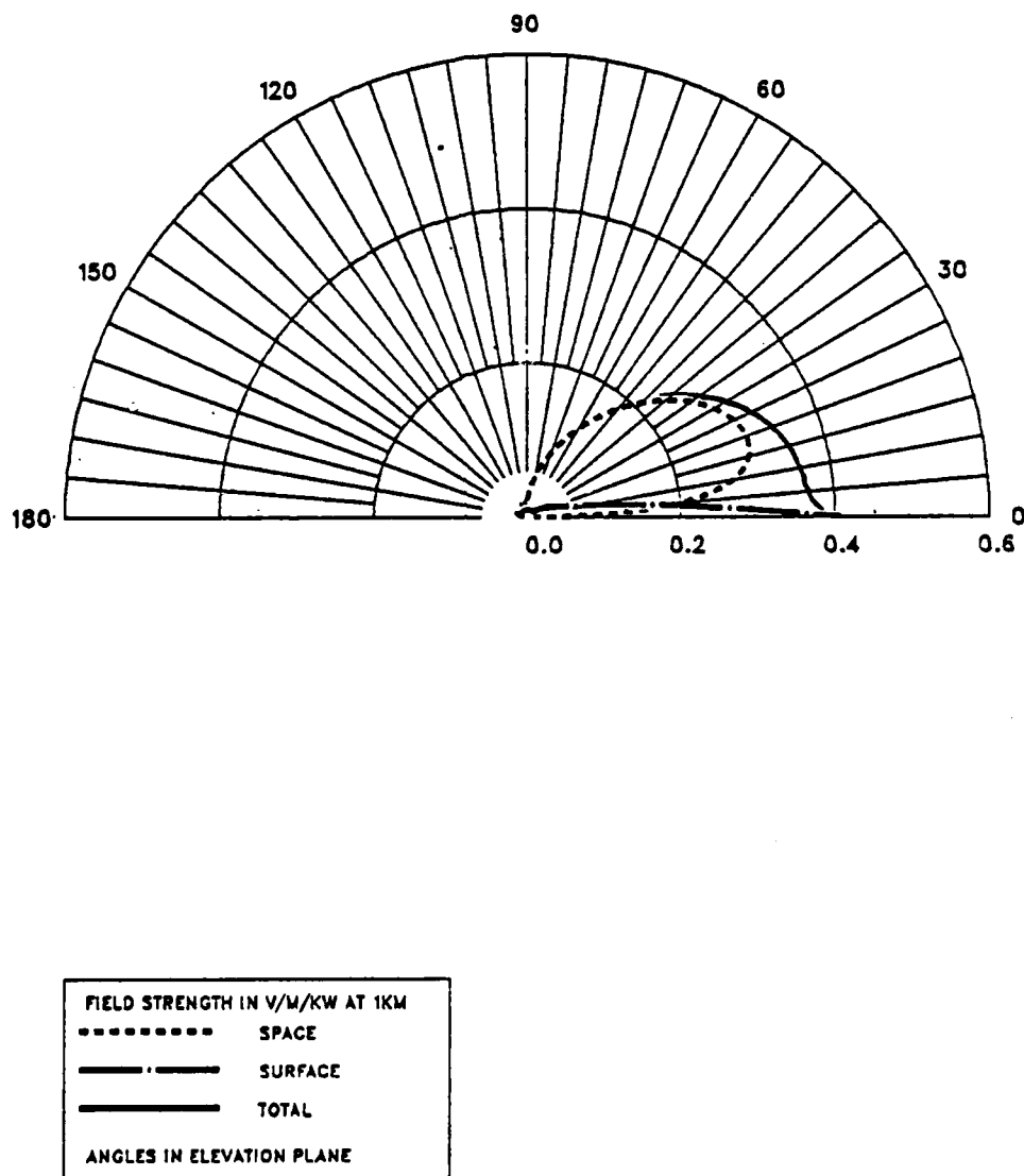
Figure A.56 Radiation Pattern - 90 Deg. Coupled Monopoles 5 Deg. over Finite Ground.
