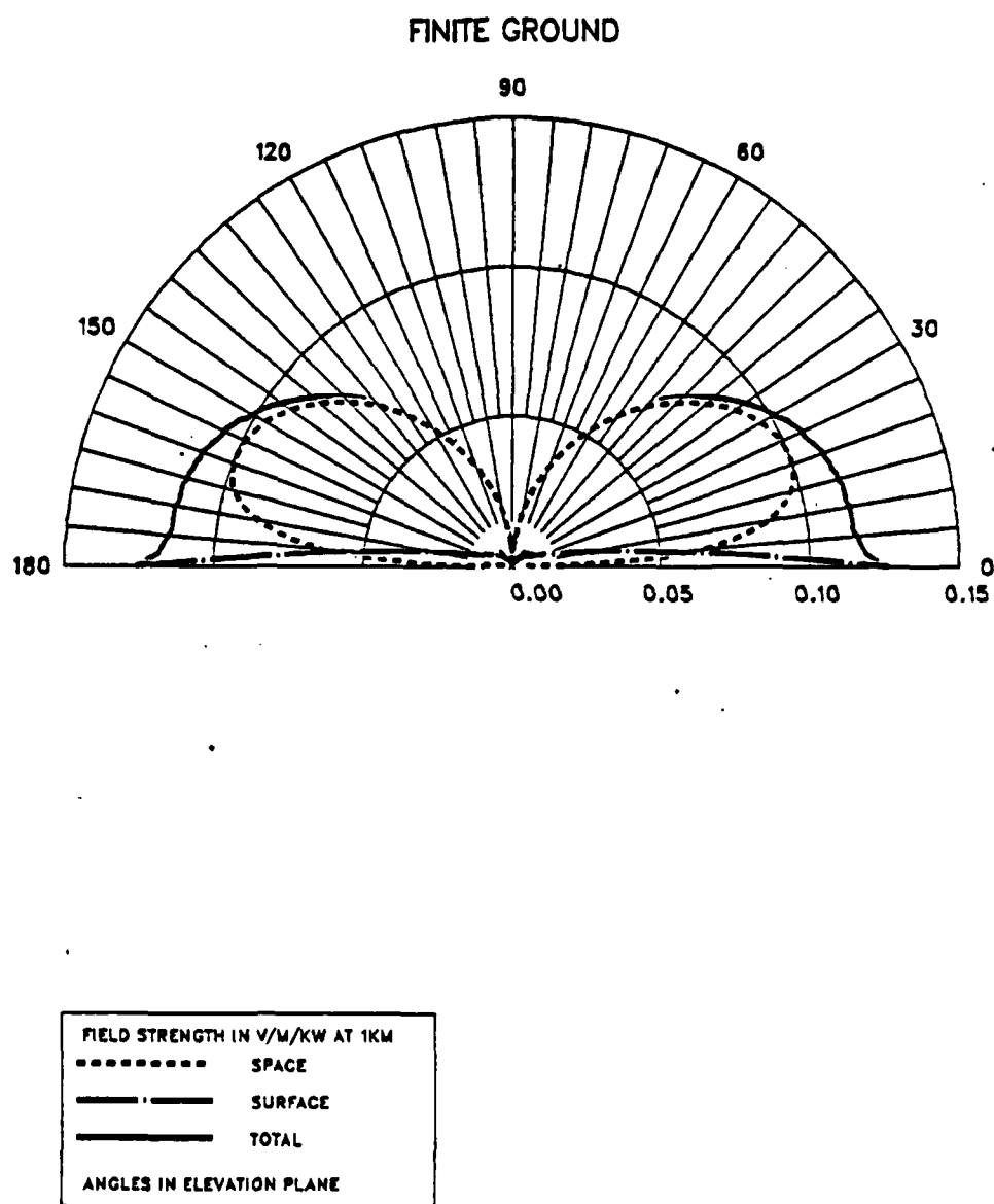
Figure A.36 Radiation Pattern - 90 Deg. Monopole over Finite Ground.
