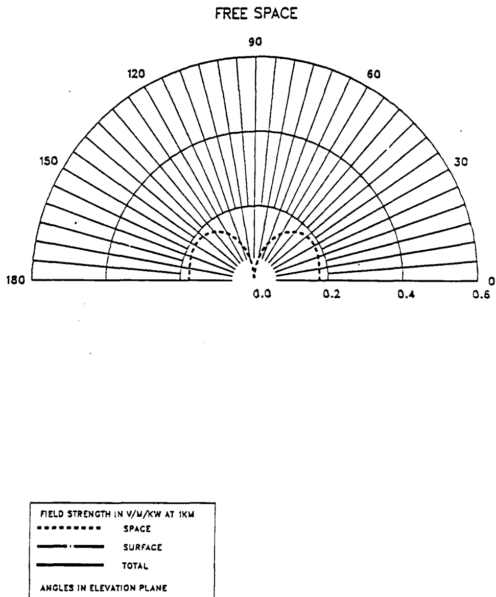
Figure A.41 Radiation Pattern - 10 Deg. Monopole in Free Space.
