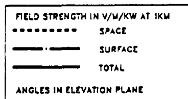
Figure A.27 Radiation Pattern - 20 Deg. Coupled Dipoles 0.5 Deg. over Finite Ground.
