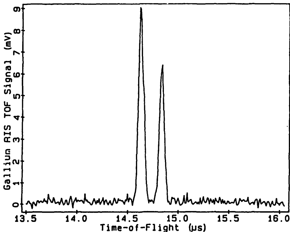
Figure 26. Gallium signal seen after only 500 laser shots from a sample containing 0.48 ppm Ga in Si. The sensitivity derived from this data is 15 ppb. Simple operational changes could increase the sensitivity to at least 0.1 ppb.
