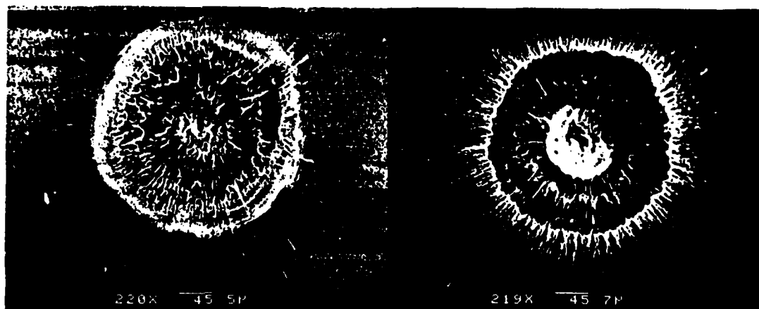
Figure 11. Scanning electron micrographs of craters produced in silicon after a single laser shot at 2 \times 10^{11} \text{ W cm}^{-2} (left) and after ten laser shots at the same power density (right). Profiles of these same craters were shown in Figure 9.
