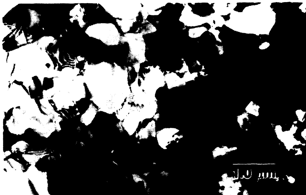
Figure 4.6. TEM micrographs of the grip section of a simulated warm temperature tested sample, deformed at 300°C and 1.67 \times 10^{-3} \text{ s}^{-1} strain rate.
